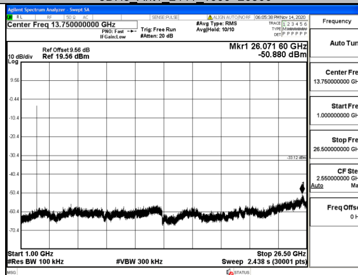
3DH5_Ant1_2480_0~Reference
