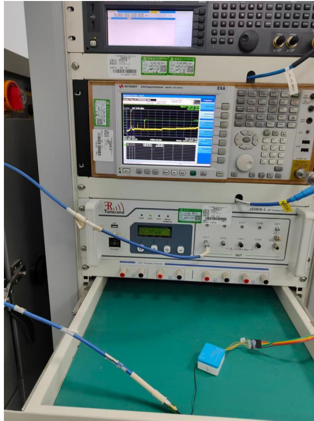
Conducted Emission Test View
