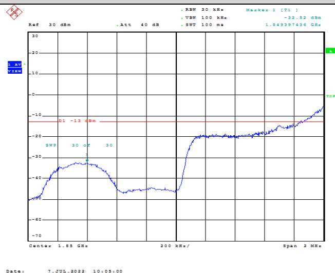
Band2-1.4MHz-QPSK-18607-1RB#5
