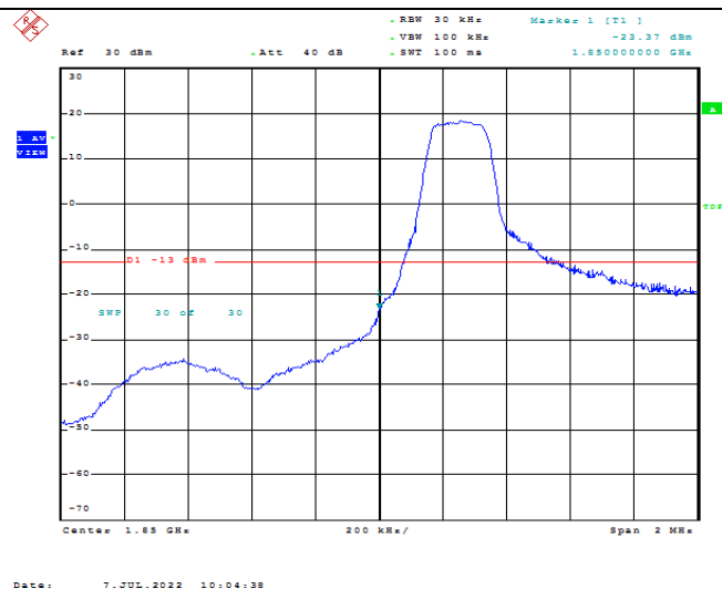
Band2-1.4MHz-QPSK-18607-1RB#0
