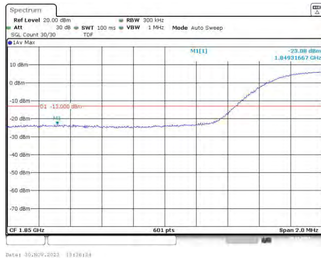
Band25-15MHz-16QAM-26615-75RB#0
