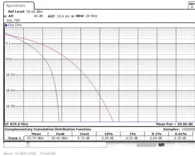
Band26-10MHz-QPSK-26915-50RB#0
