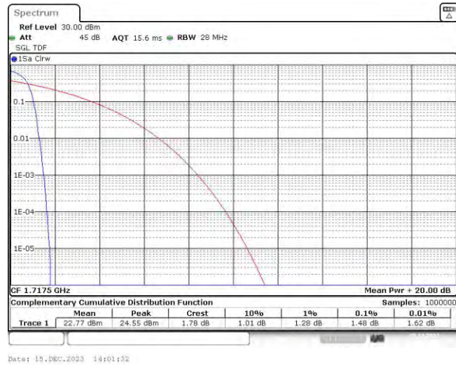
Band66-15MHz-QPSK-132322-75RB#0
