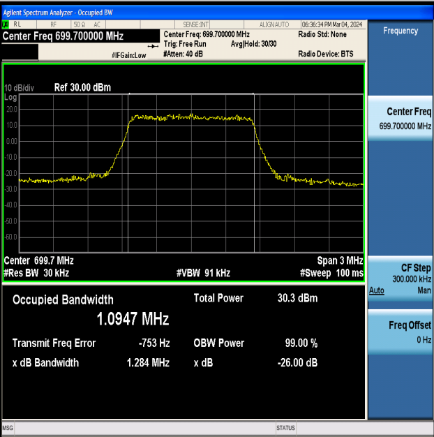
Band12-1.4MHz-16QAM-23017-6RB#0-PASS
