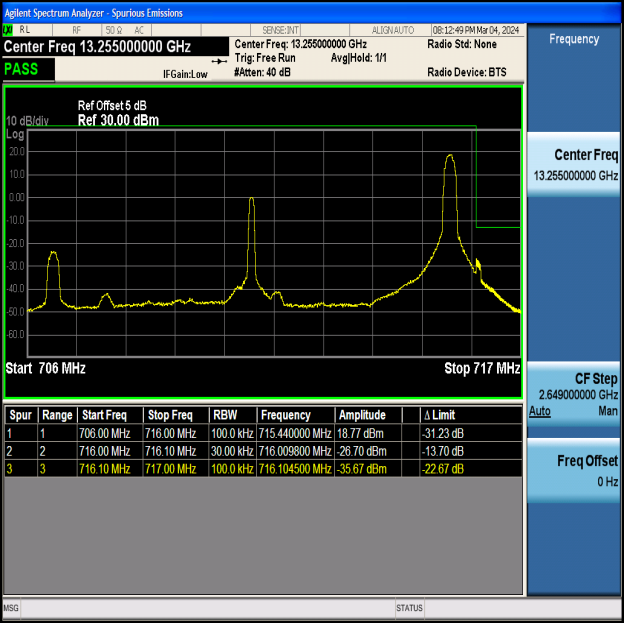
Band12_10MHz_16QAM_23130_1RB#49
