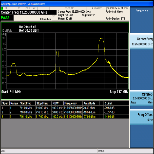
Band12_5MHz_QPSK_23155_1RB#24
