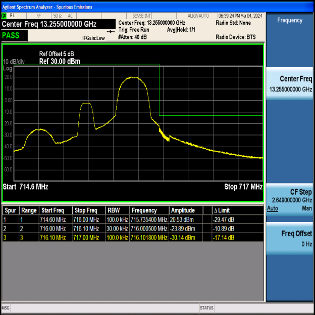
Band12_1.4MHz_QPSK_23173_1RB#5
