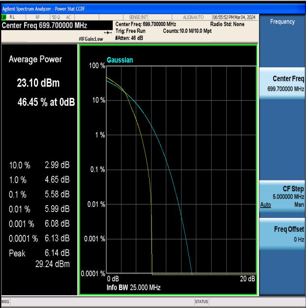
Band12-1.4MHz-16QAM-23017-1RB#0-PASS
