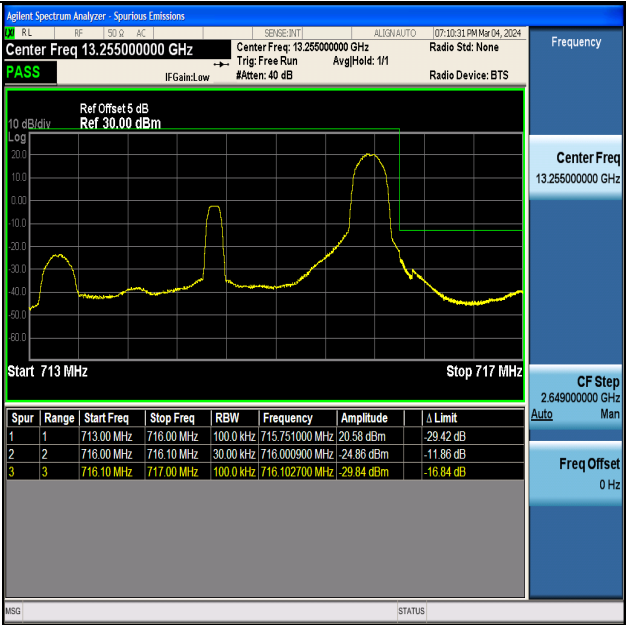
Band12_3MHz_QPSK_23165_1RB#14
