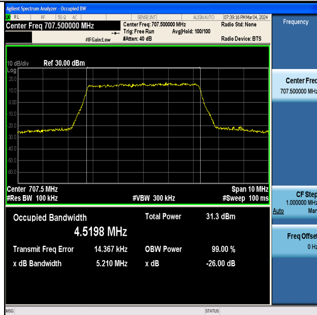
Band12-5MHz-16QAM-23095-25RB#0-PASS
