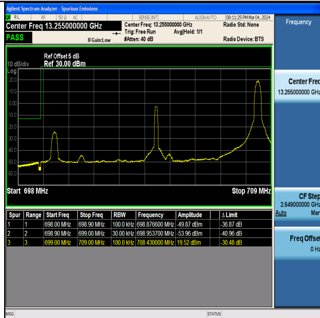
Band12_10MHz_16QAM_23060_1RB#49
