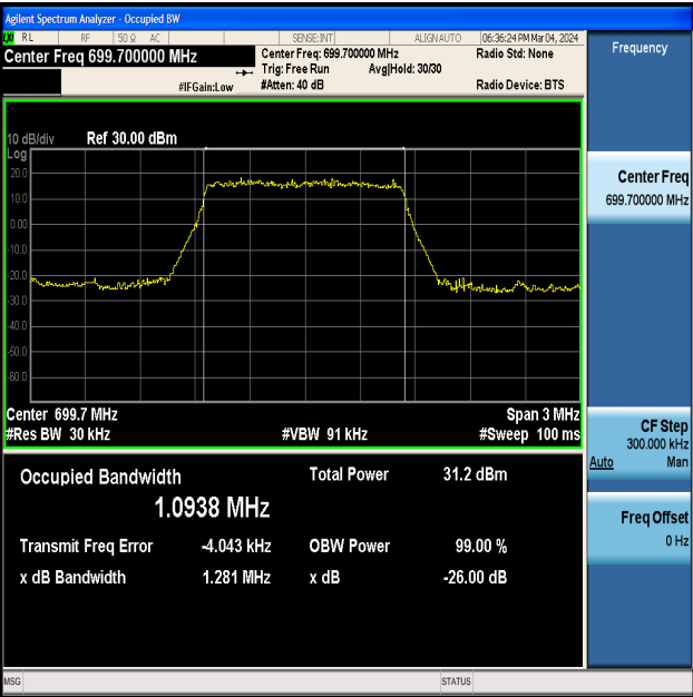
Band12-1.4MHz-QPSK-23017-6RB#0-PASS
