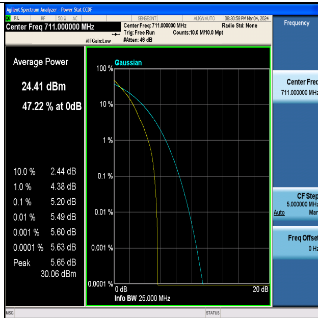
Band12-10MHz-QPSK-23130-1RB#0-PASS
