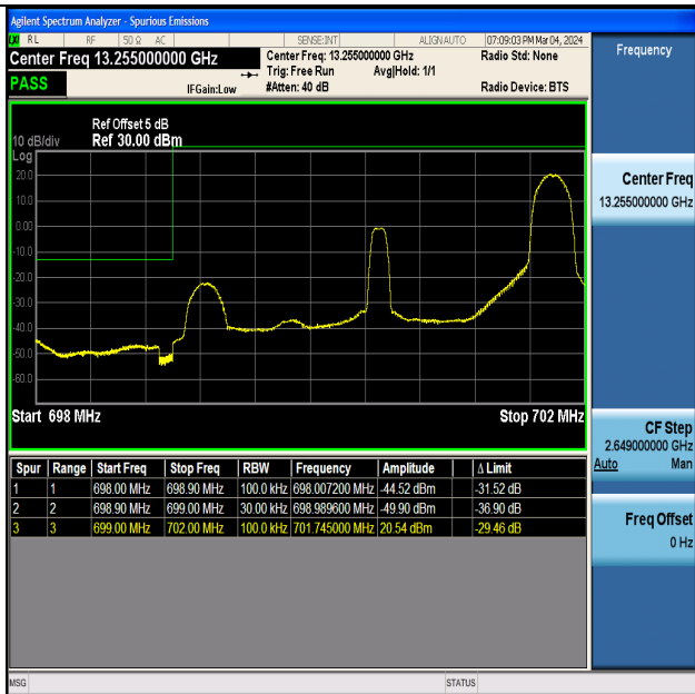
Band12_3MHz_QPSK_23025_1RB#14
