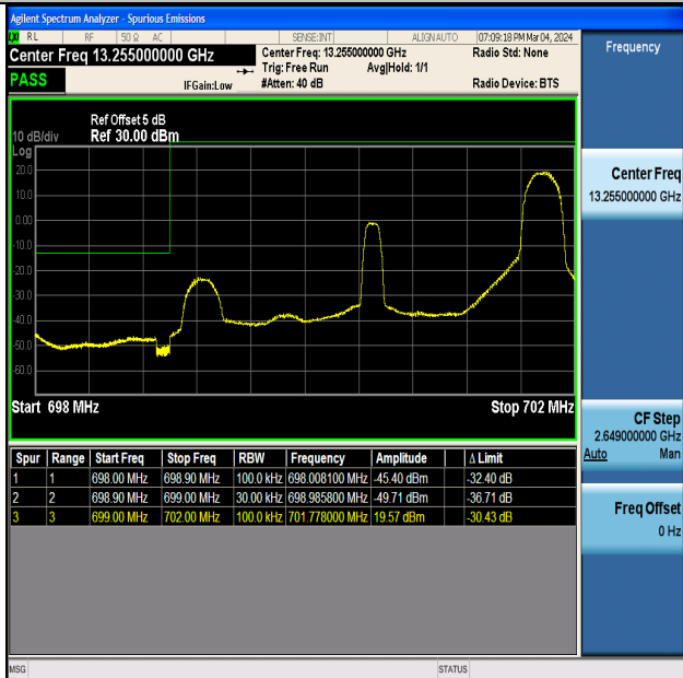
Band12_3MHz_16QAM_23025_1RB#14
