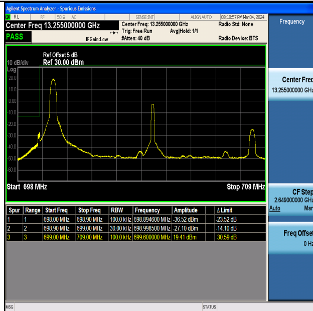
Band12_10MHz_16QAM_23060_1RB#0
