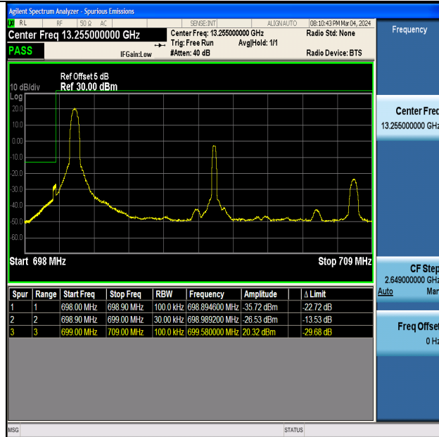
Band12_10MHz_QPSK_23060_1RB#0
