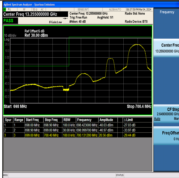
Band12_1.4MHz_QPSK_23017_1RB#5
