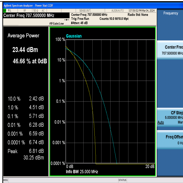
Band12-5MHz-QPSK-23095-25RB#0-PASS
