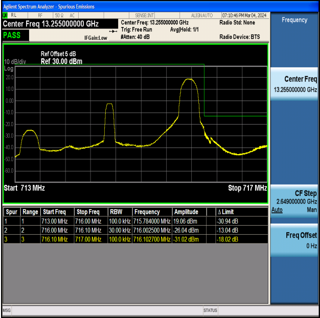
Band12_3MHz_16QAM_23165_1RB#14
