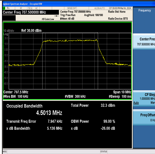
Band12-5MHz-QPSK-23095-25RB#0-PASS
