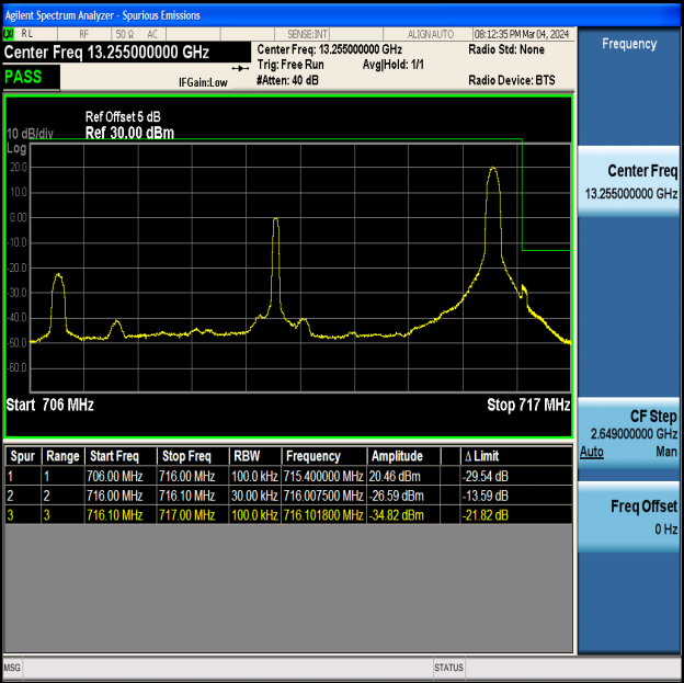
Band12_10MHz_QPSK_23130_1RB#49
