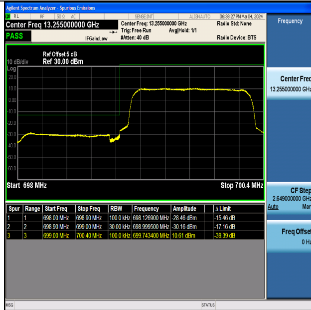
Band12_1.4MHz_QPSK_23017_6RB#0
