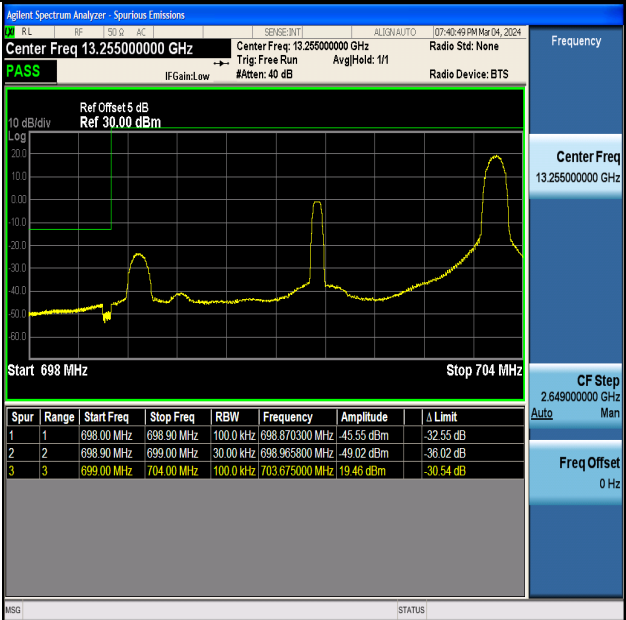
Band12_5MHz_16QAM_23035_1RB#24
