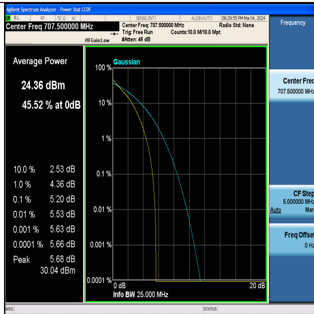
Band12-10MHz-QPSK-23095-1RB#0-PASS
