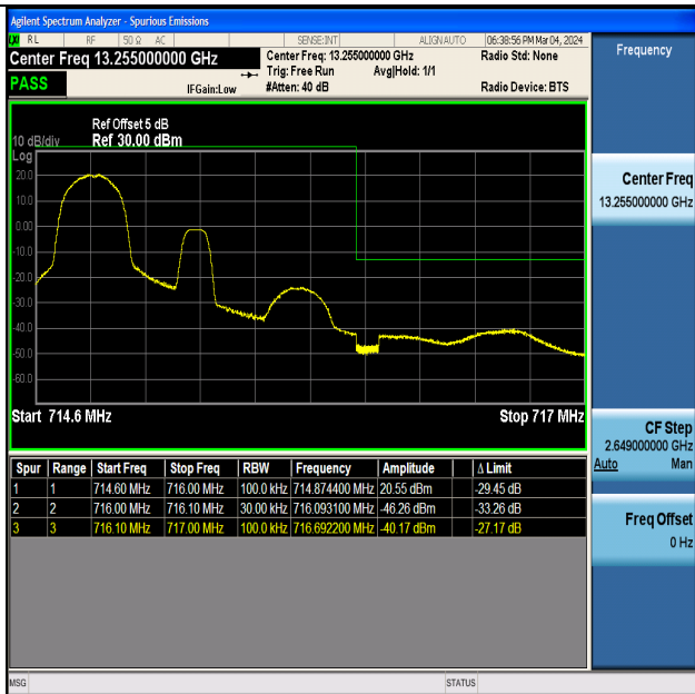
Band12_1.4MHz_QPSK_23173_1RB#0
