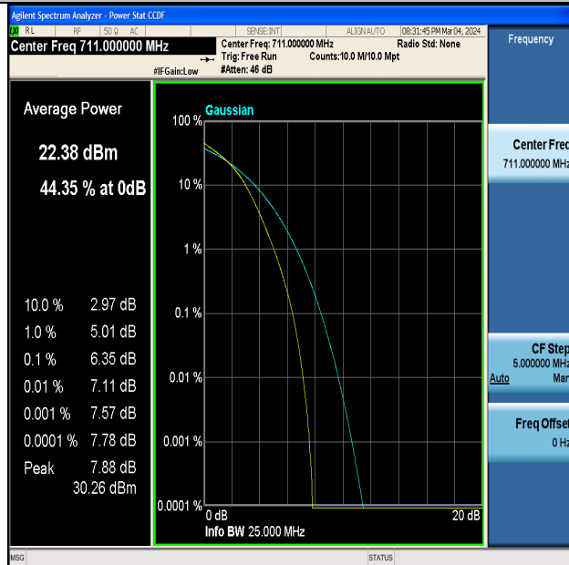
Band12-10MHz-16QAM-23130-50RB#0-PASS
