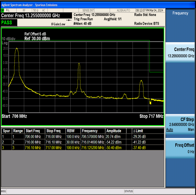
Band12_10MHz_QPSK_23130_1RB#0
