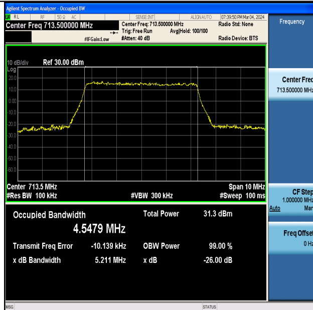
Band12-5MHz-16QAM-23155-25RB#0-PASS
