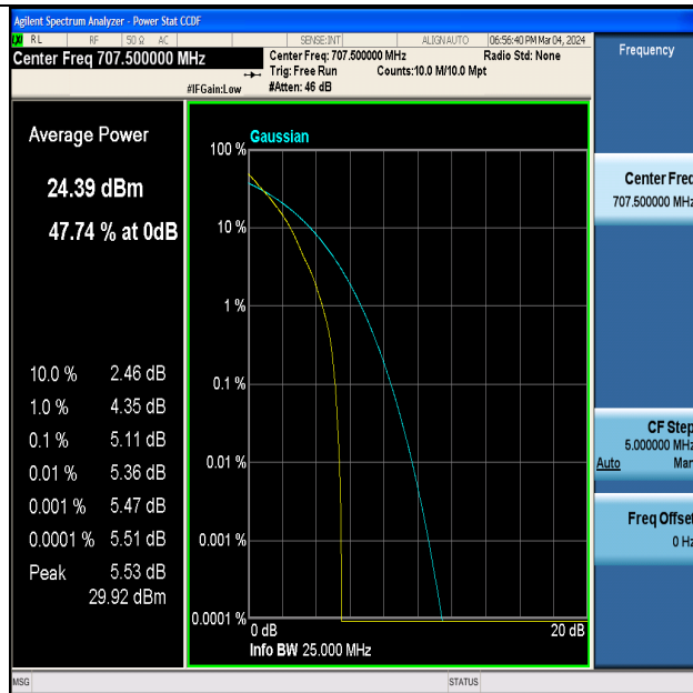
Band12-1.4MHz-QPSK-23095-1RB#0-PASS
