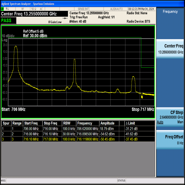
Band12_10MHz_16QAM_23130_1RB#0
