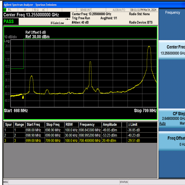
Band12_10MHz_QPSK_23060_1RB#49
