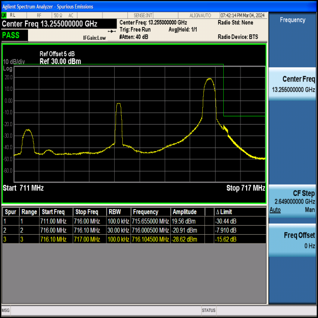
Band12_5MHz_16QAM_23155_1RB#24
