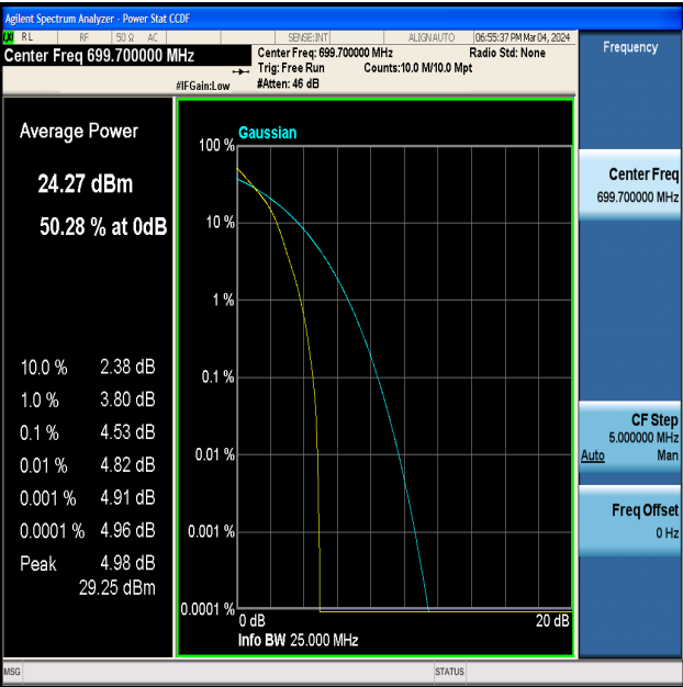
Band12-1.4MHz-QPSK-23017-1RB#0-PASS
