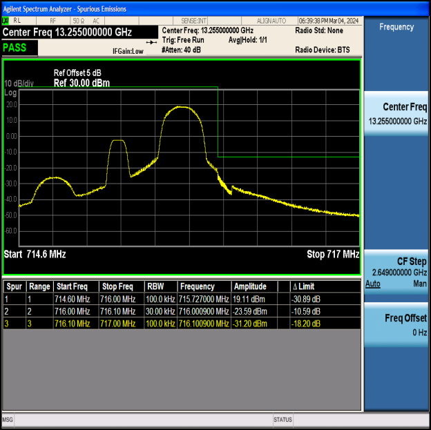
Band12_1.4MHz_16QAM_23173_1RB#5
