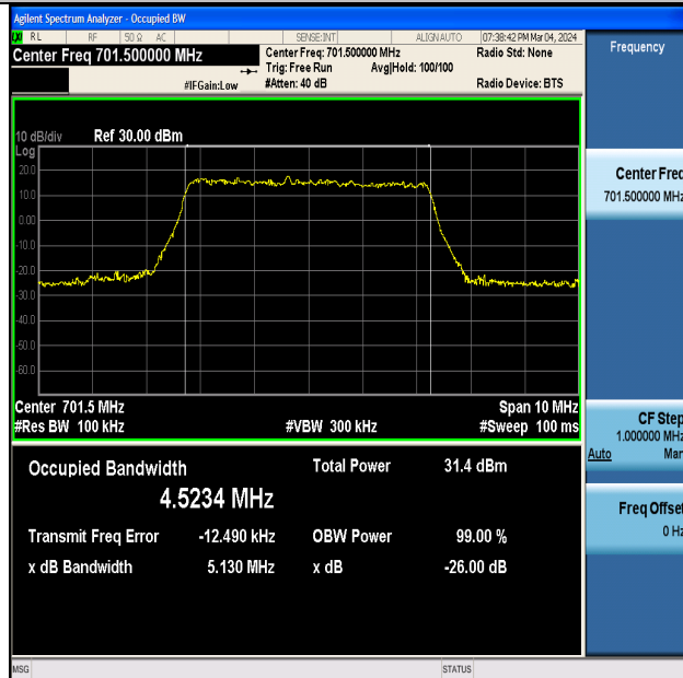
Band12-5MHz-16QAM-23035-25RB#0-PASS
