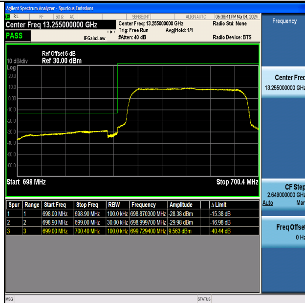
Band12_1.4MHz_16QAM_23017_6RB#0
