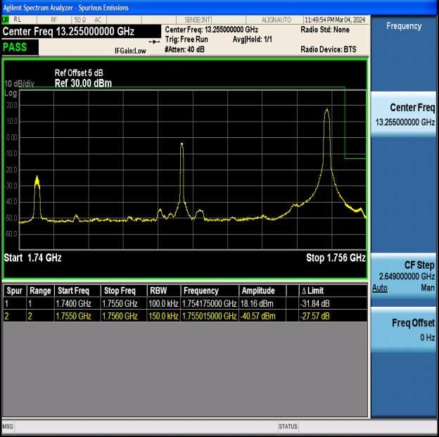
Band4_15MHz_16QAM_20325_1RB#74
