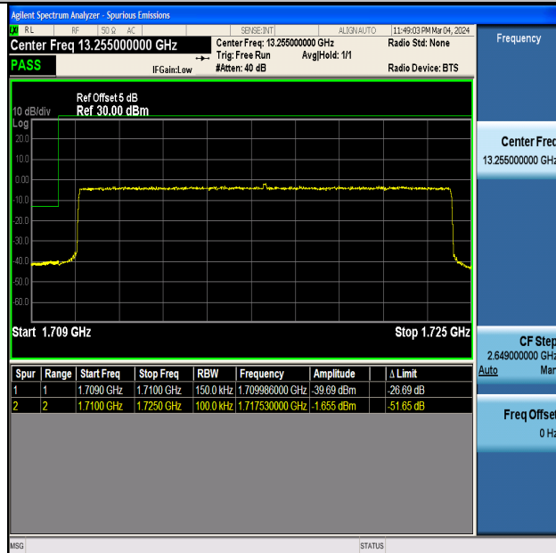
Band4_15MHz_16QAM_20025_75RB#0
