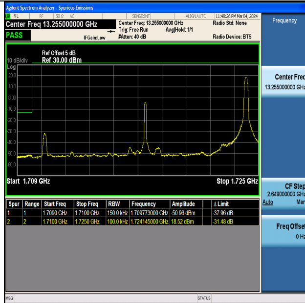
Band4_15MHz_QPSK_20025_1RB#74
