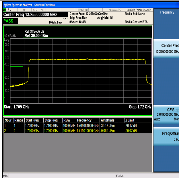
Band4_10MHz_16QAM_20000_50RB#0
