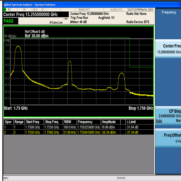
Band4_5MHz_QPSK_20375_1RB#0
