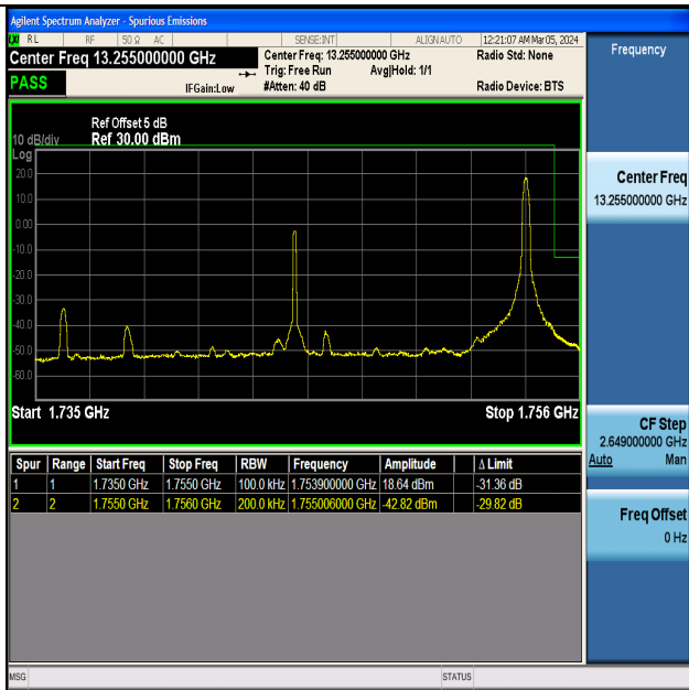
Band4_20MHz_QPSK_20300_1RB#99
