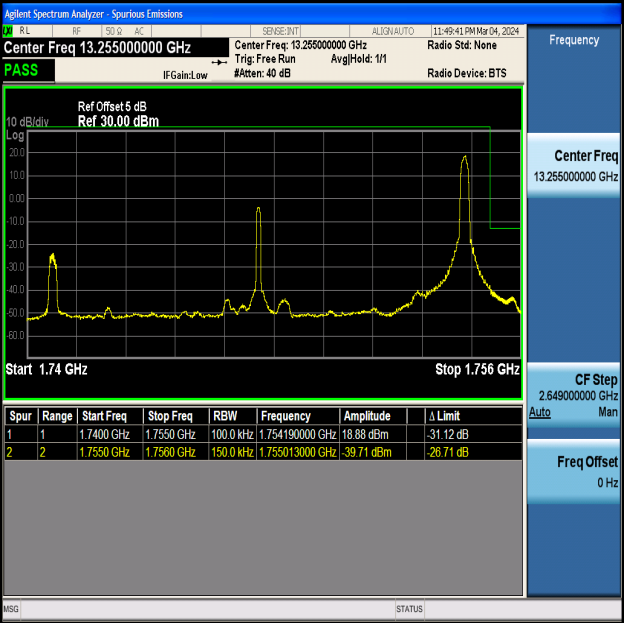
Band4_15MHz_QPSK_20325_1RB#74
