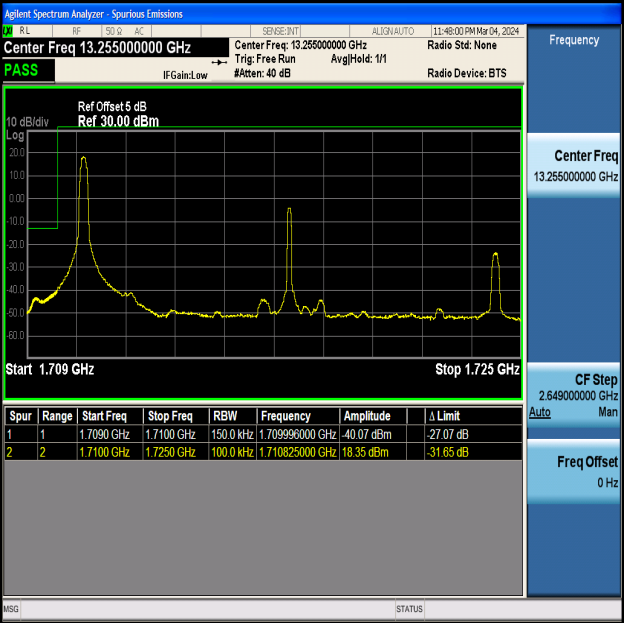
Band4_15MHz_QPSK_20025_1RB#0
