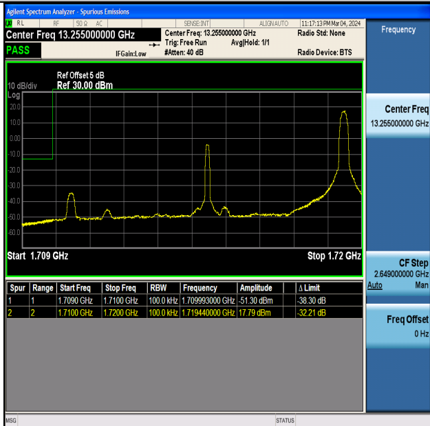
Band4_10MHz_16QAM_20000_1RB#49
