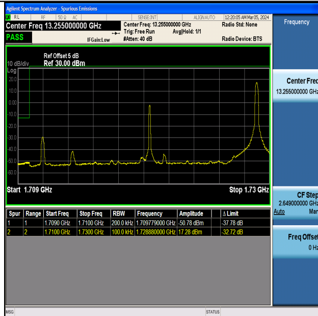
Band4_20MHz_16QAM_20050_1RB#99
