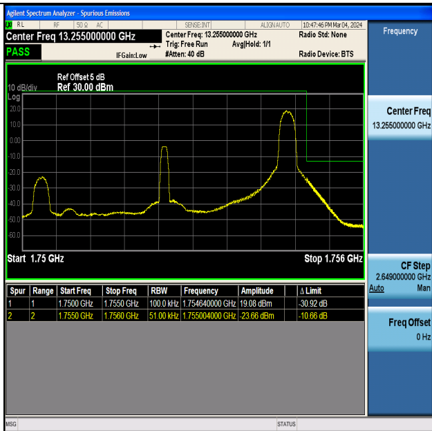
Band4_5MHz_QPSK_20375_1RB#24
