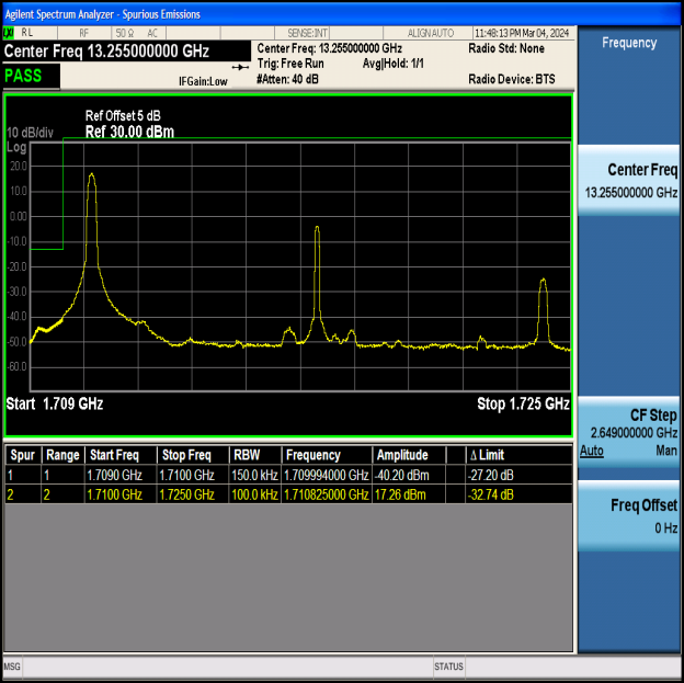
Band4_15MHz_16QAM_20025_1RB#0
