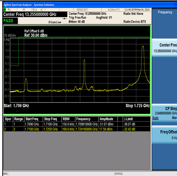
Band4_15MHz_16QAM_20025_1RB#74
