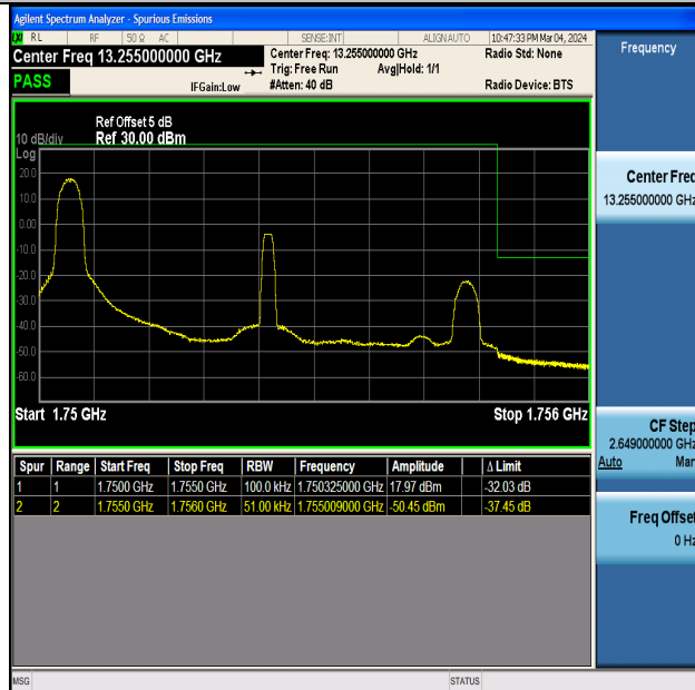
Band4_5MHz_16QAM_20375_1RB#0
