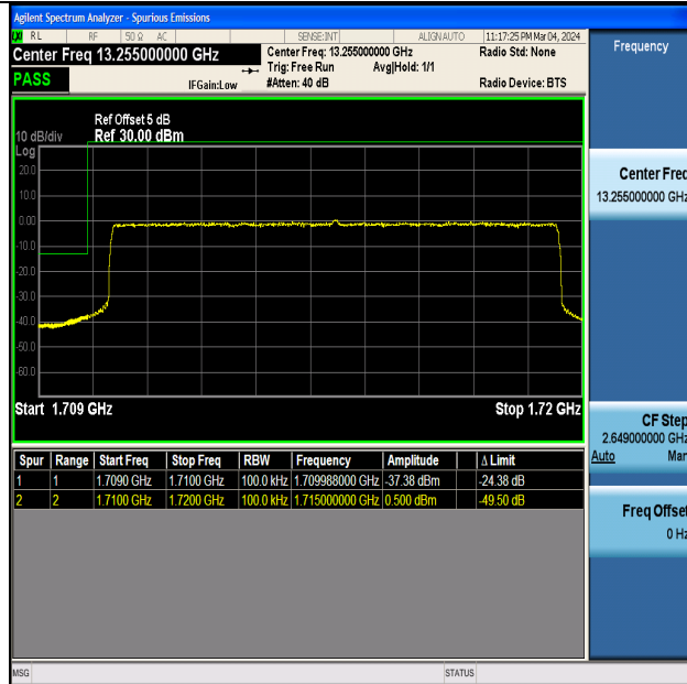
Band4_10MHz_QPSK_20000_50RB#0
