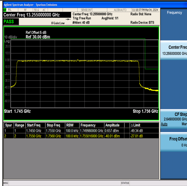
Band4_10MHz_QPSK_20350_50RB#0
