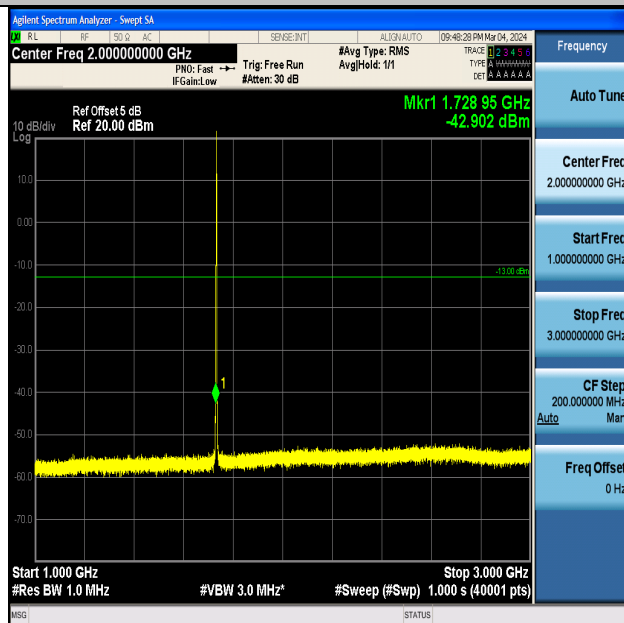
Band4_1.4MHz_QPSK_20175_1RB#0_1000~3000_1000~3000
