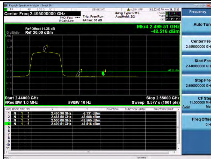
11N20SISO_Ant1_High_2462_AV
