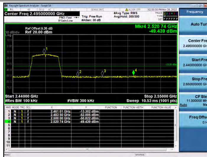
11N20SISO_Ant1_High_2462
