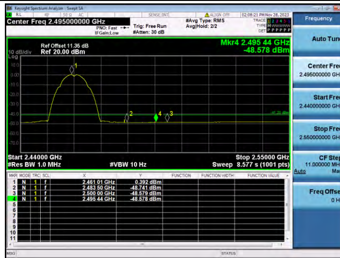
11B_Ant1_High_2462_AV
