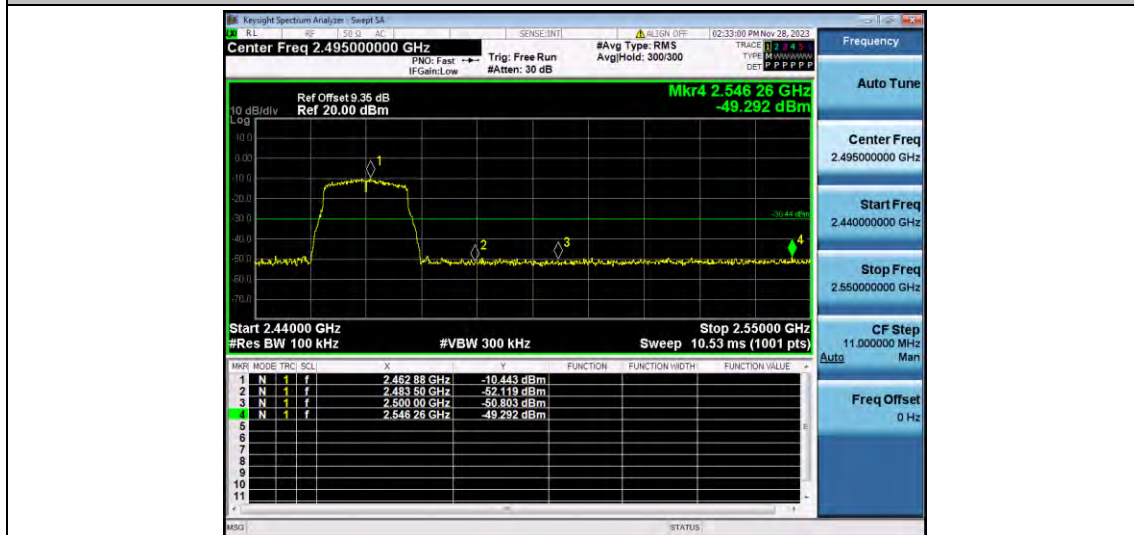
11G_Ant1_High_2462
