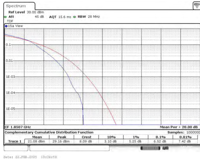
Band25-1.4MHz-16QAM-26365-6RB#0
