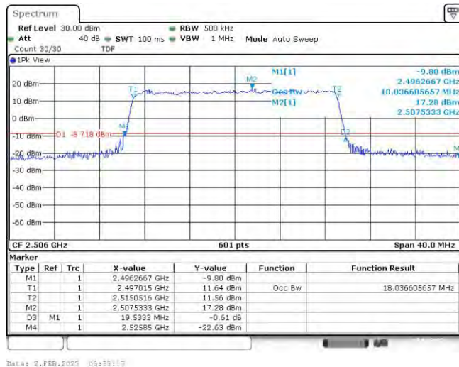
Band41-20MHz-QPSK-40690-100RB#0
