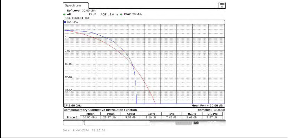
Band41-20MHz-QPSK-41490-100RB#0
