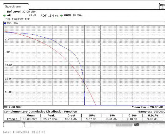
Band41-20MHz-16QAM-41490-100RB#0
