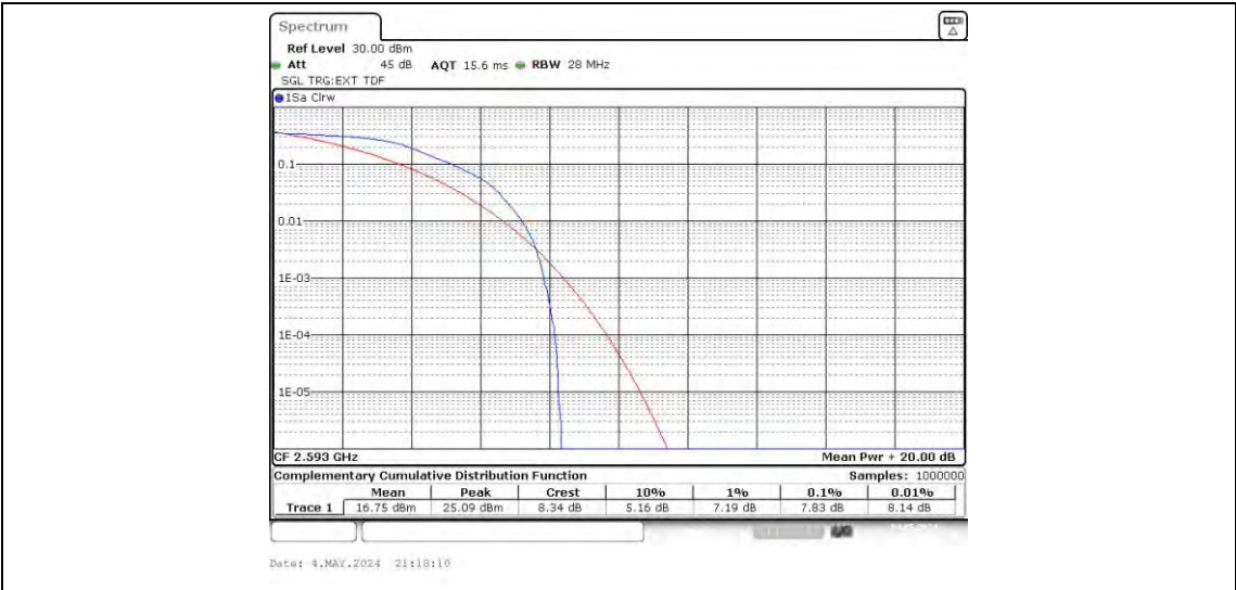
Band41-20MHz-QPSK-40620-100RB#0
