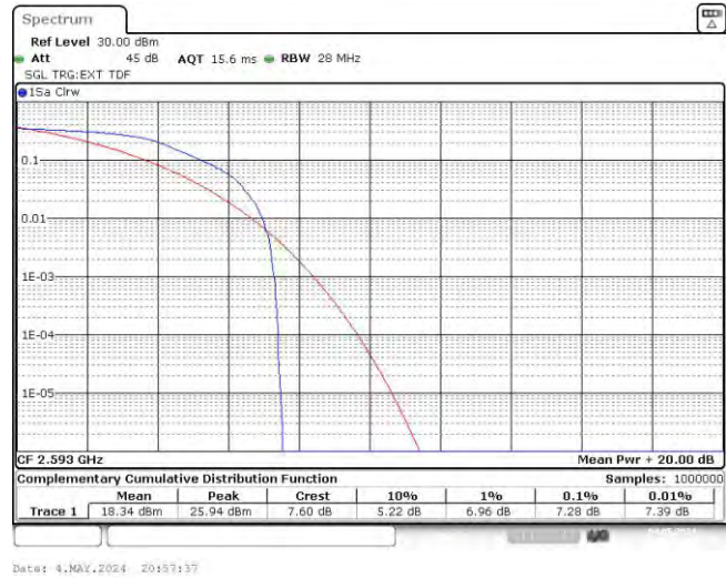
Band41-15MHz-QPSK-40620-75RB#0
