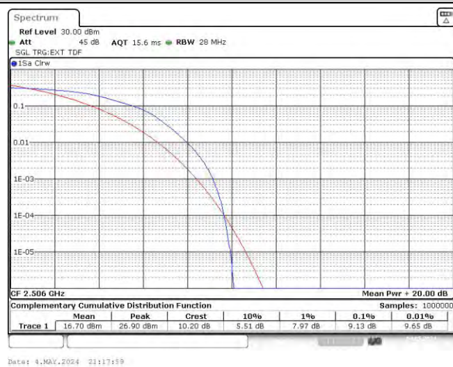
Band41-20MHz-16QAM-40620-1RB#0
