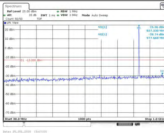
Band26-1.4MHz-QPSK-26915-6RB#0-Range1:30~1000MHz
