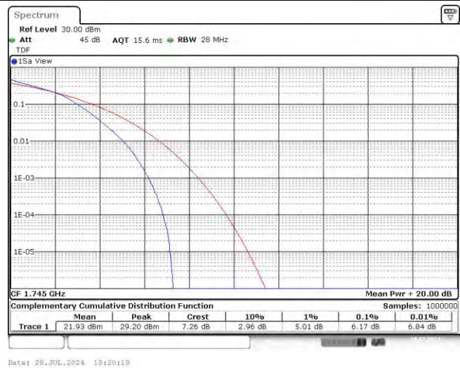
Band66-10MHz-16QAM-132622-50RB#0
