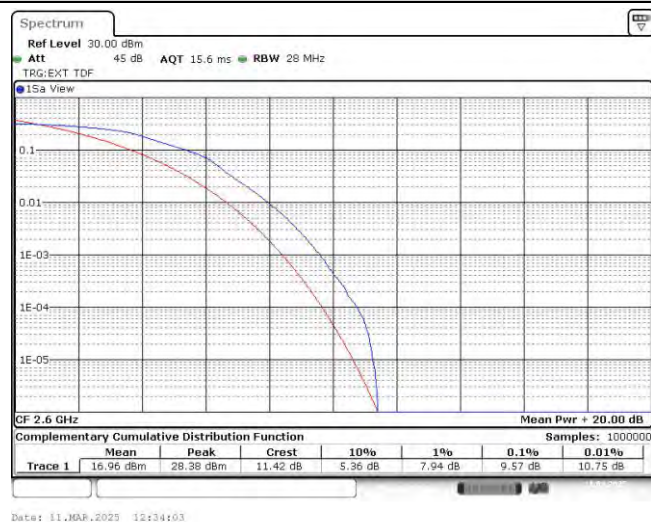
Band41-5MHz-QPSK-41215-25RB#0
