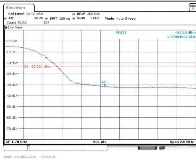
Band66-15MHz-16QAM-132047-75RB#0
