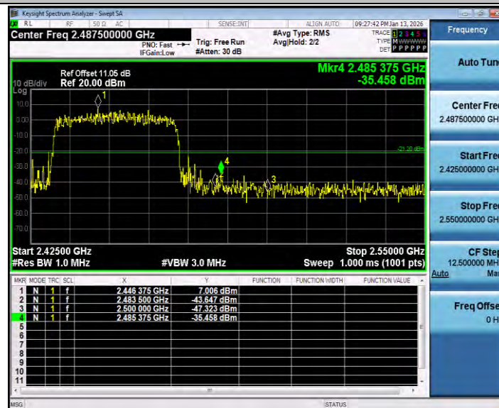
11AX40ISO_Ant1_High_2452_Peak
