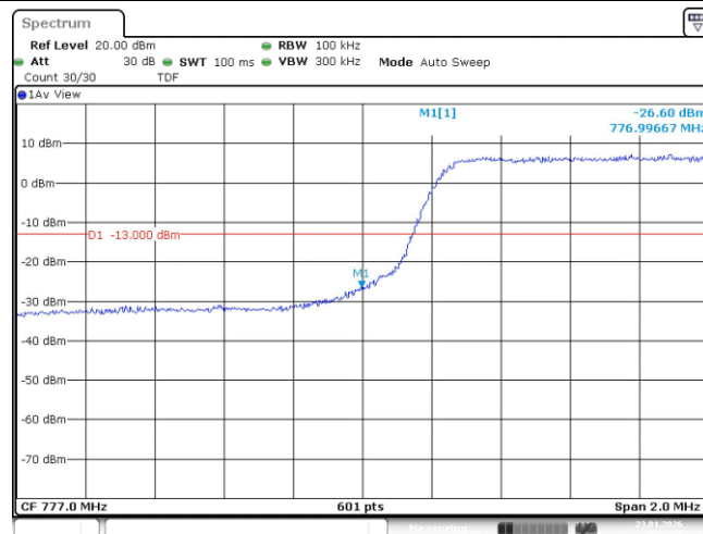
Band13-5MHz-16QAM-23205-25RB#0
