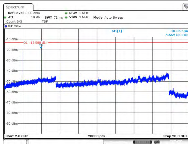
Band2-1.4MHz-QPSK-18607-6RB#0-Range3:2000~20000MHz
