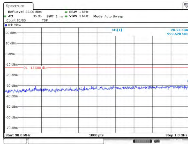
Band2-1.4MHz-QPSK-18607-6RB#0-Range1:30~1000MHz
