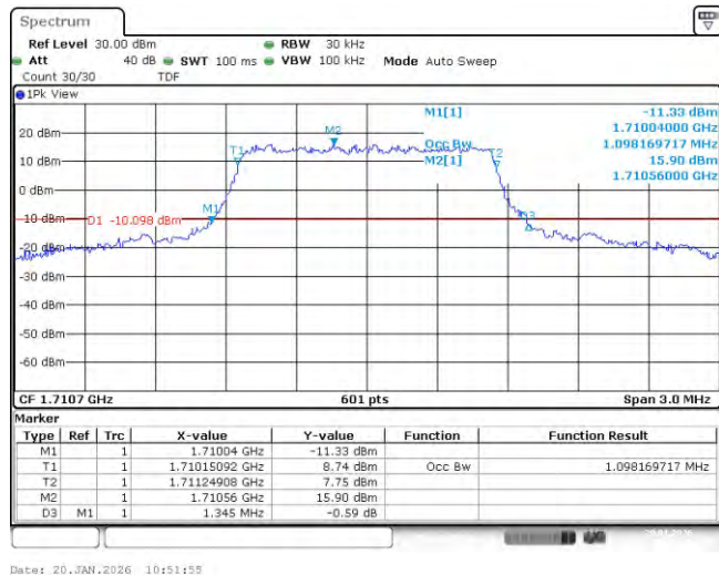
Band4-1.4MHz-QPSK-20175-6RB#0-1.098
