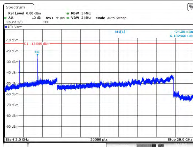
Band4-1.4MHz-QPSK-19957-6RB#0-Range3:2000~20000MHz
