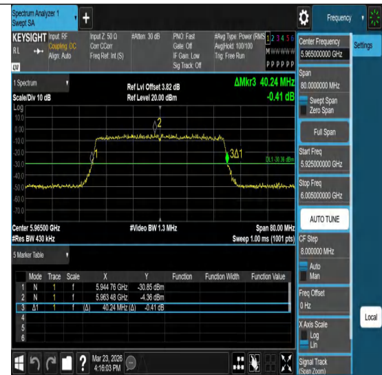
11ax40MIMO-Ant2-5965
