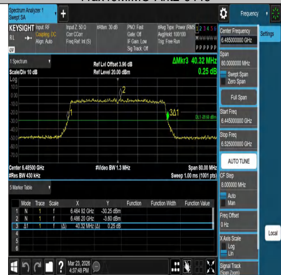
11ax40MIMO-Ant2-6485
