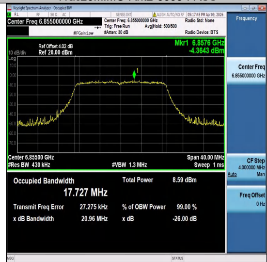
11ac20MIMO-Ant2-6855-PASS
