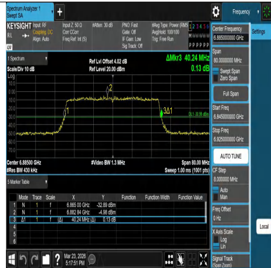
11ax40MIMO-Ant2-6885
