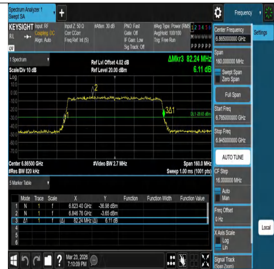
11ax80MIMO-Ant2-6865
