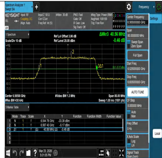
11ax40MIMO-Ant2-6565
