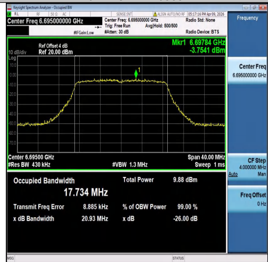
11ac20MIMO-Ant2-6695-PASS
