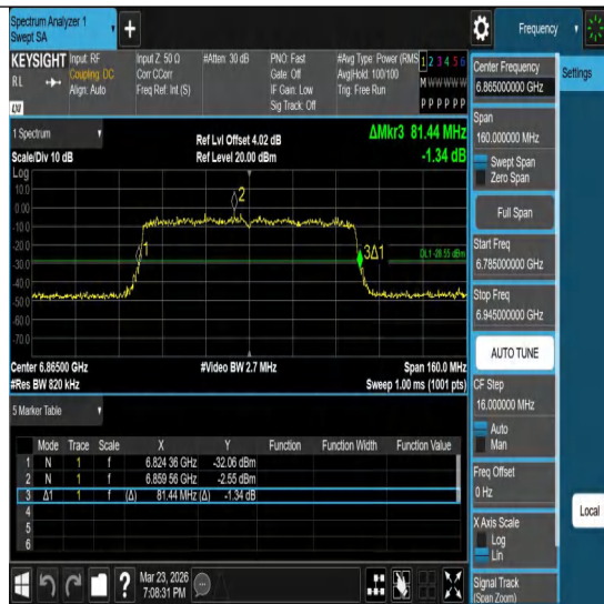
11ax80MIMO-Ant1-6865
