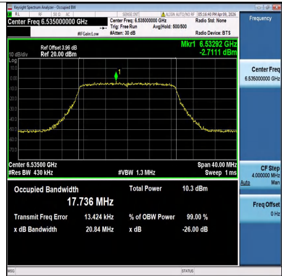
11ac20MIMO-Ant2-6535-PASS
