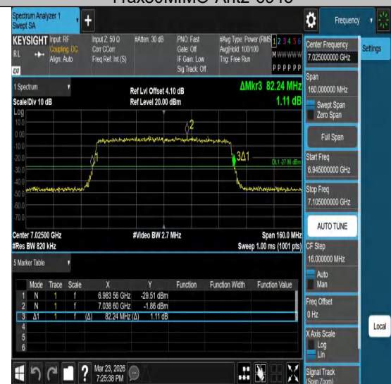
11ax80MIMO-Ant2-7025
