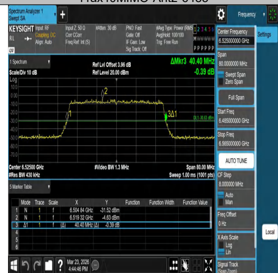
11ax40MIMO-Ant2-6525
