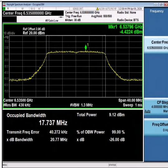
11ac20MIMO-Ant1-6535-PASS
