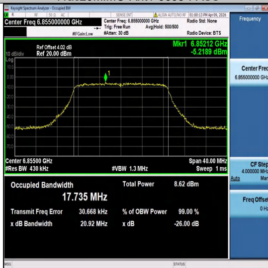
11ac20MIMO-Ant1-6855-PASS
