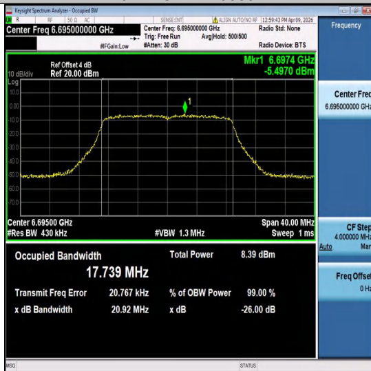
11ac20MIMO-Ant1-6695-PASS
