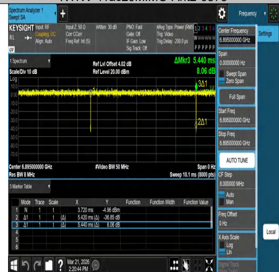
NTNV-11ac20MIMO-Ant2-6895
