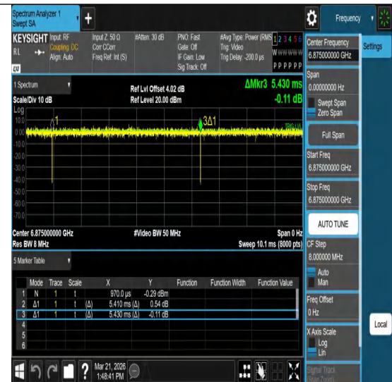
NTNV-11ac20MIMO-Ant2-6875
