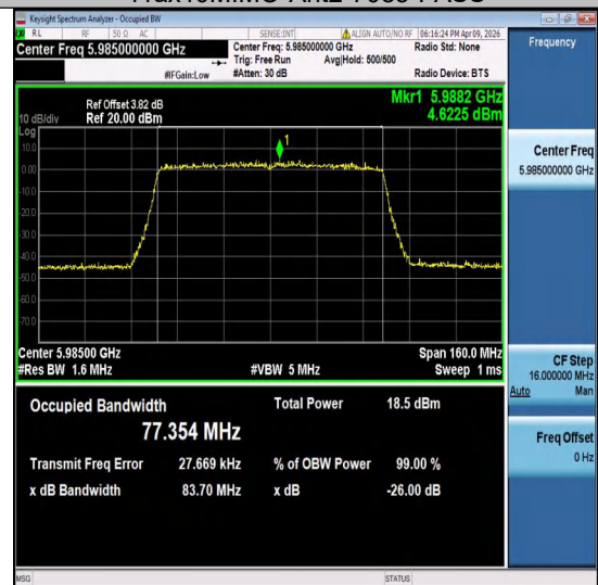
11ax80MIMO-Ant2-5985-PASS
