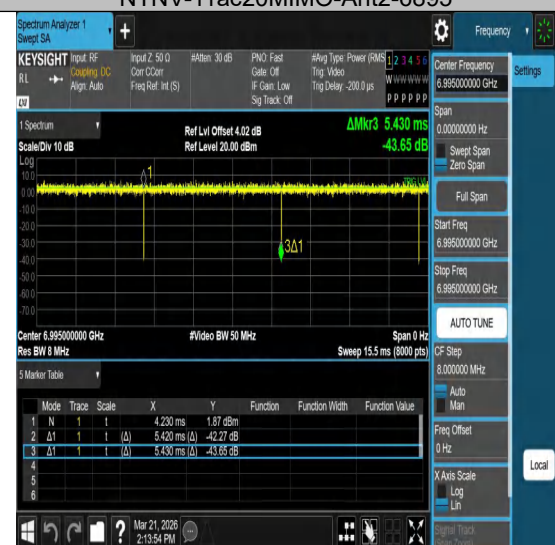
NTNV-11ac20MIMO-Ant2-6995
