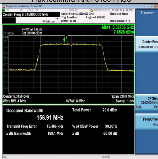
11ax160MIMO-Ant1-6345-PASS
