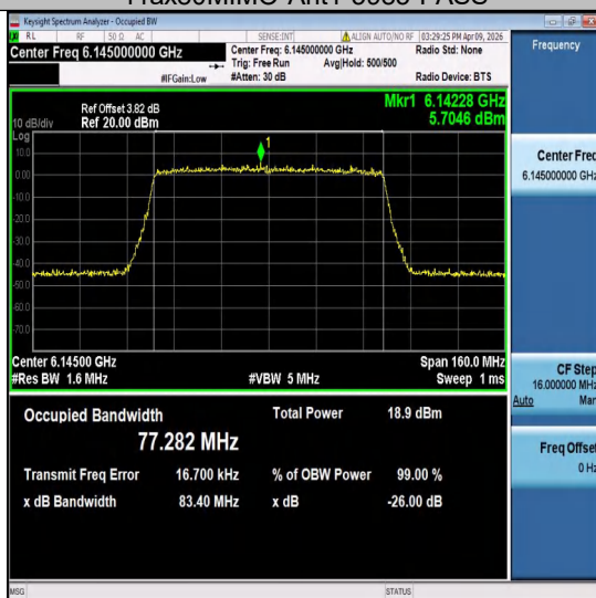
11ax80MIMO-Ant1-6145-PASS
