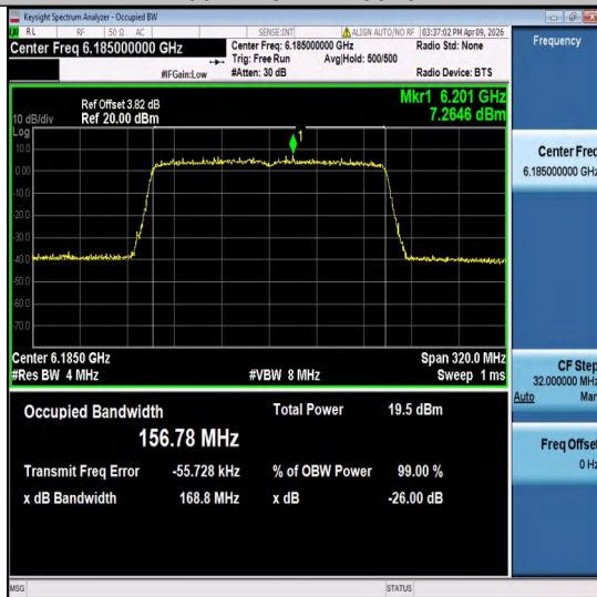
11ax160MIMO-Ant1-6185-PASS
