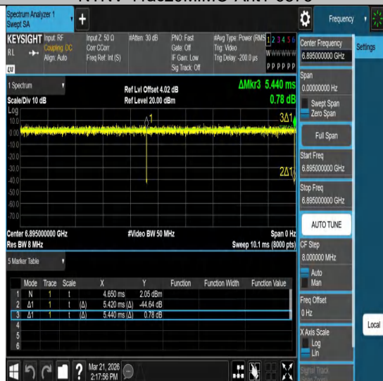
NTNV-11ac20MIMO-Ant1-6895
