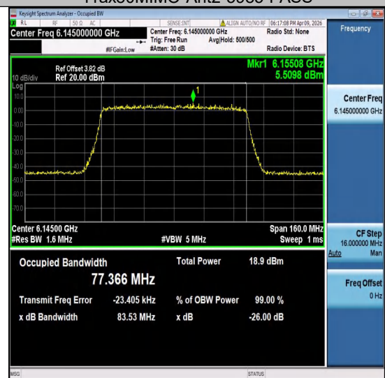
11ax80MIMO-Ant2-6145-PASS
