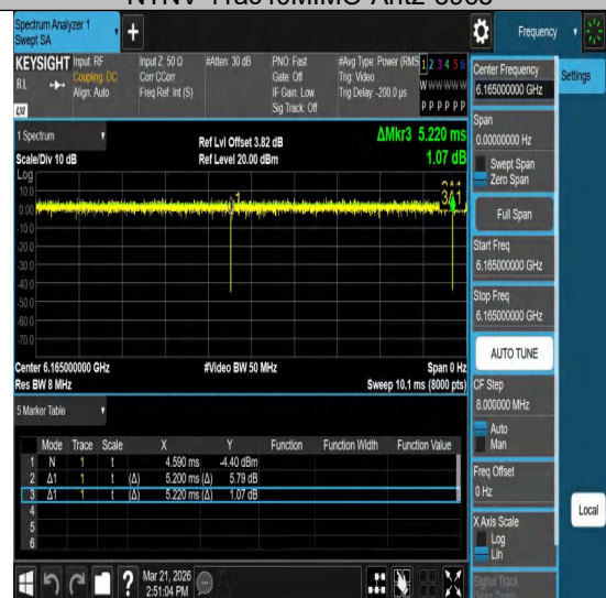
NTNV-11ac40MIMO-Ant2-6165
