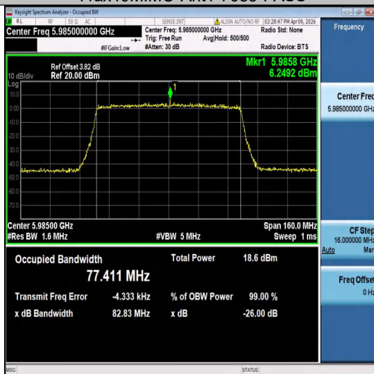
11ax80MIMO-Ant1-5985-PASS
