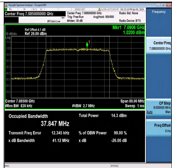
11ax40MIMO-Ant2-7085-PASS
