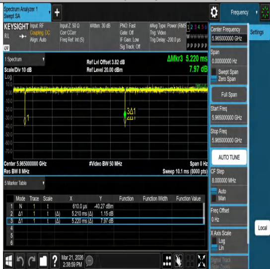
NTNV-11ac40MIMO-Ant1-5965
