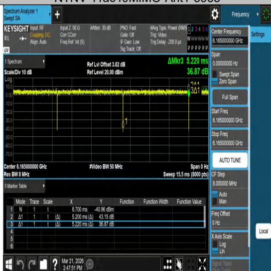
NTNV-11ac40MIMO-Ant1-6165
