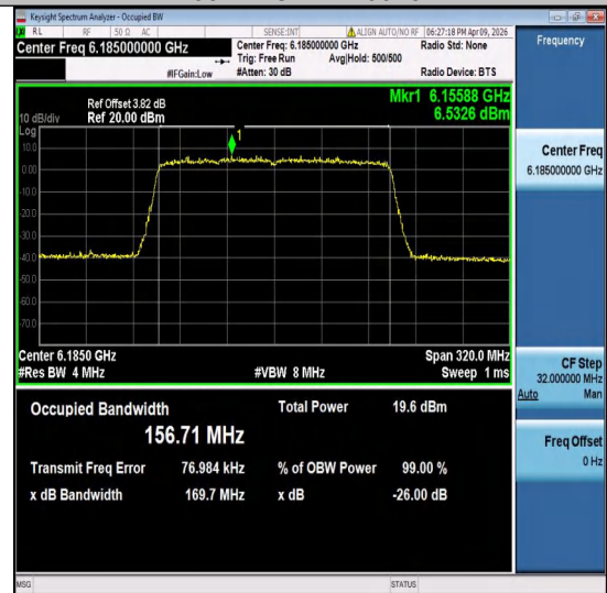
11ax160MIMO-Ant2-6185-PASS
