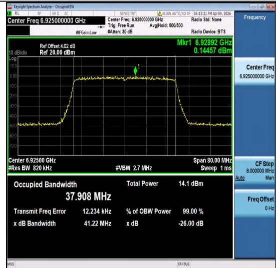
11ax40MIMO-Ant2-6925-PASS
