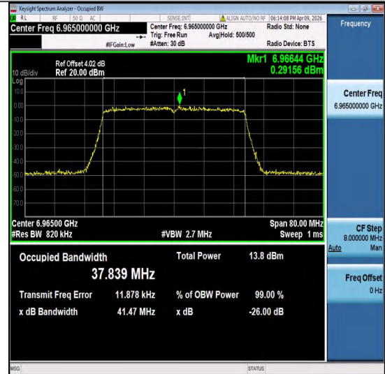
11ax40MIMO-Ant2-6965-PASS
