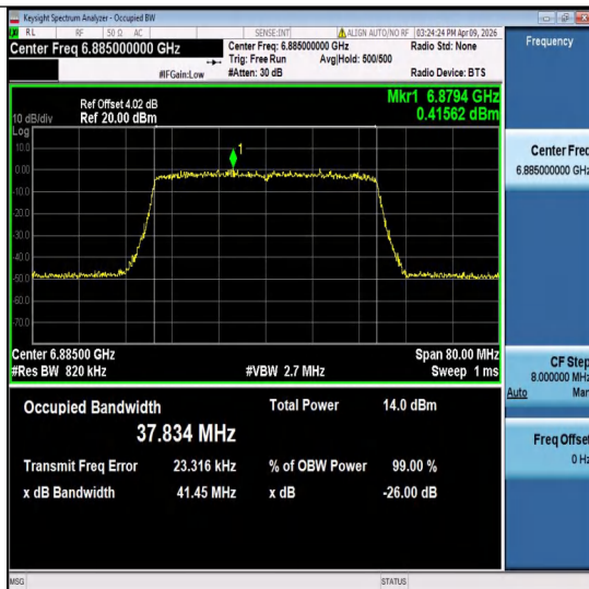
11ax40MIMO-Ant1-6885-PASS
