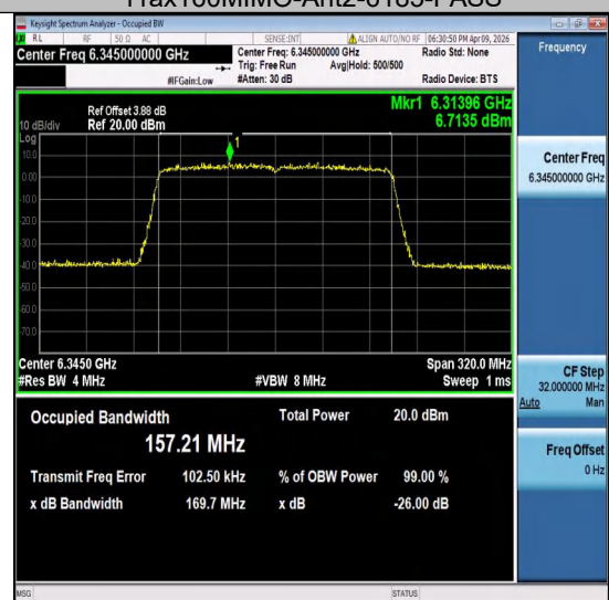
11ax160MIMO-Ant2-6345-PASS
