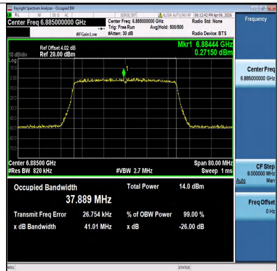
11ax40MIMO-Ant2-6885-PASS
