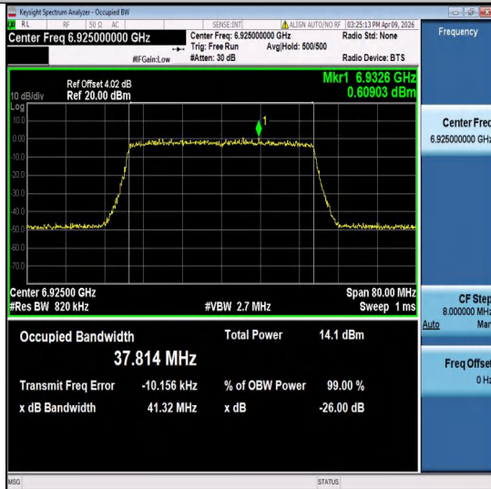
11ax40MIMO-Ant1-6925-PASS
