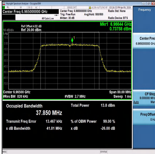
11ax40MIMO-Ant1-6965-PASS
