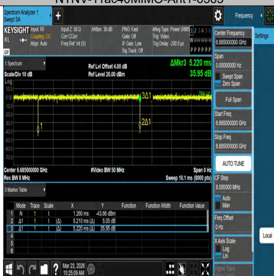
NTNV-11ac40MIMO-Ant1-6685
