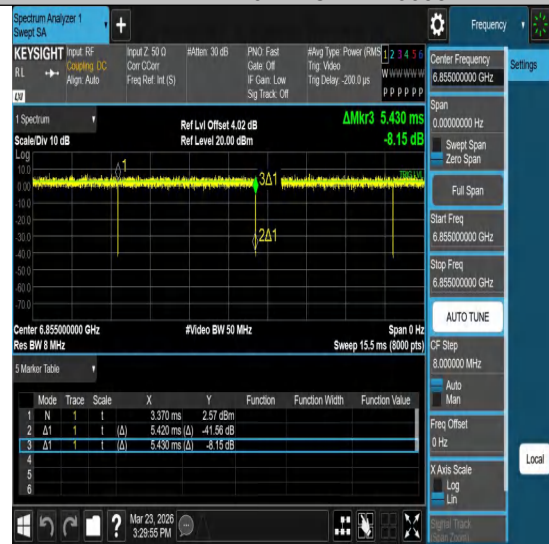
NTNV-11ax20MIMO-Ant2-6855
