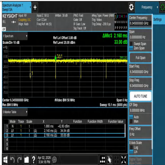
NTNV-11ac160MIMO-Ant1-6345
