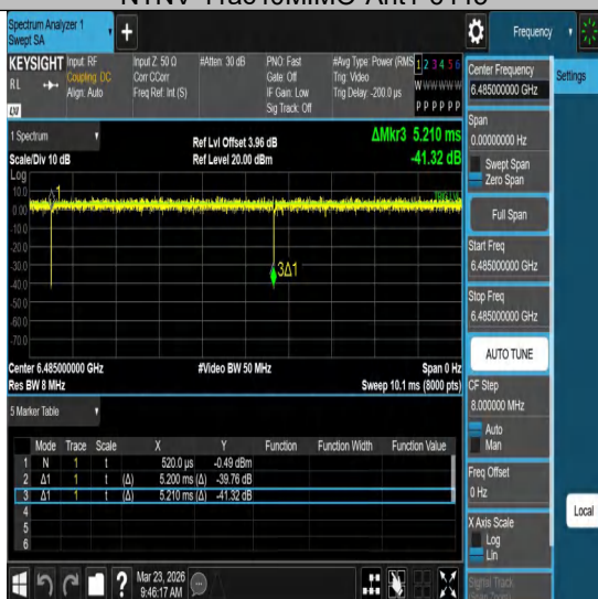
NTNV-11ac40MIMO-Ant1-6485
