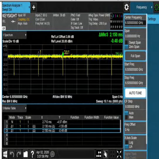
NTNV-11ac160MIMO-Ant1-6505
