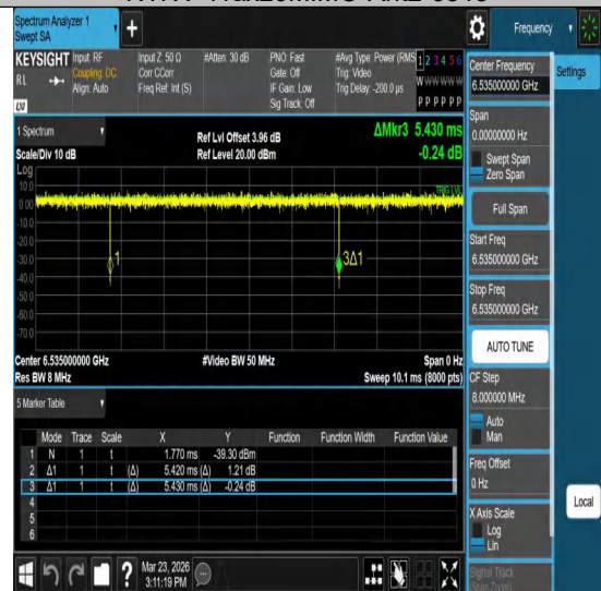
NTNV-11ax20MIMO-Ant2-6535
