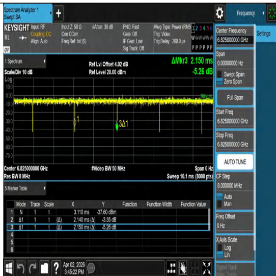
NTNV-11ac160MIMO-Ant1-6825
