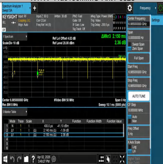
NTNV-11ac160MIMO-Ant1-6985
