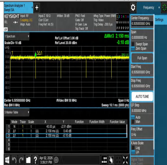
NTNV-11ac160MIMO-Ant2-6505
