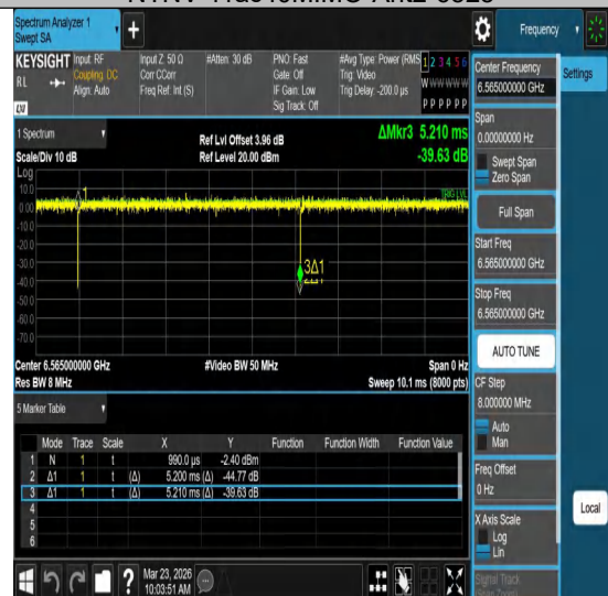
NTNV-11ac40MIMO-Ant2-6565
