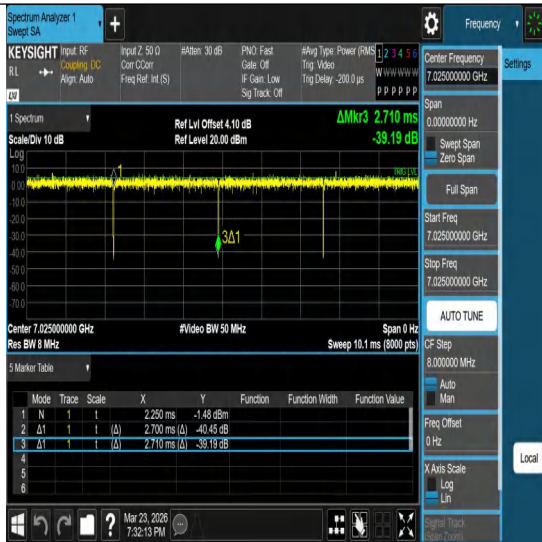
NTNV-11ac80MIMO-Ant1-7025
