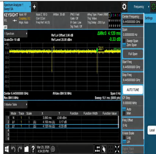
NTNV-11ax40MIMO-Ant2-6445
