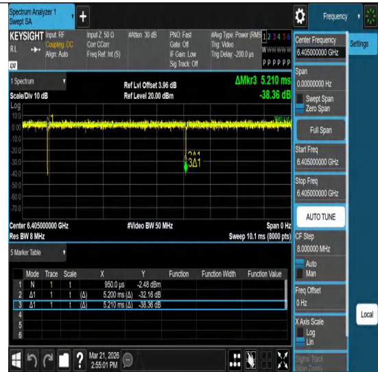
NTNV-11ac40MIMO-Ant2-6405
