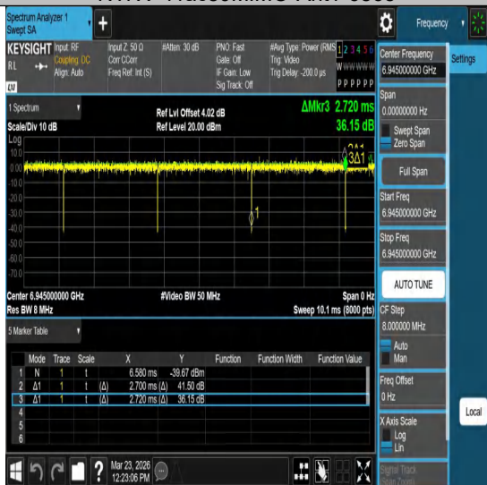
NTNV-11ac80MIMO-Ant1-6945
