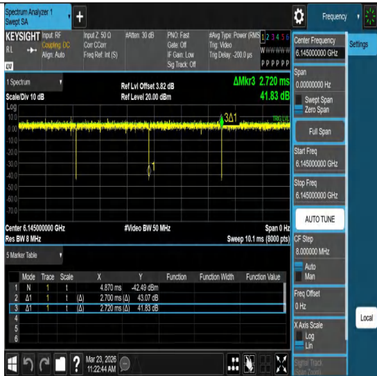
NTNV-11ac80MIMO-Ant1-6145
