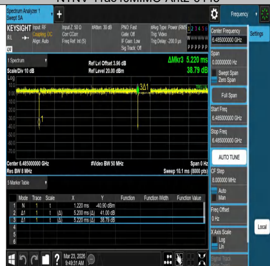
NTNV-11ac40MIMO-Ant2-6485
