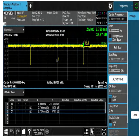
NTNV-11ac80MIMO-Ant2-7025
