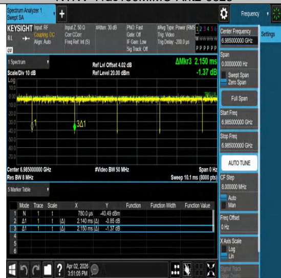
NTNV-11ac160MIMO-Ant2-6985
