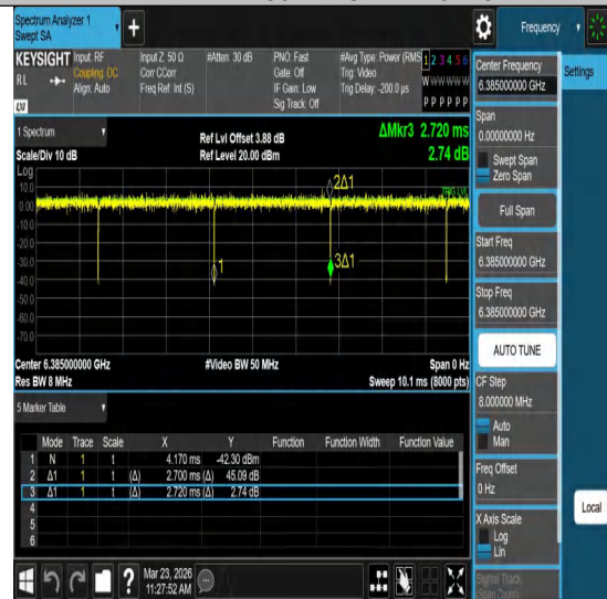
NTNV-11ac80MIMO-Ant2-6385
