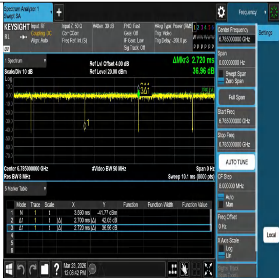
NTNV-11ac80MIMO-Ant1-6785
