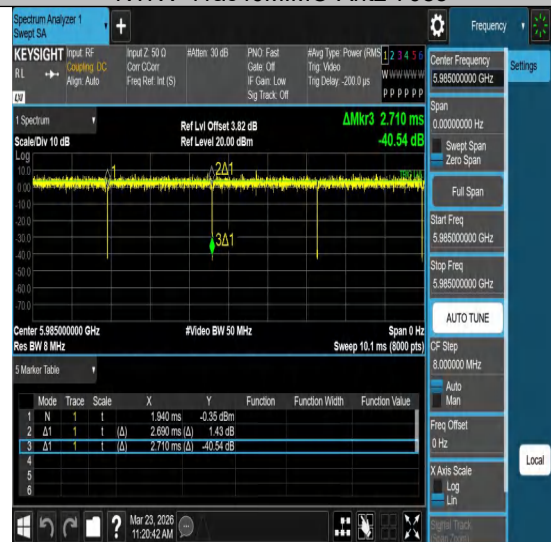
NTNV-11ac80MIMO-Ant2-5985
