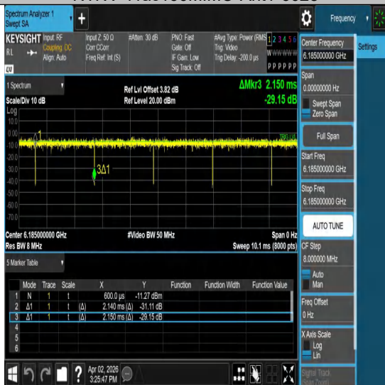
NTNV-11ac160MIMO-Ant1-6185
