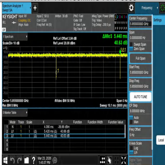
NTNV-11ax20MIMO-Ant1-5955
