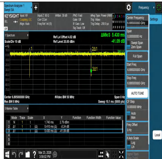
NTNV-11ax20MIMO-Ant2-6895
