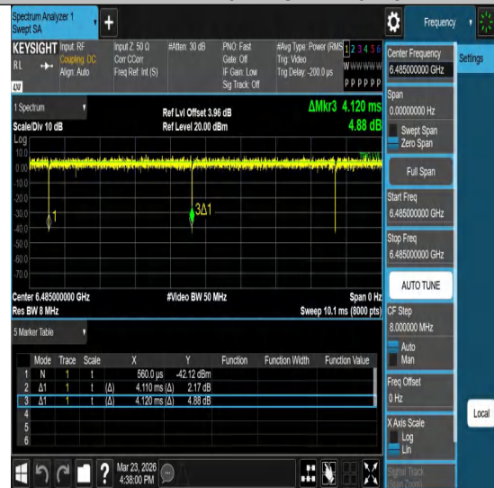
NTNV-11ax40MIMO-Ant2-6485
