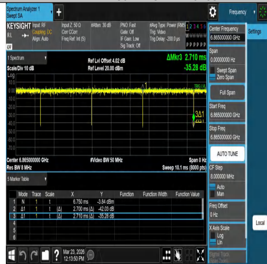
NTNV-11ac80MIMO-Ant2-6865
