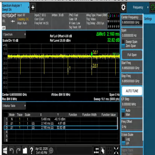
NTNV-11ac160MIMO-Ant1-6665
