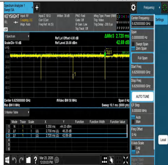
NTNV-11ac80MIMO-Ant2-6625
