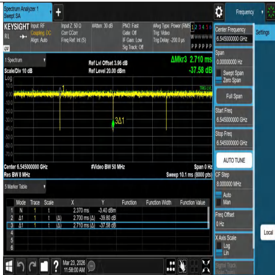
NTNV-11ac80MIMO-Ant1-6545
