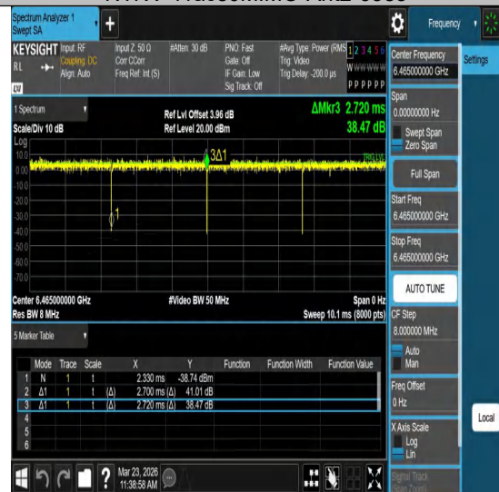
NTNV-11ac80MIMO-Ant2-6465
