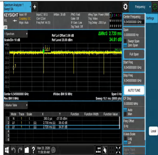
NTNV-11ac80MIMO-Ant2-6545
