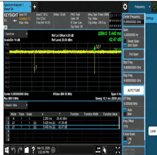
NTNV-11ax20MIMO-Ant2-6695
