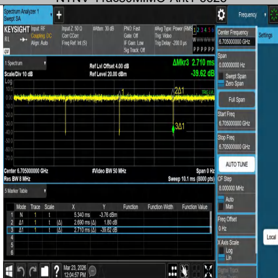
NTNV-11ac80MIMO-Ant1-6705
