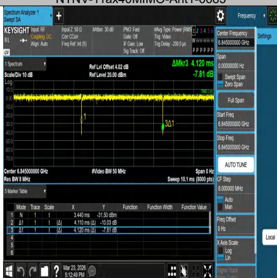
NTNV-11ax40MIMO-Ant1-6845
