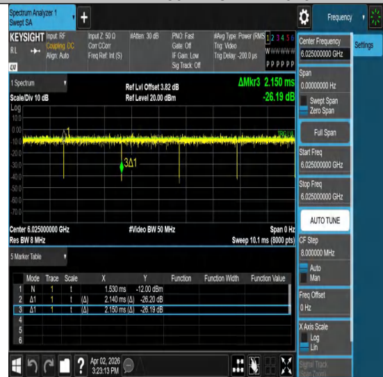
NTNV-11ac160MIMO-Ant2-6025
