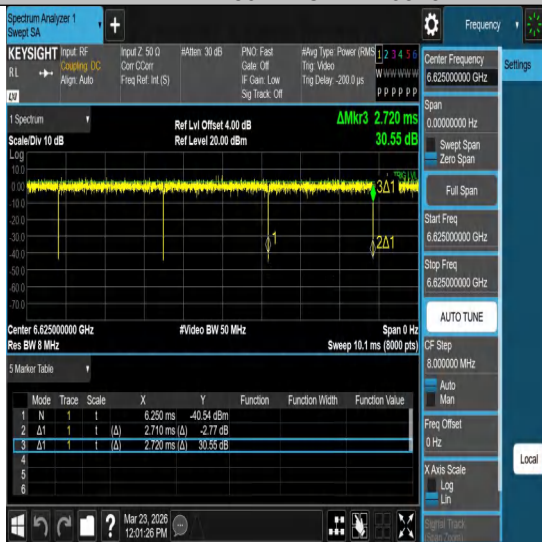
NTNV-11ac80MIMO-Ant1-6625
