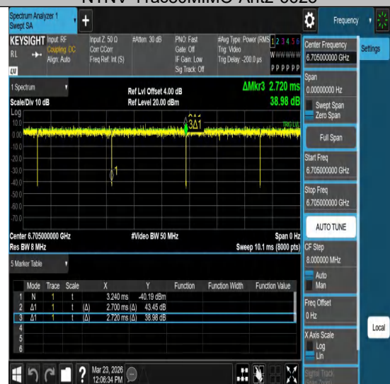
NTNV-11ac80MIMO-Ant2-6705
