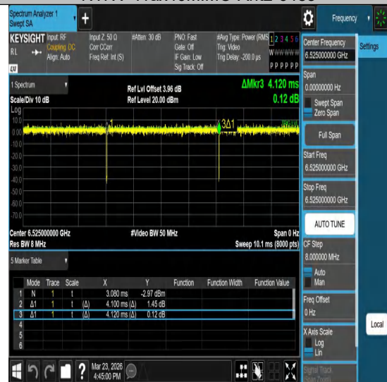
NTNV-11ax40MIMO-Ant2-6525
