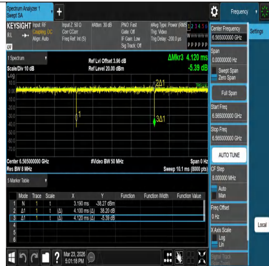
NTNV-11ax40MIMO-Ant2-6565
