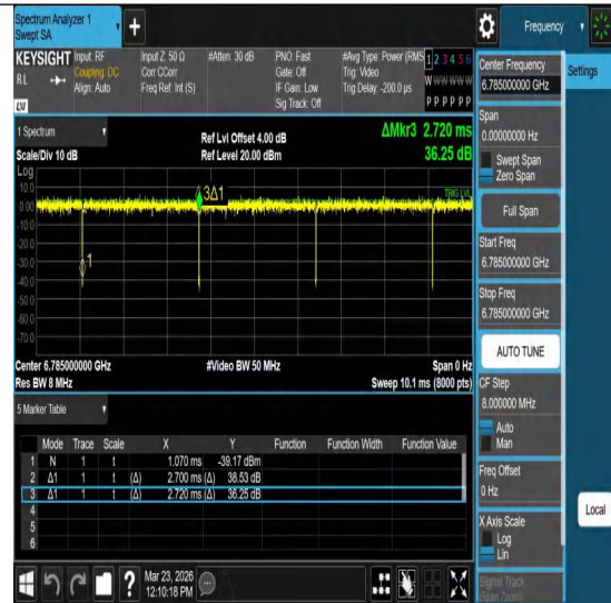
NTNV-11ac80MIMO-Ant2-6785
