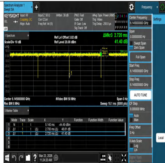
NTNV-11ac80MIMO-Ant2-6145
