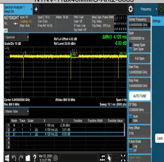
NTNV-11ax40MIMO-Ant2-6845
