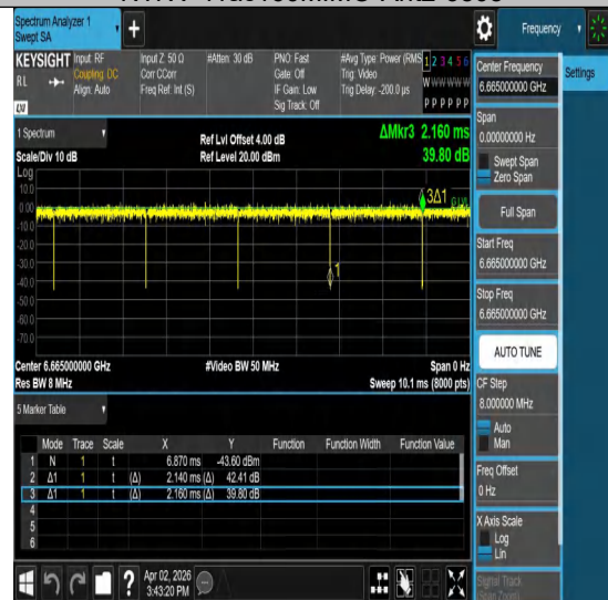
NTNV-11ac160MIMO-Ant2-6665
