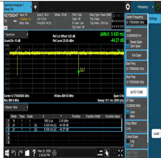
NTNV-11ax20MIMO-Ant2-6175
