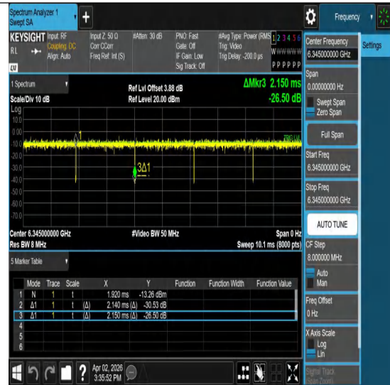
NTNV-11ac160MIMO-Ant2-6345
