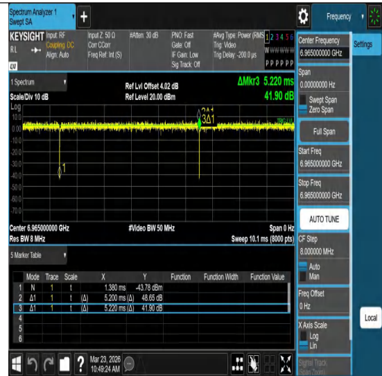
NTNV-11ac40MIMO-Ant2-6965
