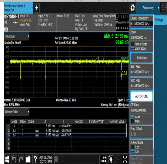
NTNV-11ac160MIMO-Ant2-6185
