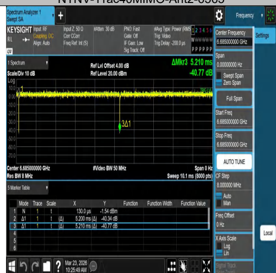
NTNV-11ac40MIMO-Ant2-6685
