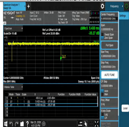
NTNV-11ax20MIMO-Ant2-6995
