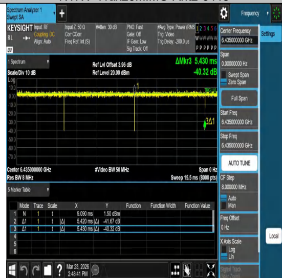
NTNV-11ax20MIMO-Ant2-6435
