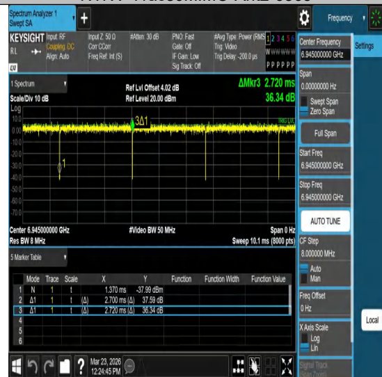
NTNV-11ac80MIMO-Ant2-6945
