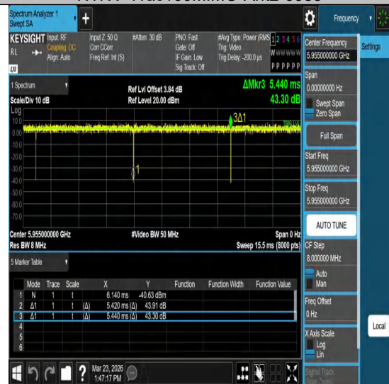
NTNV-11ax20MIMO-Ant2-5955
