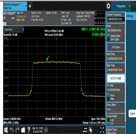
11ax80MIMO-Ant2-5985-PASS
