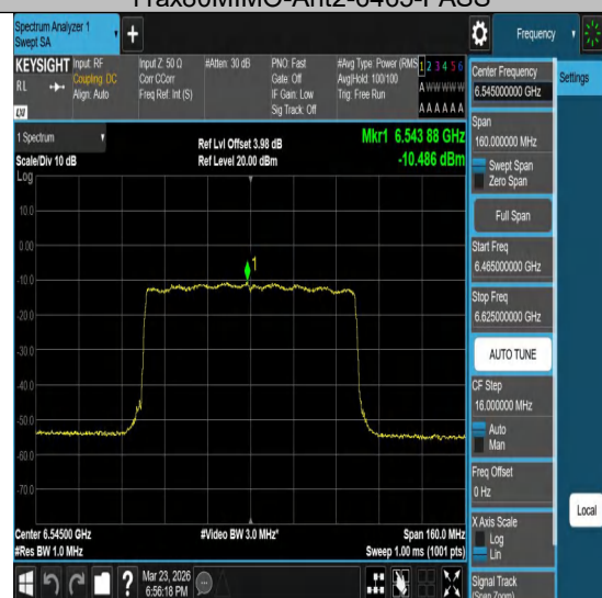
11ax80MIMO-Ant2-6545-PASS
