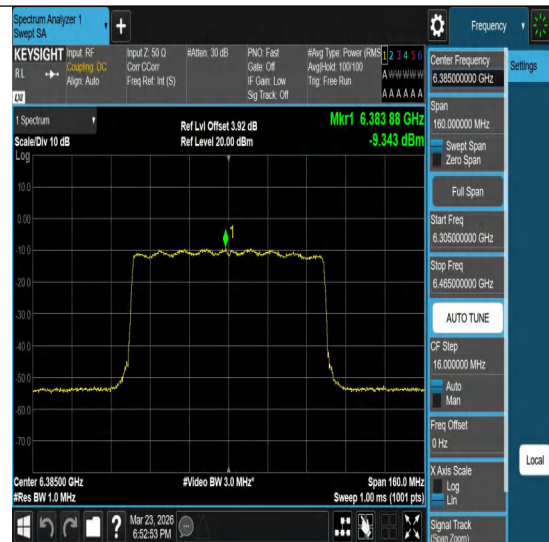
11ax80MIMO-Ant2-6385-PASS
