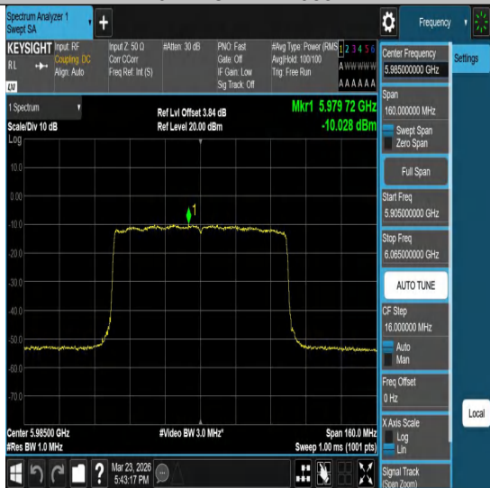
11ax80MIMO-Ant1-5985-PASS
