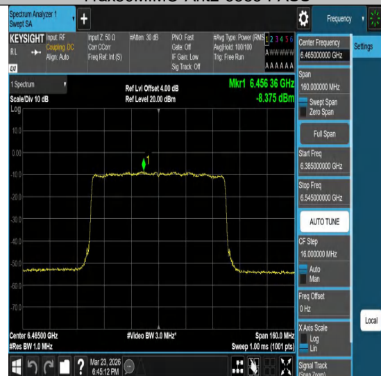
11ax80MIMO-Ant2-6465-PASS
