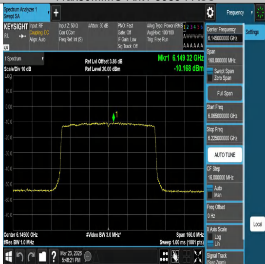
11ax80MIMO-Ant1-6145-PASS
