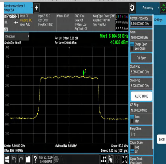
11ax80MIMO-Ant2-6145-PASS
