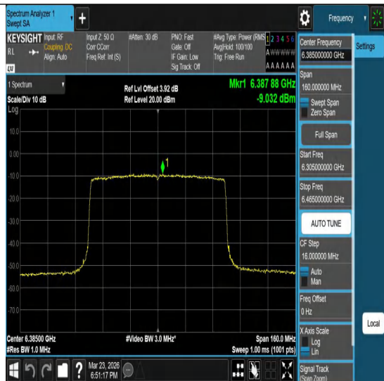
11ax80MIMO-Ant1-6385-PASS
