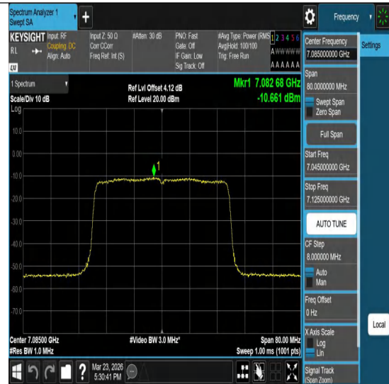
11ax40MIMO-Ant2-7085-PASS
