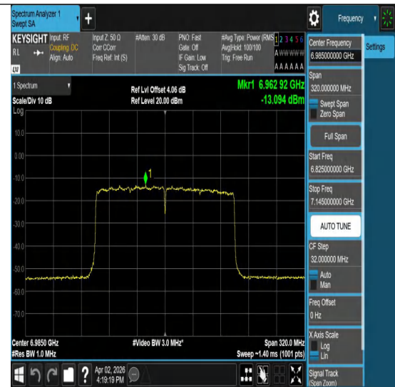
11ax160MIMO-Ant2-6985-PASS
