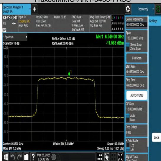
11ax80MIMO-Ant1-6545-PASS
