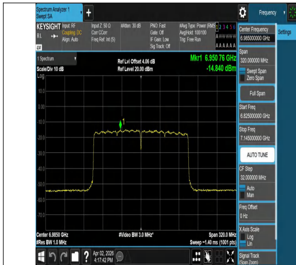
11ax160MIMO-Ant1-6985-PASS
