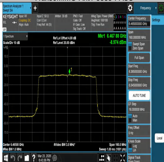
11ax80MIMO-Ant1-6465-PASS
