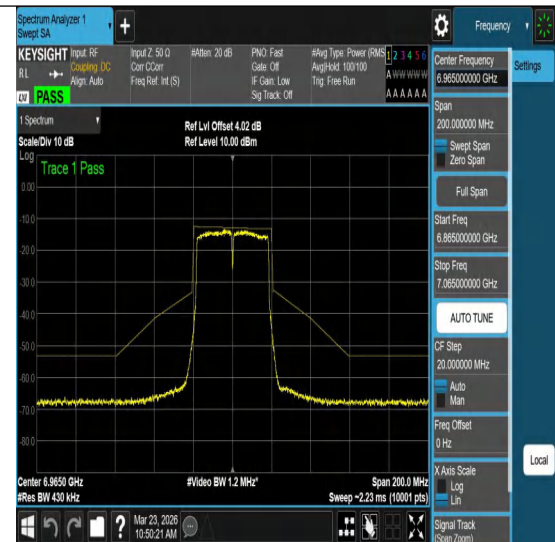
NTVN-11ac40MIMO-Ant2-6965-PASS
