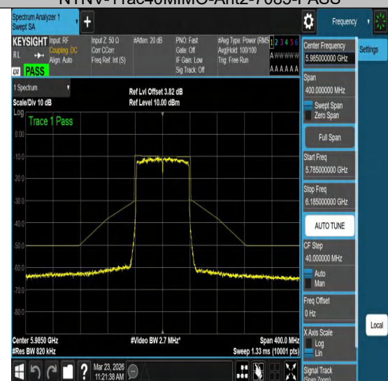
NTVN-11ac80MIMO-Ant2-5985-PASS
