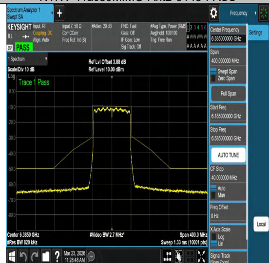
NTVN-11ac80MIMO-Ant2-6385-PASS
