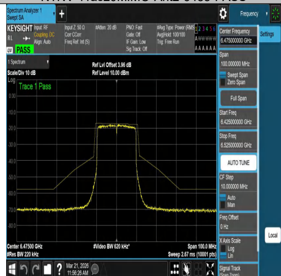
NTVN-11ac20MIMO-Ant2-6475-PASS
