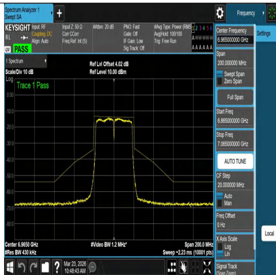
NTVN-11ac40MIMO-Ant1-6965-PASS
