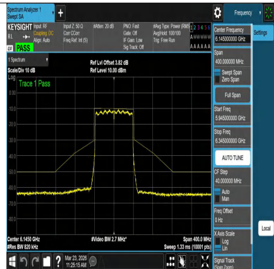
NTVN-11ac80MIMO-Ant2-6145-PASS
