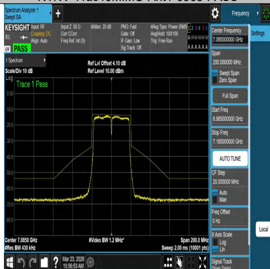
NTVN-11ac40MIMO-Ant1-7085-PASS
