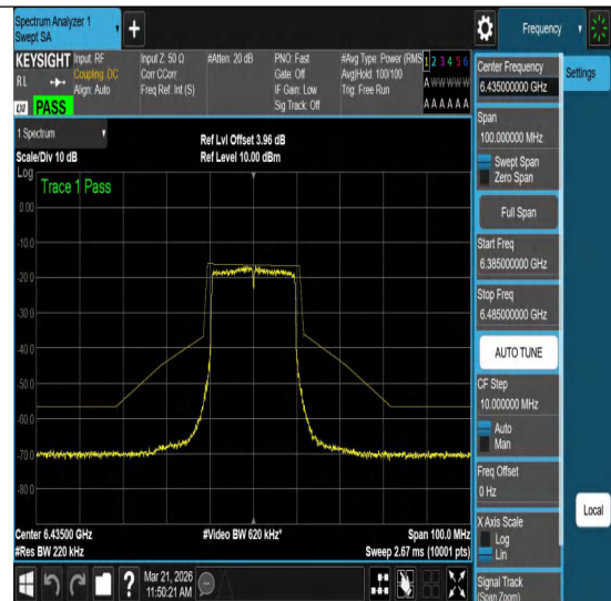
NTVN-11ac20MIMO-Ant2-6435-PASS
