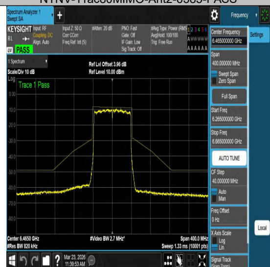
NTVN-11ac80MIMO-Ant2-6465-PASS
