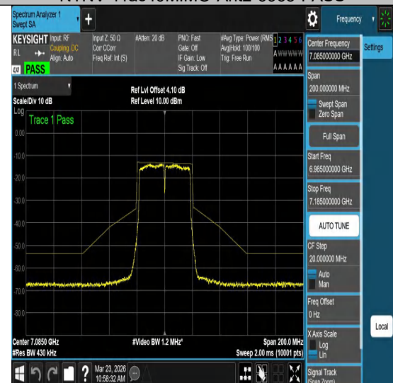
NTVN-11ac40MIMO-Ant2-7085-PASS
