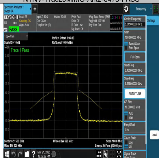
NTVN-11ac20MIMO-Ant2-6515-PASS
