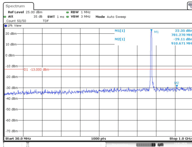
Band13-5MHz-QPSK-23205-25RB#0-Range1:30~1000MHz
