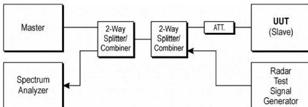
Figure 7-1. Test Setup
