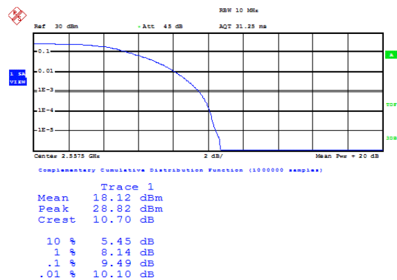
Band41-5MHz-QPSK-40265-25RB#0
