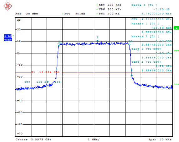
Band41-5MHz-QPSK-40265-25RB#0-4.51
