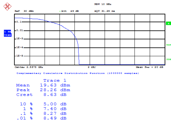
Band41-5MHz-QPSK-40265-1RB#0
