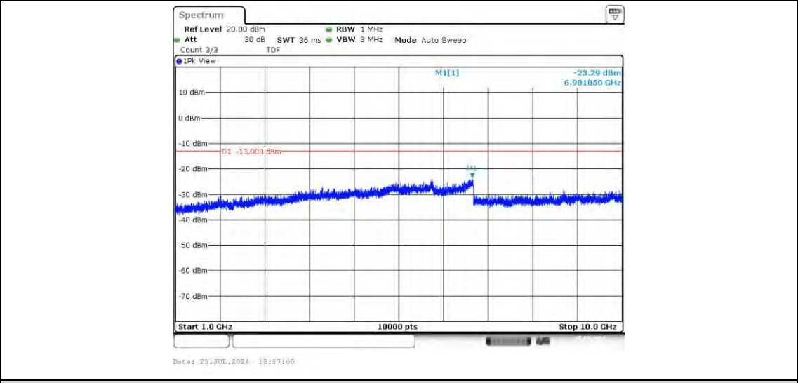
Band26-15MHz-QPSK-26865-75RB#0-Range1:30~1000MHz
