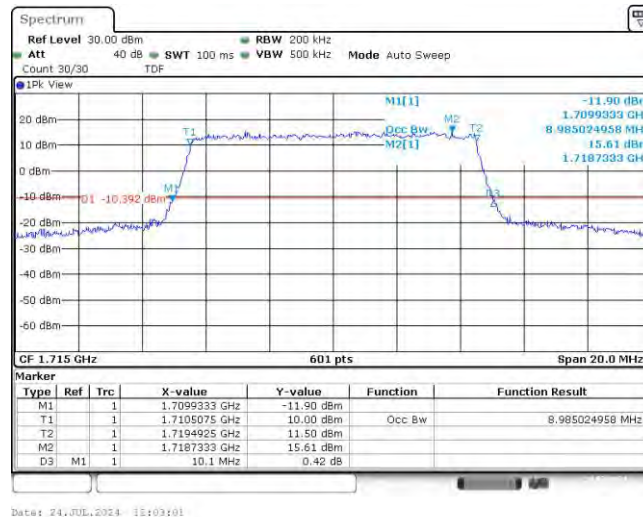
Band4-10MHz-16QAM-20175-50RB#0
