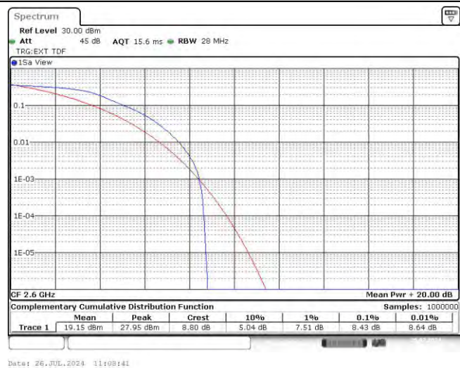
Band41-5MHz-QPSK-41565-25RB#0
