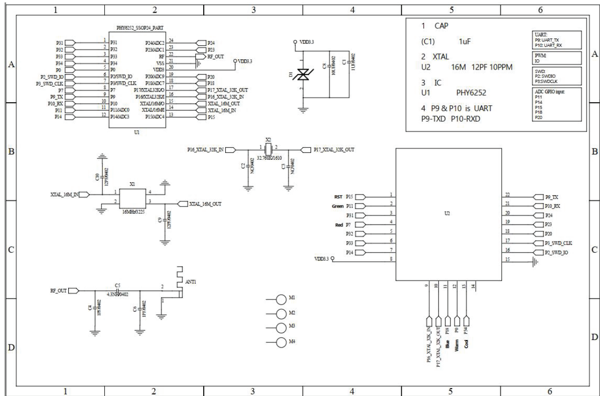
Figure 6 Module schematic
