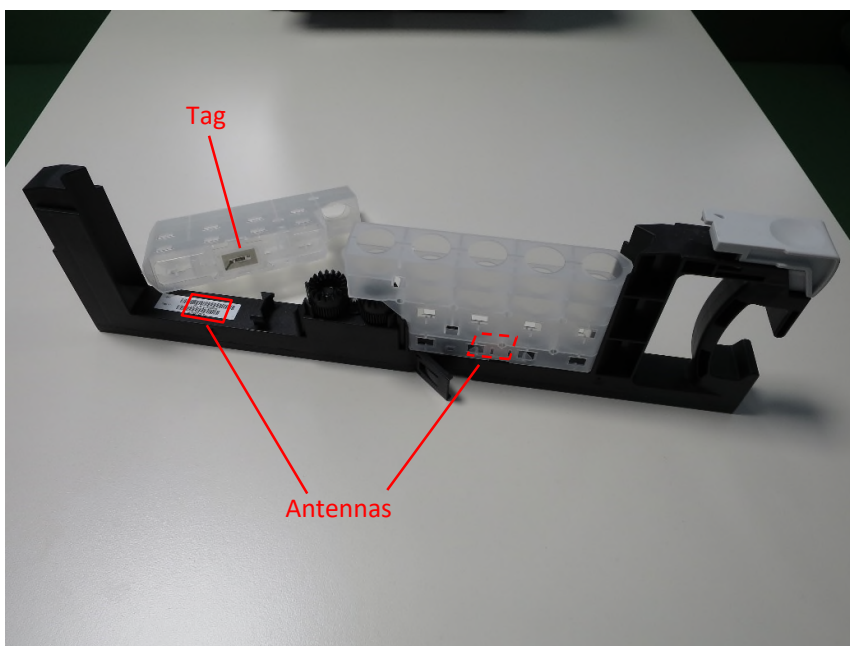
Fig. 2 - ARS Rack with Reagent Integrals
