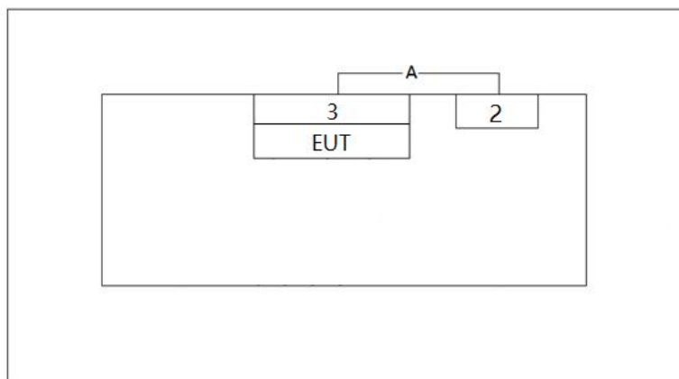
Connection Diagram for AC Conducted Emission Measurement
