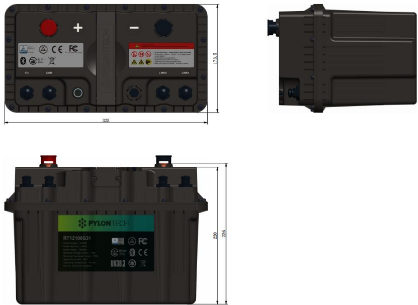
RT12100G31 Battery Dimension
