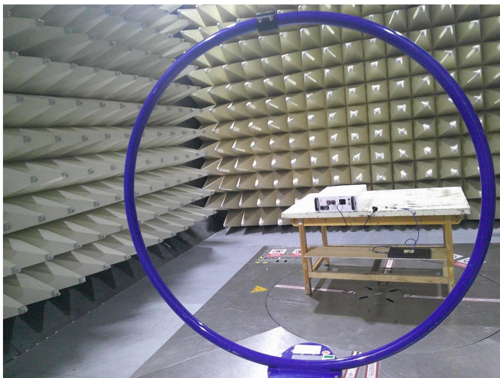
Photograph 2: Set-up photo for Radiated Emission, 9kHz - 30MHz
