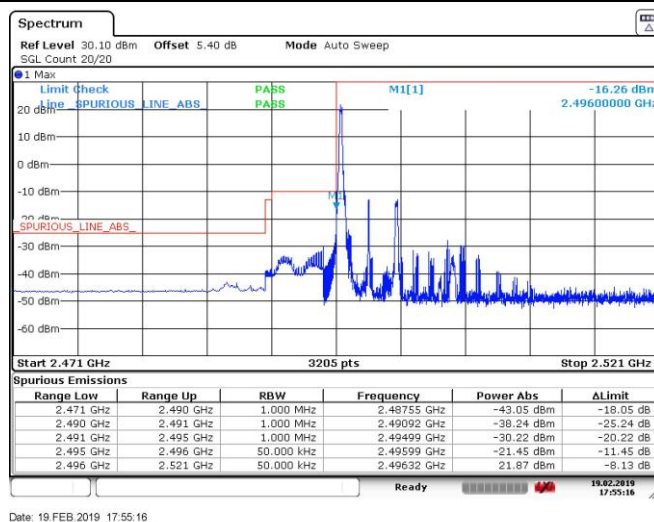
Band41_5MHz_QPSK_39675_25RB#0
