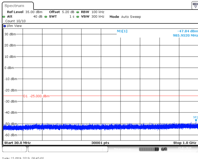
Band41_20MHz_16QAM_40620_1RB#0
