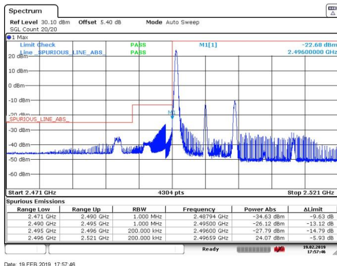
Band41_10MHz_16QAM_39700_50RB#0
