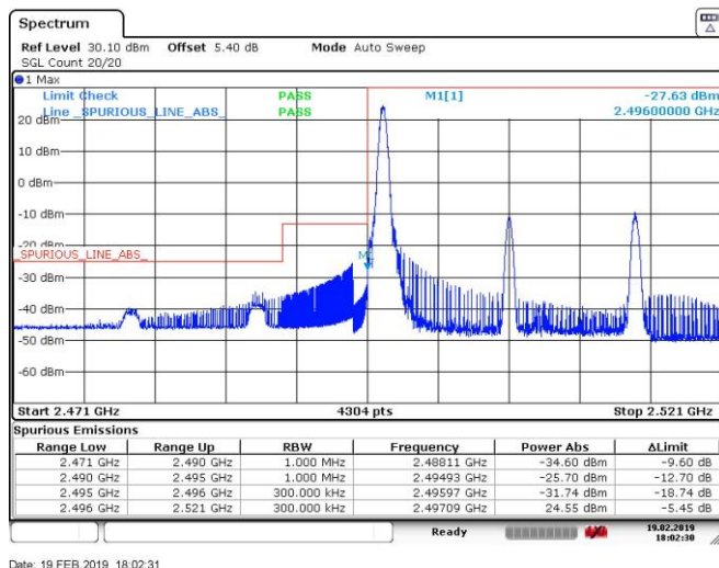
Band41_20MHz_16QAM_39750_100RB#0
