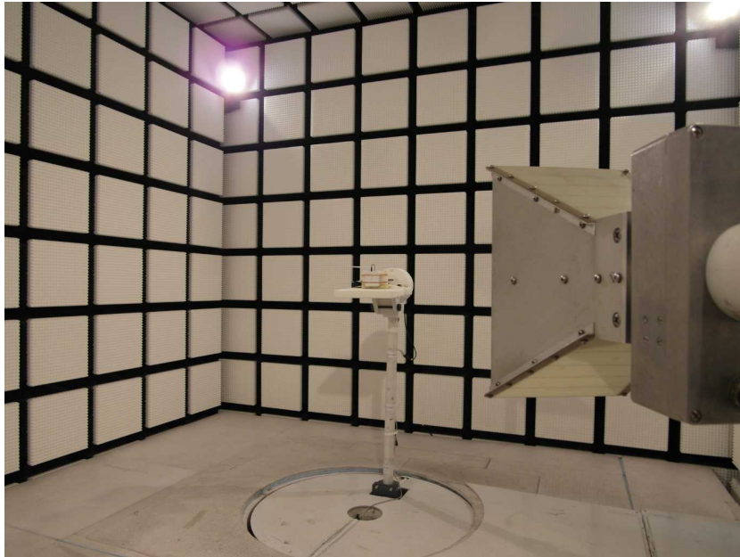
Photo 13: Chamber A up to 18 GHz
