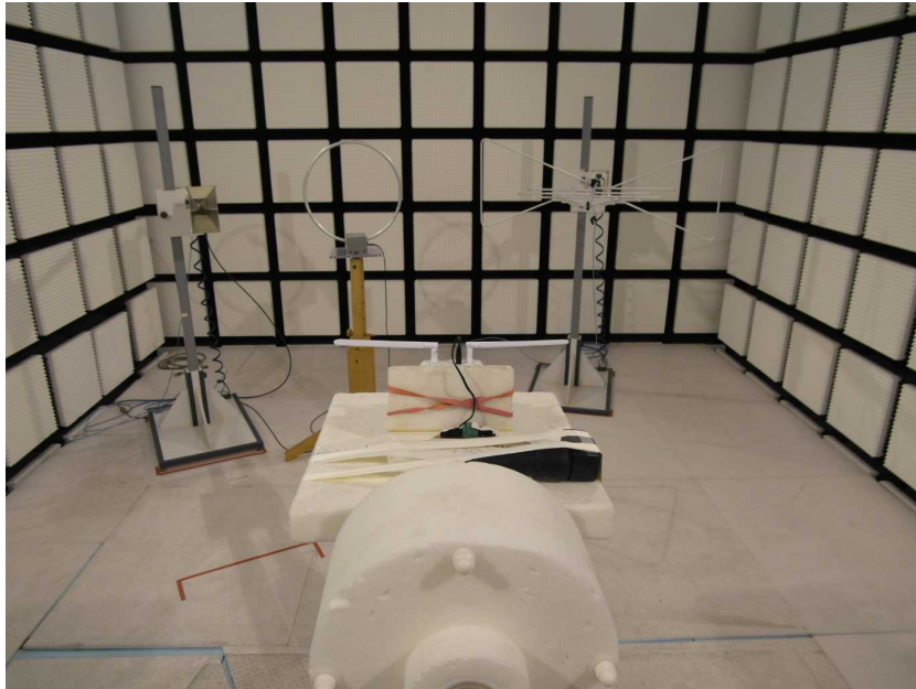
Photo 7: Chamber A up to 18 GHz
