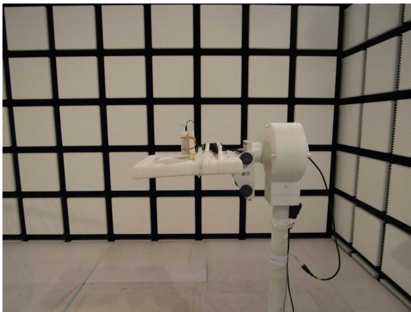
Photo 6: Chamber A up to 18 GHz
