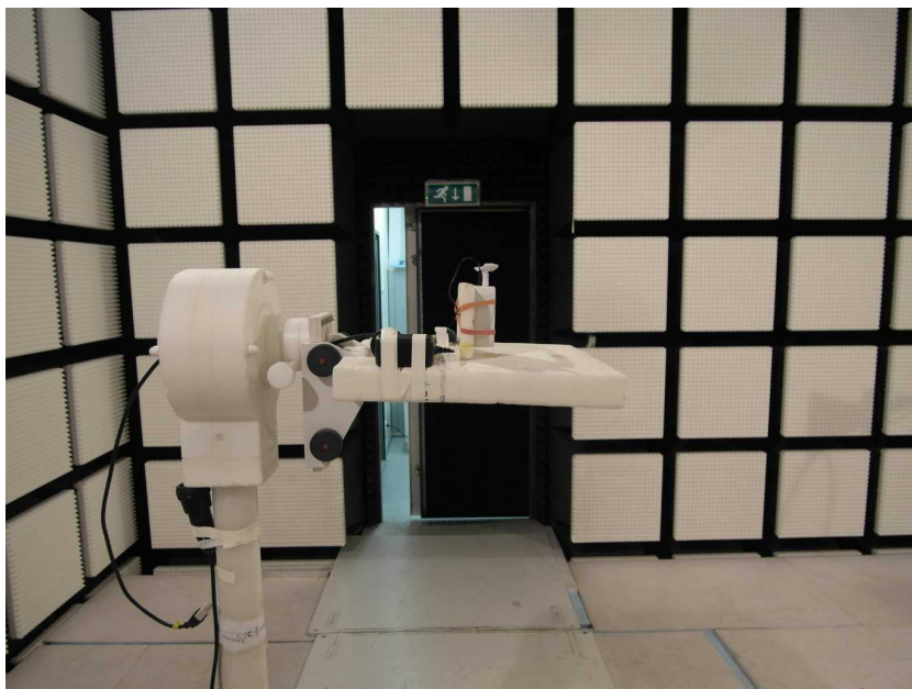
Photo 8: Chamber A up to 18 GHz
