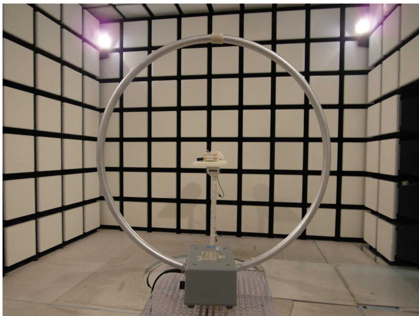
Photo 12: Chamber A up to 18 GHz
