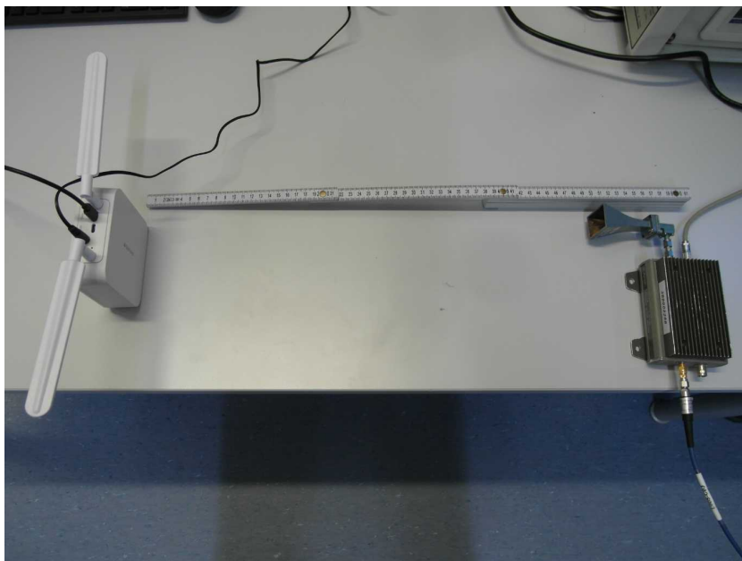
Photo 14: Up to 26 GHz
