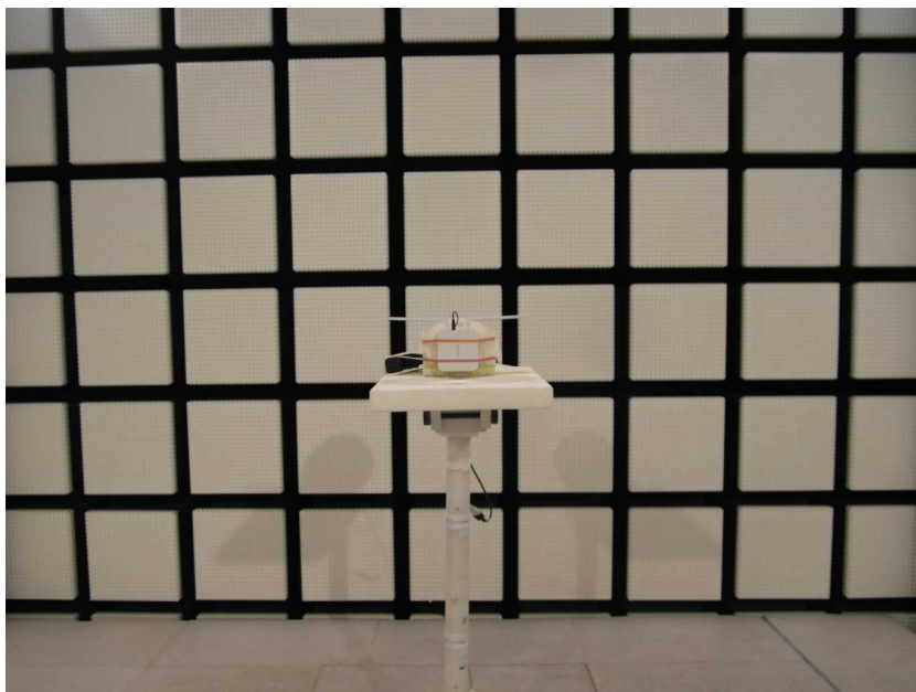
Photo 10: Chamber A up to 18 GHz
