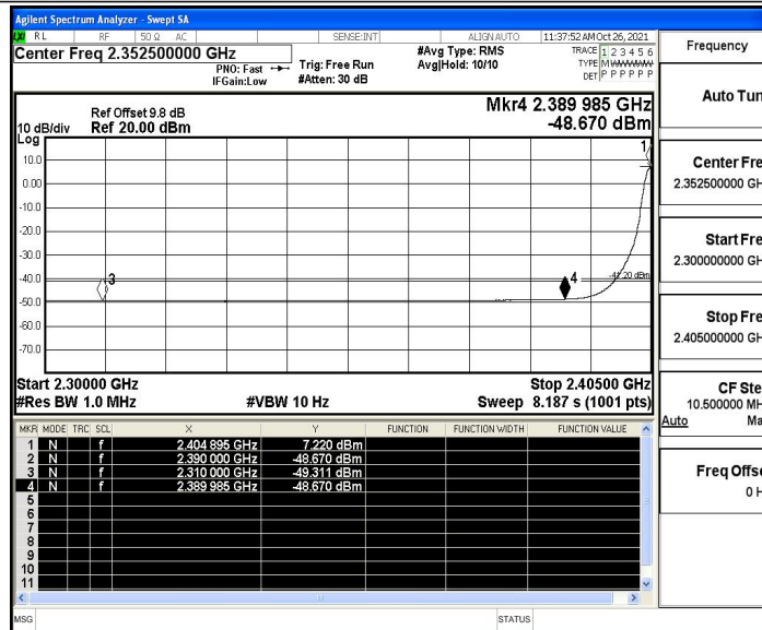
ZIGB_Ant1_Low_2405_Peak
