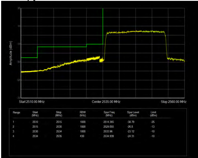
Band41(2535-2675) QPSK BW=20MHz Channel=41340 RB Size=100 Position=#0 Extended
