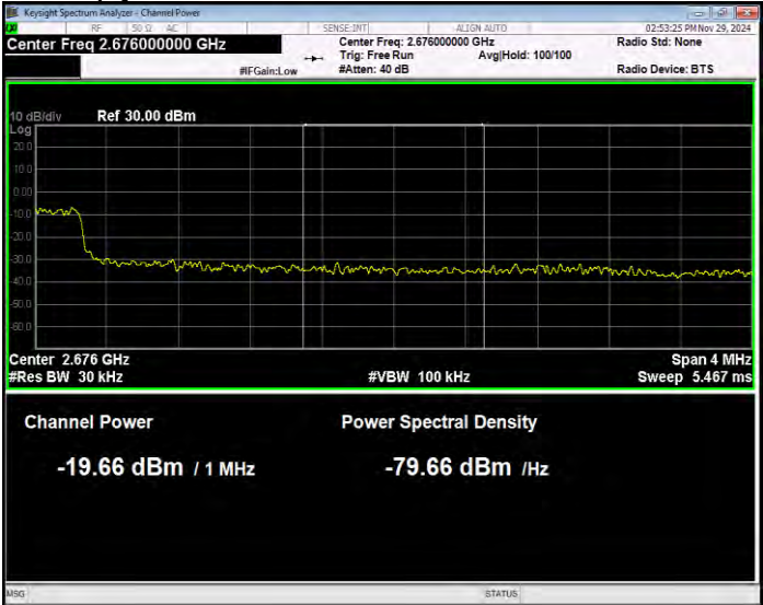
Band41(2535-2675) QPSK BW=15MHz Channel=41365 RB Size=75 Position=#0 Normal
