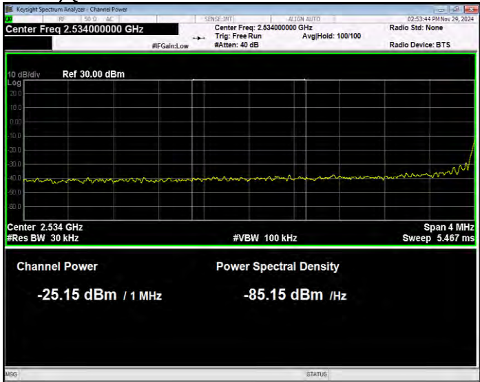
Band41(2535-2675) QPSK BW=20MHz Channel=40140 RB Size=100 Position=#0 Normal
