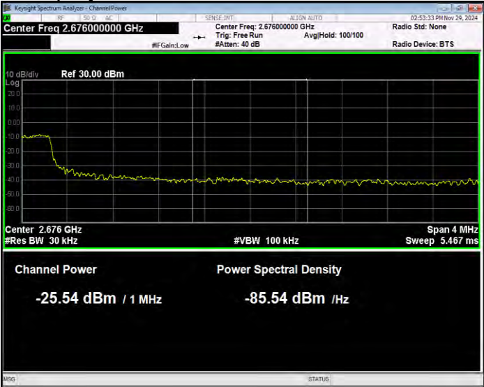
Band41(2535-2675) 16QAM BW=15MHz Channel=41365 RB Size=75 Position=#0 Normal
