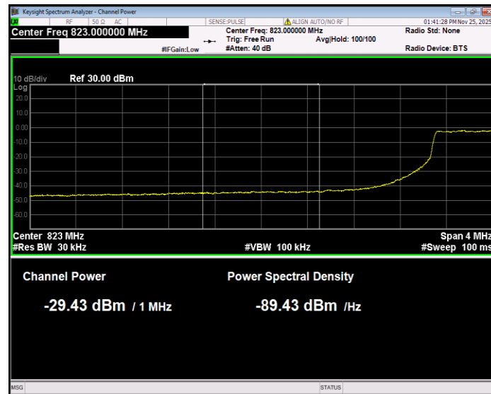
Band5 16QAM BW=10MHz Channel=20450 RB Size=50 Position=#0 Normal
