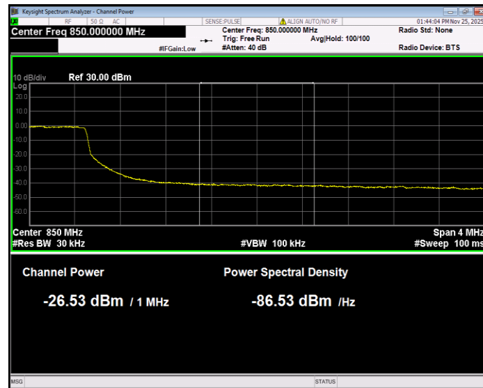
Band5 16QAM BW=10MHz Channel=20600 RB Size=50 Position=#0 Normal
