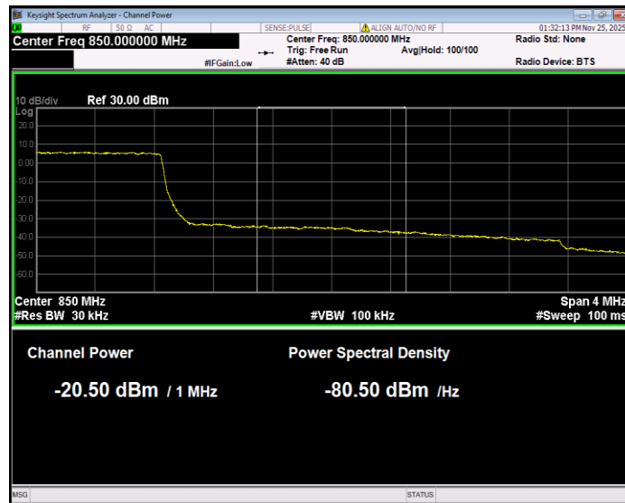
Band5 QPSK BW=3MHz Channel=20635 RB Size=15 Position=#0 Normal
