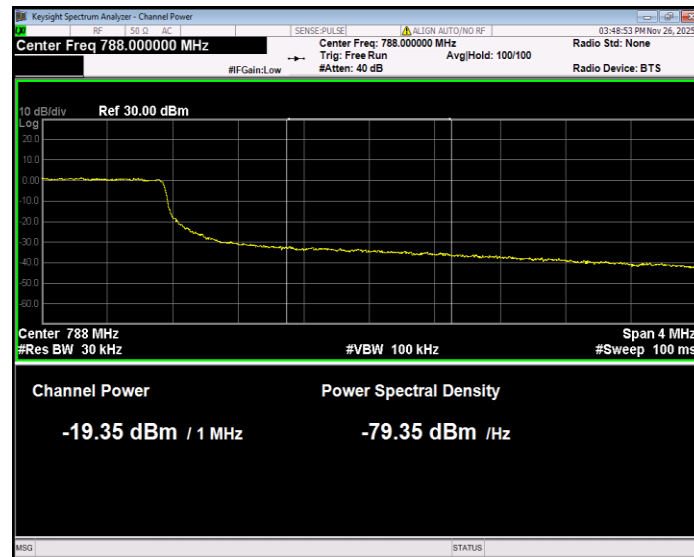
Band13 16QAM BW=5MHz Channel=23255 RB Size=25 Position=#0 Normal
