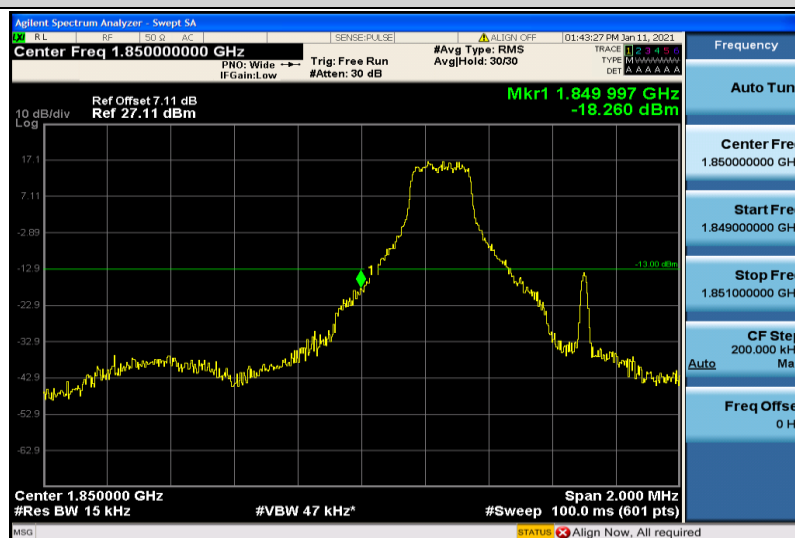
Band25-1.4MHz-16QAM-26047-1RB#0
