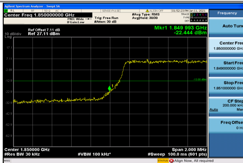
Band25-3MHz-16QAM-26055-15RB#0
