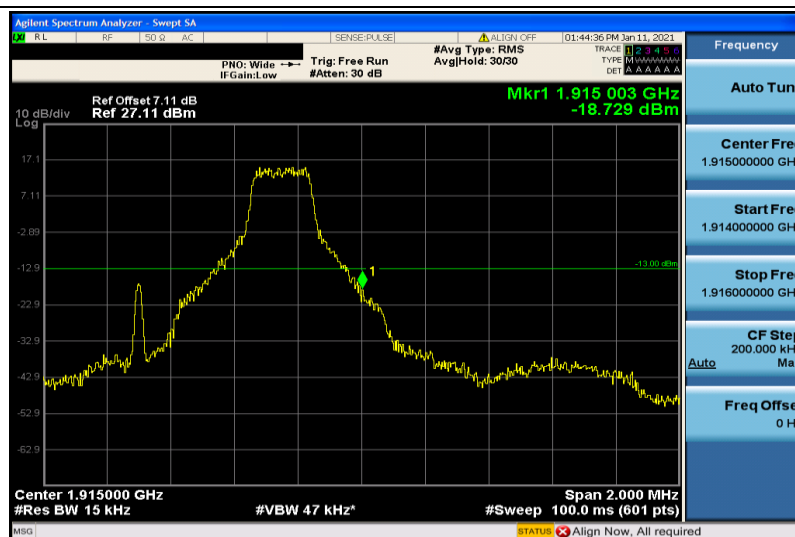
Band25-1.4MHz-QPSK-26683-1RB#5
