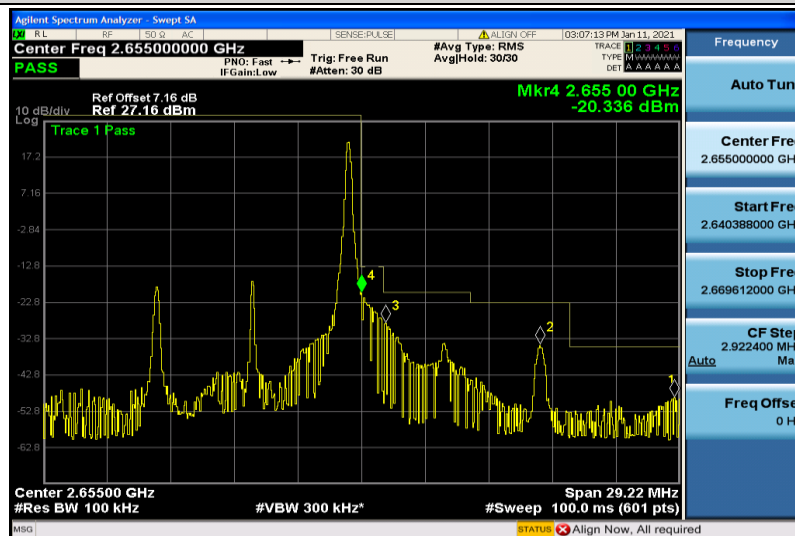
Band41-10MHz-16QAM-41190-1RB#49
