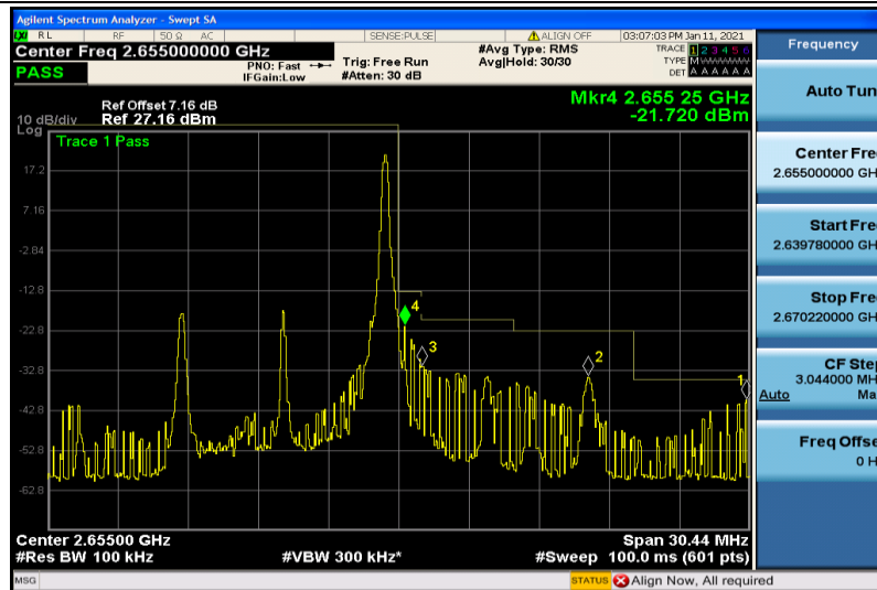
Band41-10MHz-QPSK-41190-1RB#49
