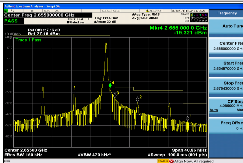
Band41-15MHz-QPSK-41165-1RB#74
