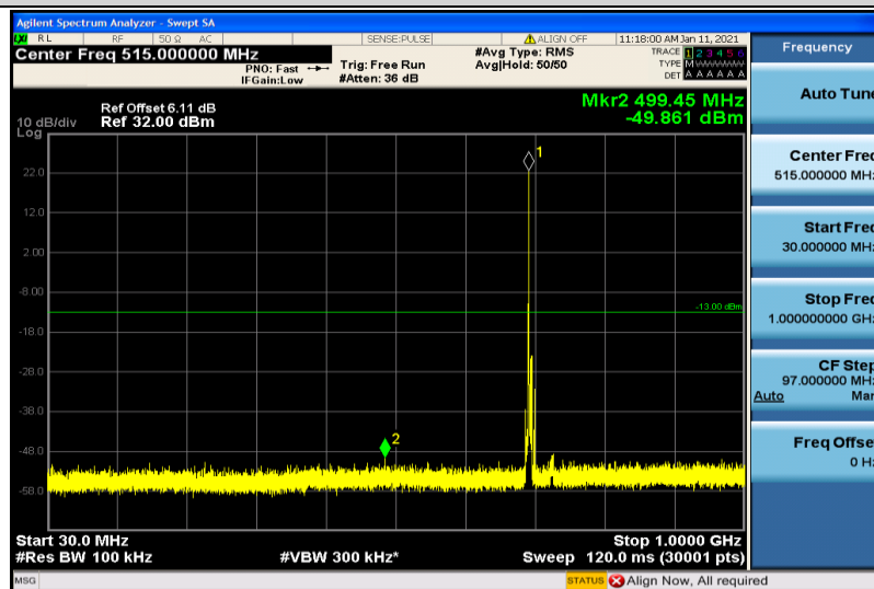
Band12-5MHz-QPSK-23035-1RB#0-30~1000MHz
