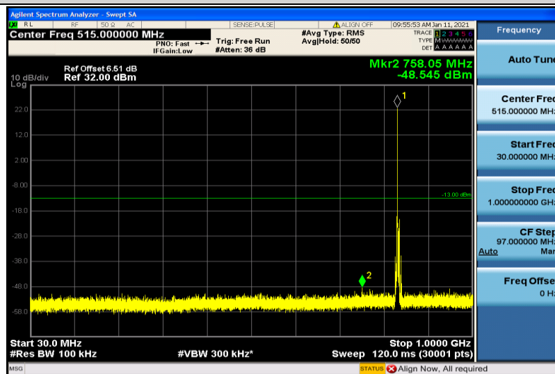
Band26-5MHz-16QAM-26915-1RB#0-30~1000MHz
