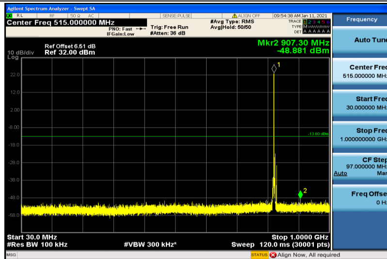
Band26-5MHz-16QAM-26815-1RB#0-30~1000MHz
