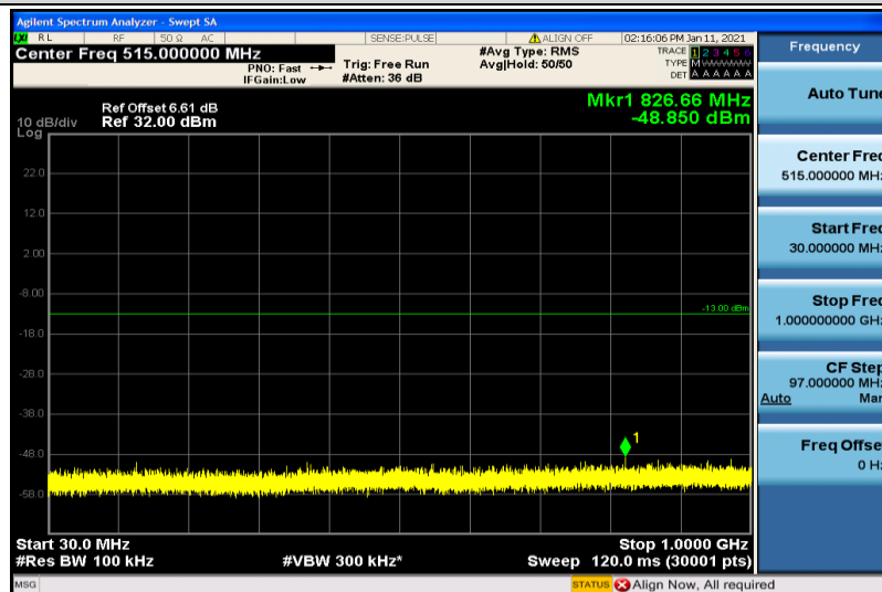
Band25-5MHz-16QAM-26665-1RB#0-30~1000MHz
