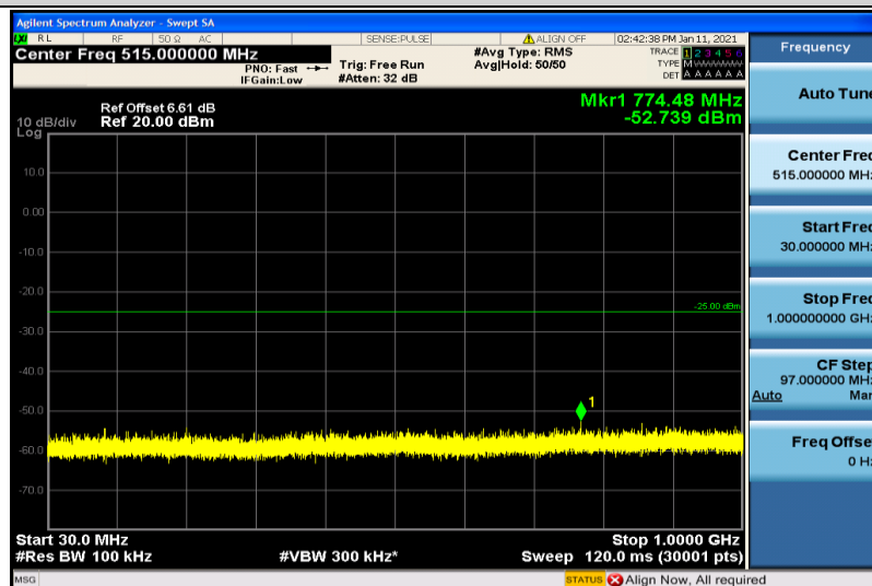
Band41-5MHz-16QAM-41215-1RB#0-30~1000MHz
