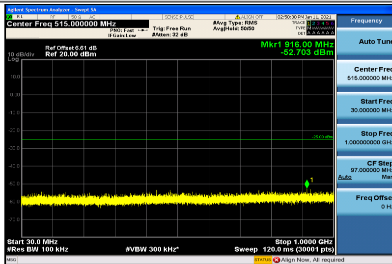
Band41-15MHz-16QAM-40315-1RB#0-30~1000MHz
