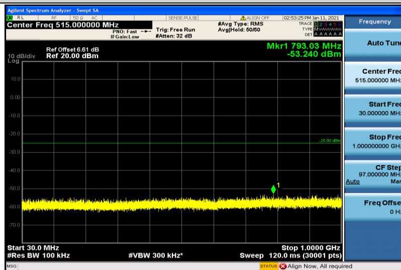
Band41-15MHz-16QAM-41165-1RB#0-30~1000MHz
