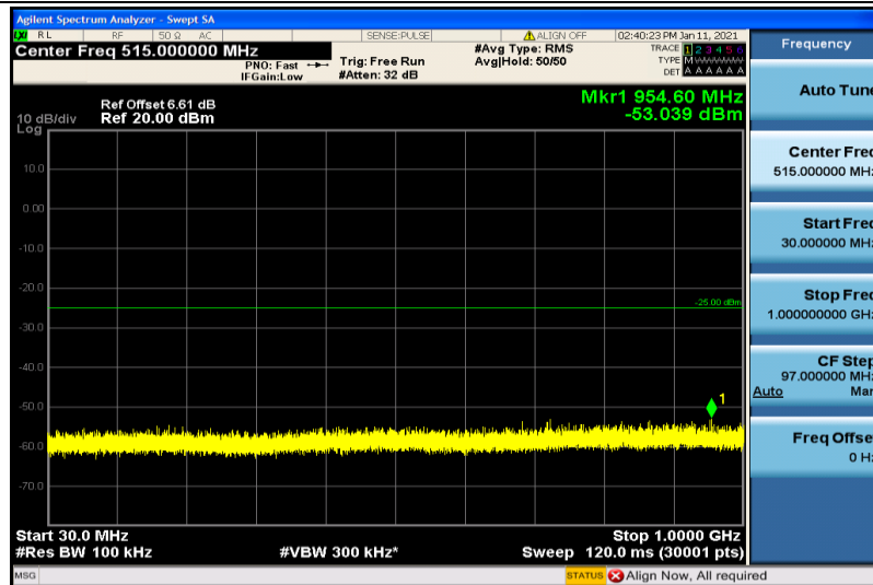
Band41-5MHz-16QAM-40740-1RB#0-30~1000MHz
