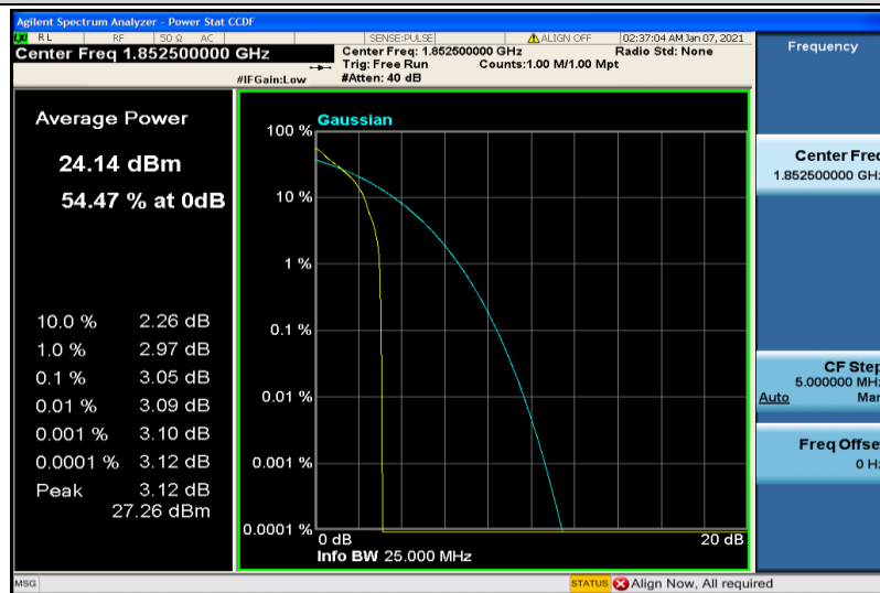
Band25-5MHz-QPSK-26065-1RB#0
