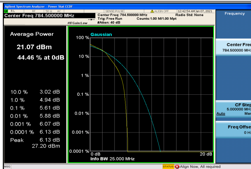
Band13-5MHz-16QAM-23255-25RB#0
