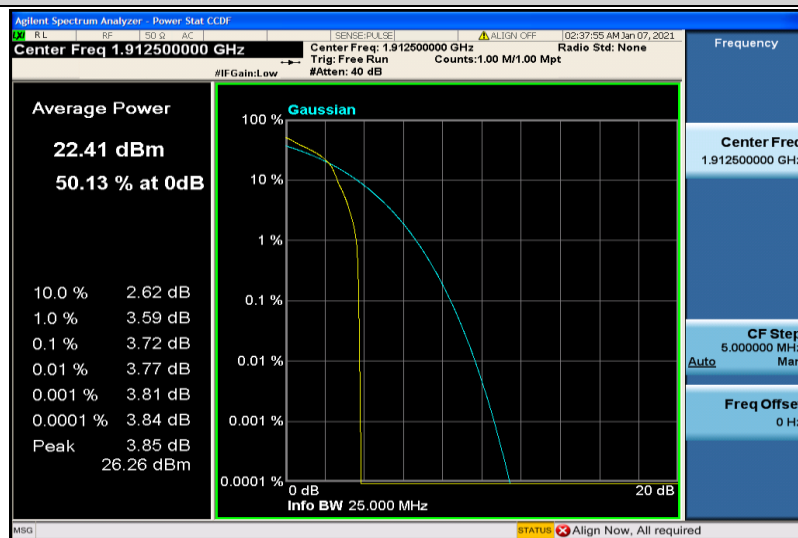
Band25-5MHz-16QAM-26665-1RB#0
