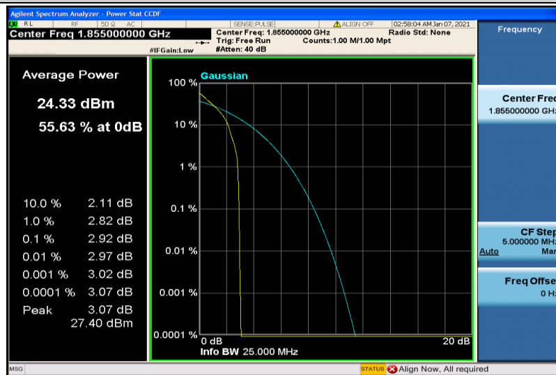
Band25-10MHz-QPSK-26090-1RB#0
