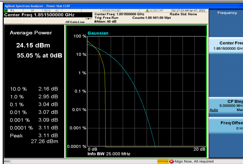
Band25-3MHz-QPSK-26055-1RB#0
