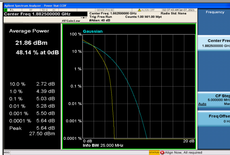
Band25-5MHz-16QAM-26365-25RB#0
