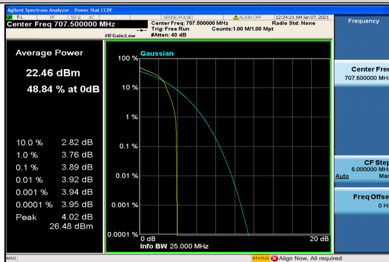
Band12-10MHz-16QAM-23095-1RB#0
