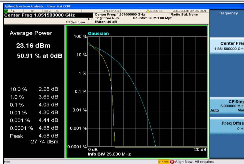
Band25-3MHz-QPSK-26055-15RB#0
