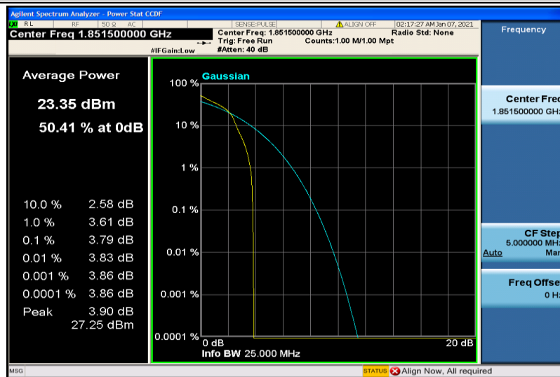
Band25-3MHz-16QAM-26055-1RB#0
