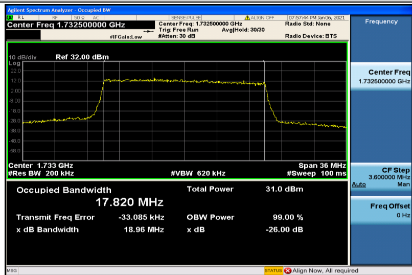
Band4-20MHz-QPSK-20175-100RB#0-17.820
