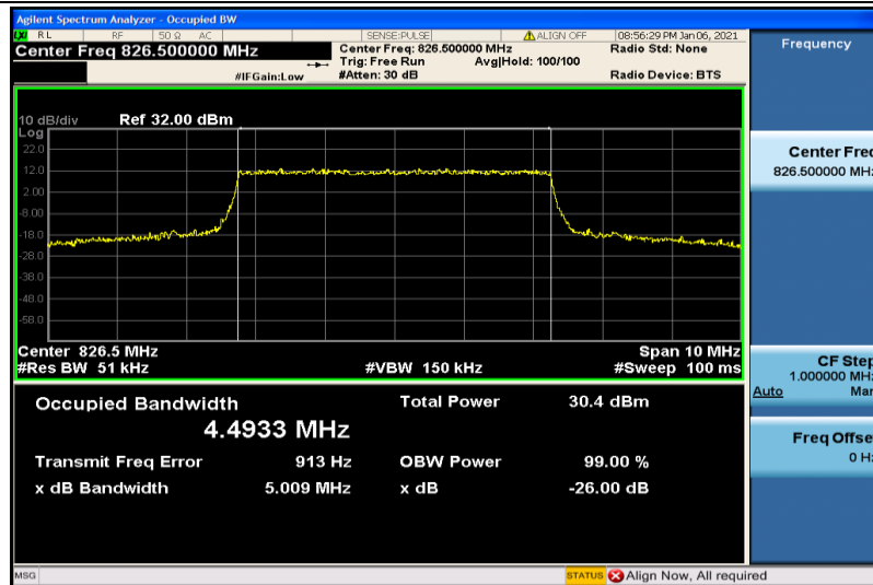
Band5-5MHz-QPSK-20425-25RB#0-4.4933
