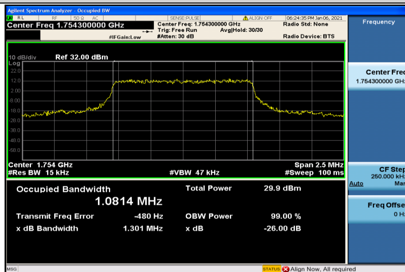
Band4-1.4MHz-QPSK-20393-6RB#0-1.0814
