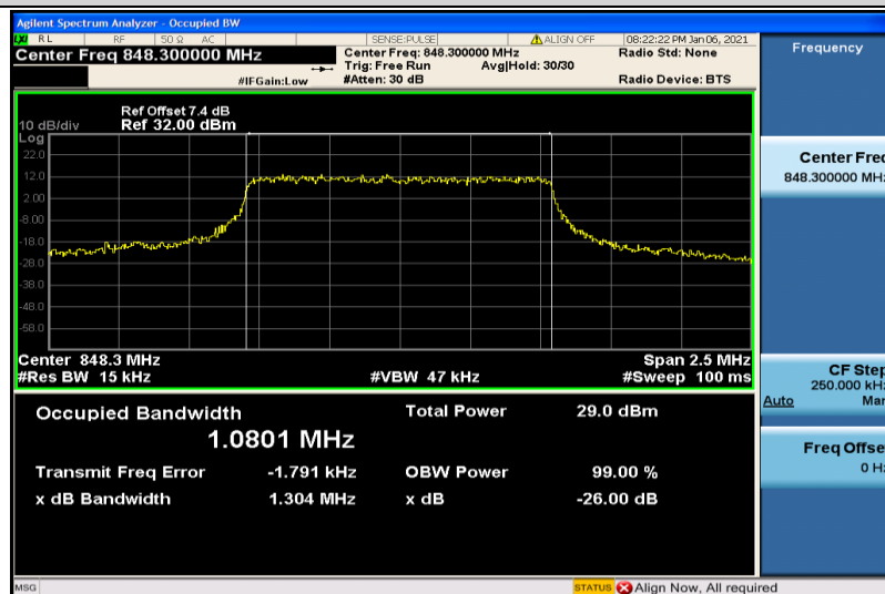
Band5-1.4MHz-QPSK-20643-6RB#0-1.0801
