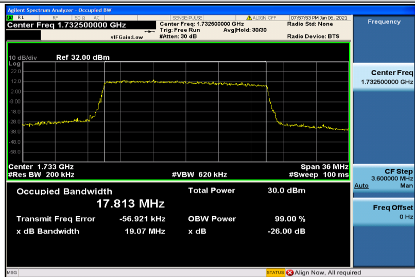
Band4-20MHz-16QAM-20175-100RB#0-17.813
