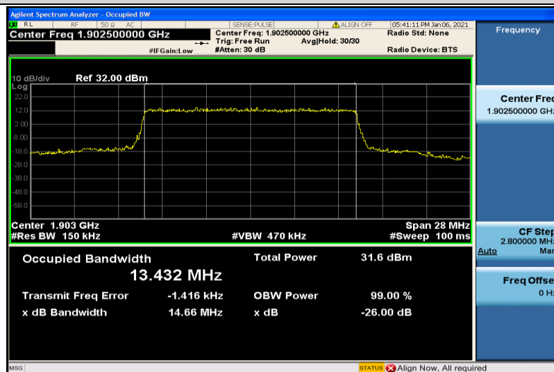
Band2-15MHz-QPSK-19125-75RB#0-13.432
