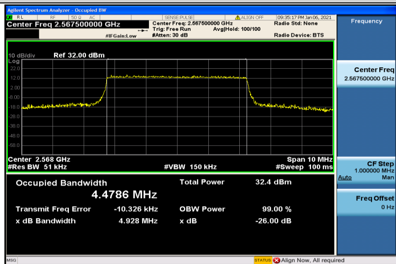
Band7-5MHz-QPSK-21425-25RB#0-4.4786
