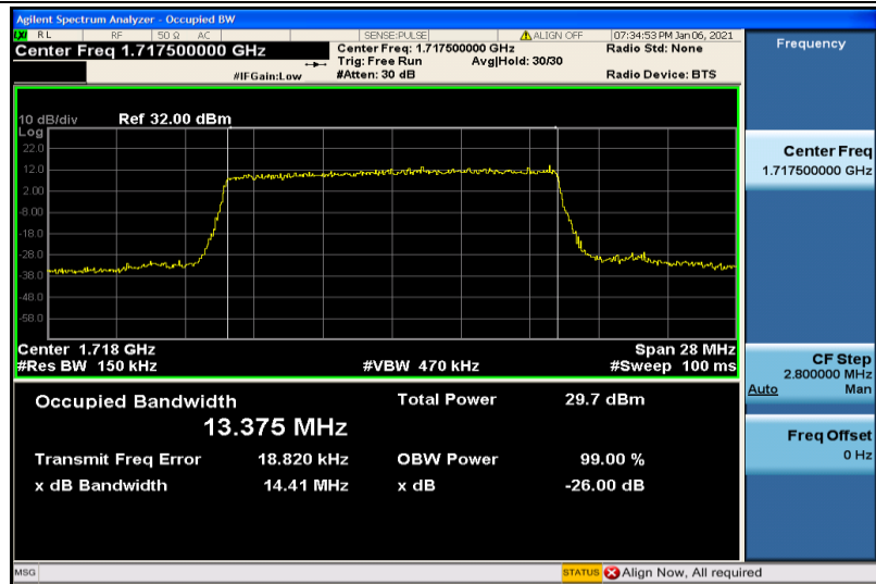
Band4-15MHz-16QAM-20025-75RB#0-13.375
