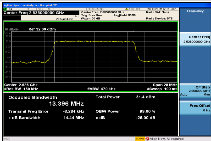
Band7-15MHz-16QAM-21100-75RB#0-13.396
