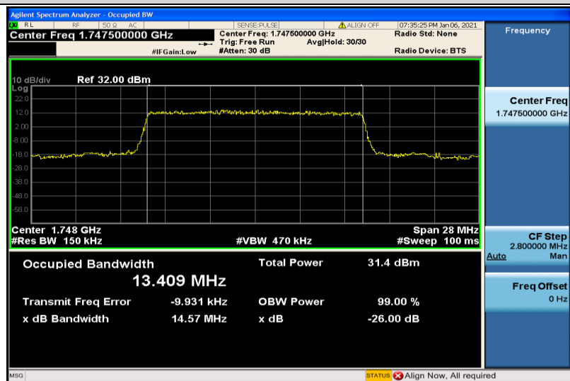
Band4-15MHz-QPSK-20325-75RB#0-13.409
