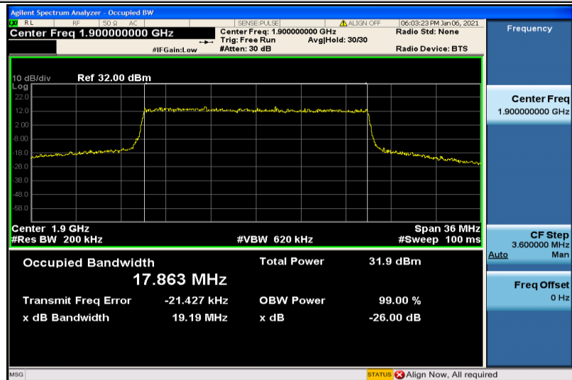
Band2-20MHz-QPSK-19100-100RB#0-17.863
