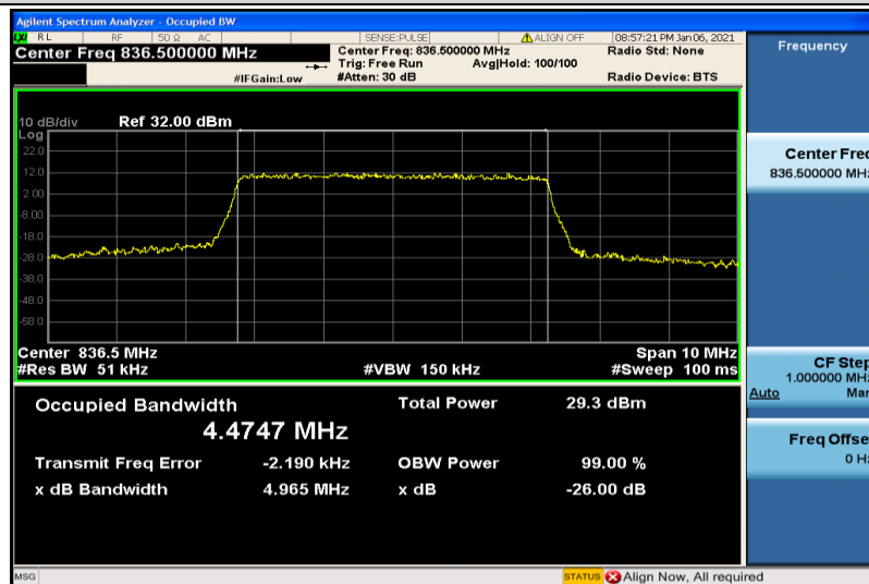
Band5-5MHz-16QAM-20525-25RB#0-4.4747
