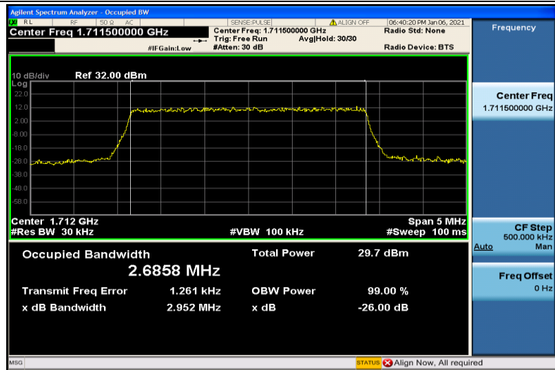
Band4-3MHz-QPSK-19965-15RB#0-2.6858
