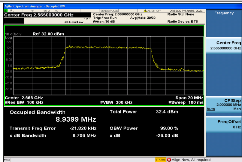
Band7-10MHz-QPSK-21400-50RB#0-8.9399
