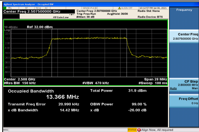
Band7-15MHz-QPSK-20825-75RB#0-13.366
