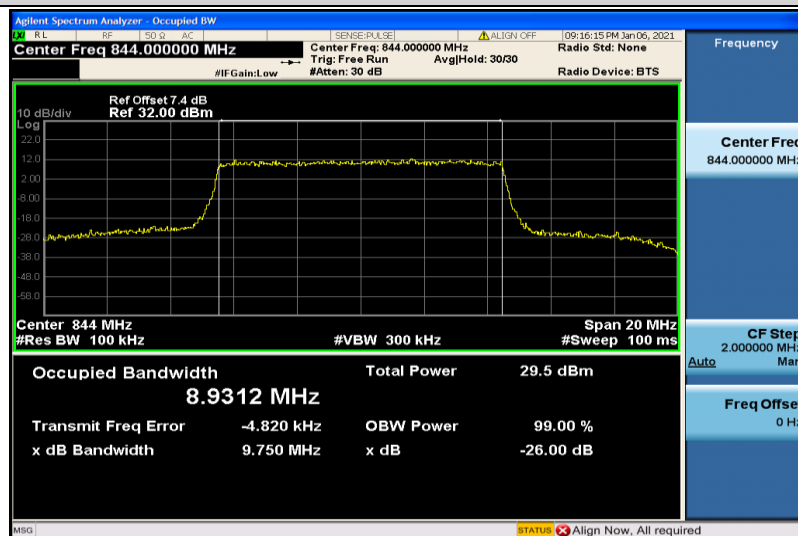
Band5-10MHz-16QAM-20600-50RB#0-8.9312
