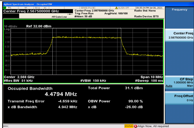
Band7-5MHz-16QAM-21425-25RB#0-4.4794
