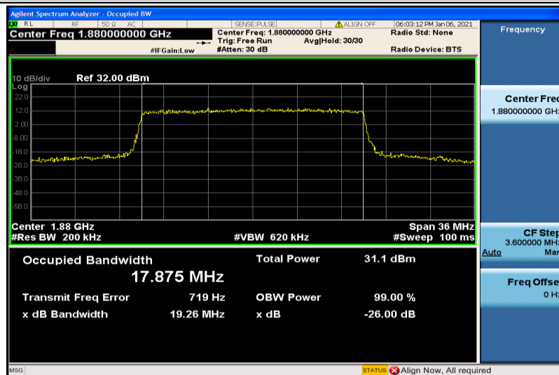
Band2-20MHz-16QAM-18900-100RB#0-17.875
