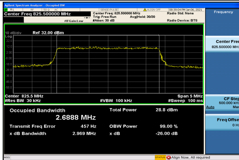
Band5-3MHz-16QAM-20415-15RB#0-2.6888
