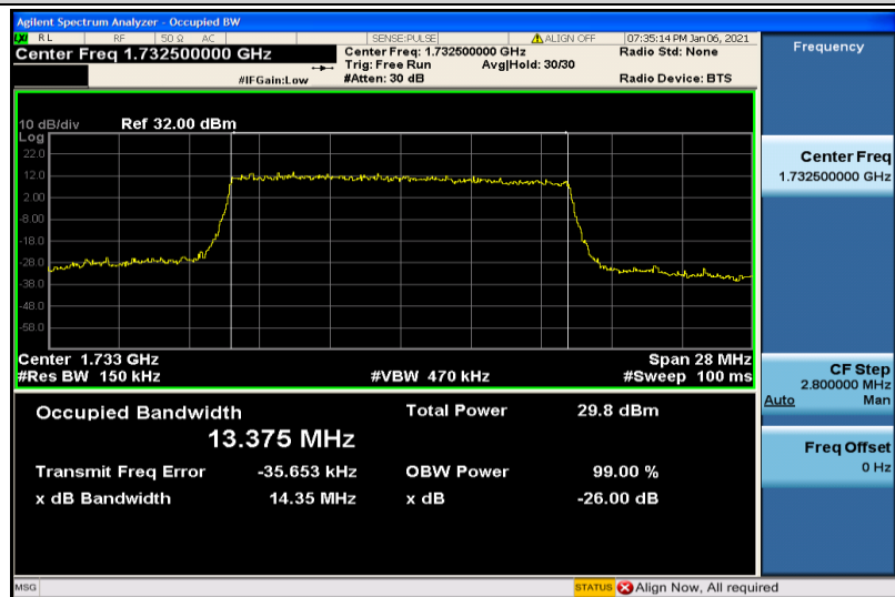
Band4-15MHz-16QAM-20175-75RB#0-13.375
