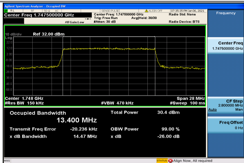
Band4-15MHz-16QAM-20325-75RB#0-13.400
