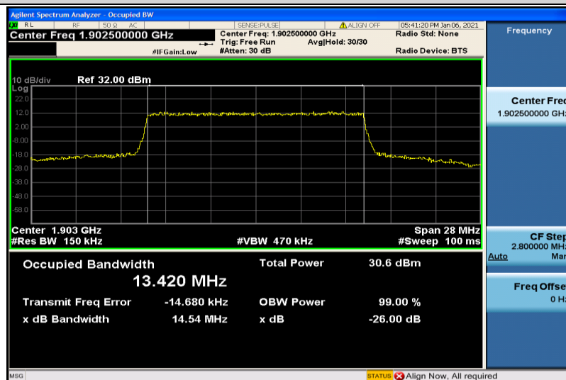
Band2-15MHz-16QAM-19125-75RB#0-13.420
