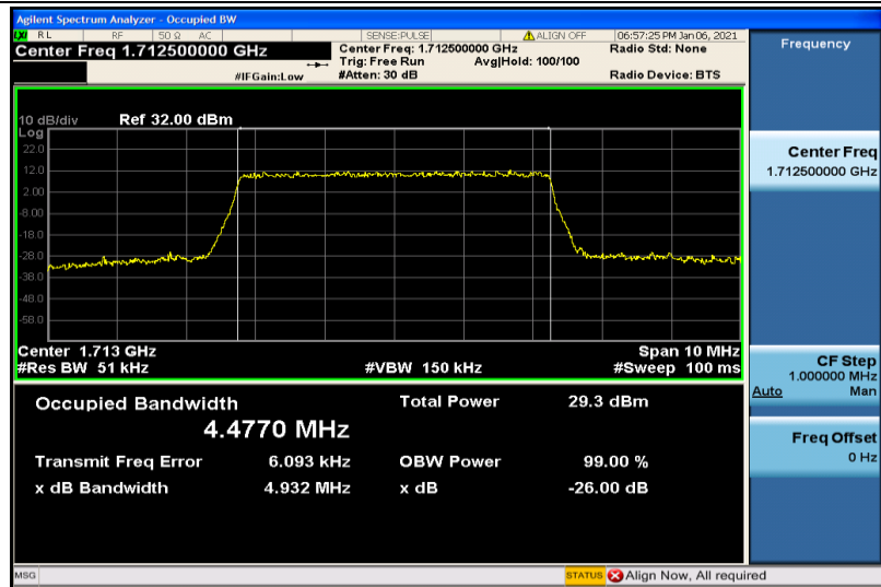
Band4-5MHz-16QAM-19975-25RB#0-4.4770
