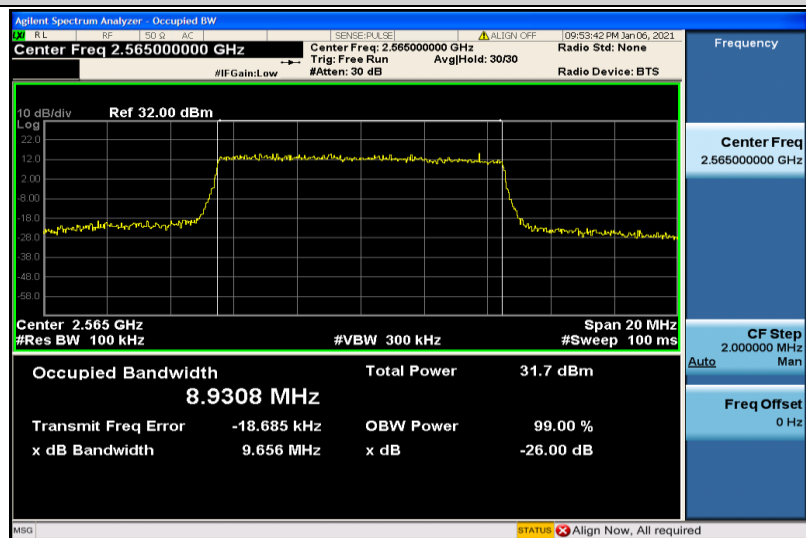
Band7-10MHz-16QAM-21400-50RB#0-8.9308
