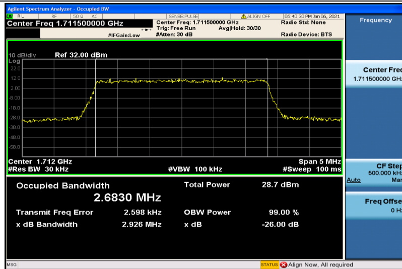
Band4-3MHz-16QAM-19965-15RB#0-2.6830
