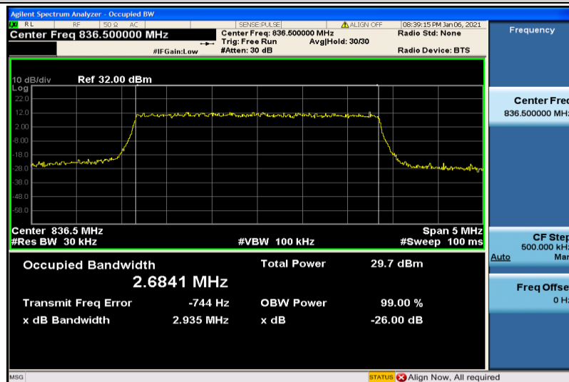
Band5-3MHz-QPSK-20525-15RB#0-2.6841
