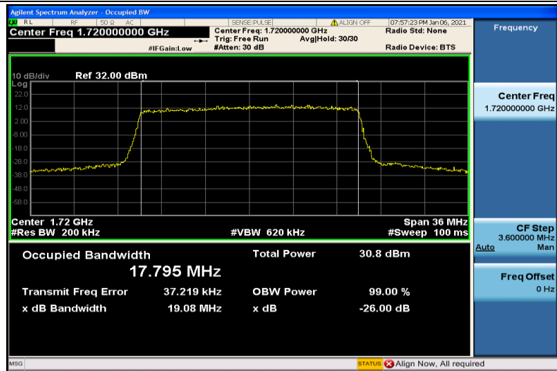
Band4-20MHz-QPSK-20050-100RB#0-17.795
