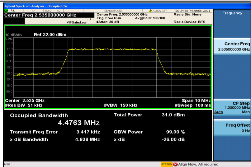
Band7-5MHz-16QAM-21100-25RB#0-4.4763
