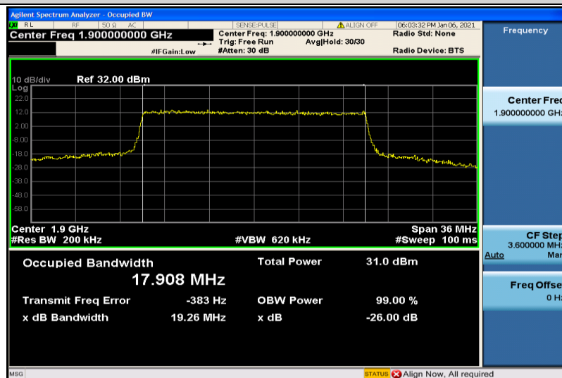
Band2-20MHz-16QAM-19100-100RB#0-17.908
