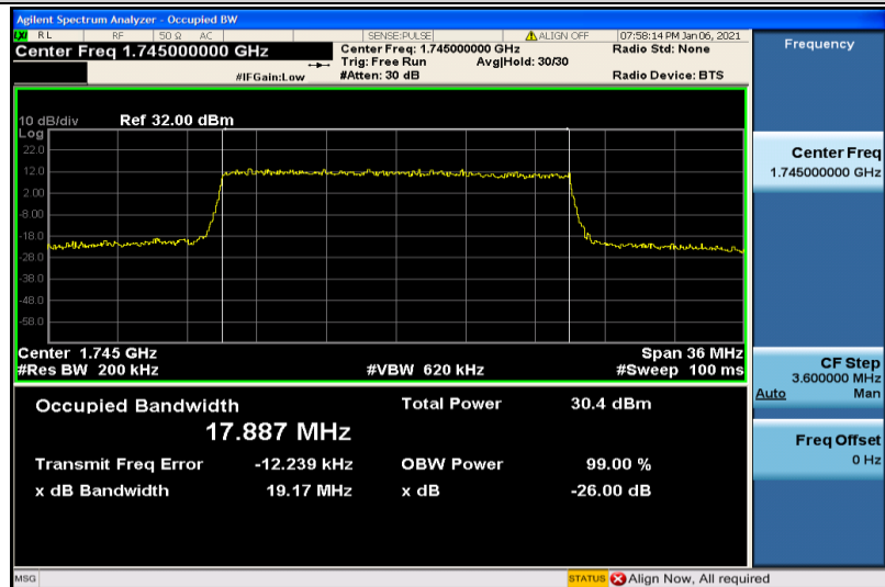
Band4-20MHz-16QAM-20300-100RB#0-17.887
