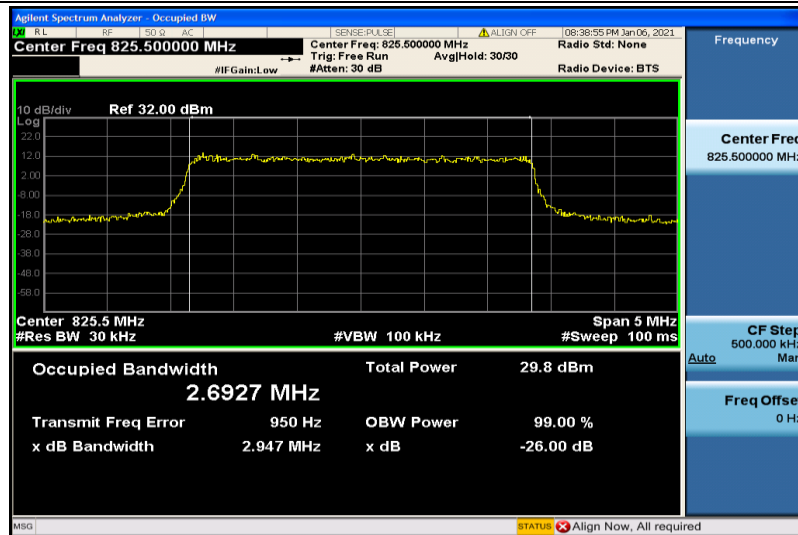
Band5-3MHz-QPSK-20415-15RB#0-2.6927
