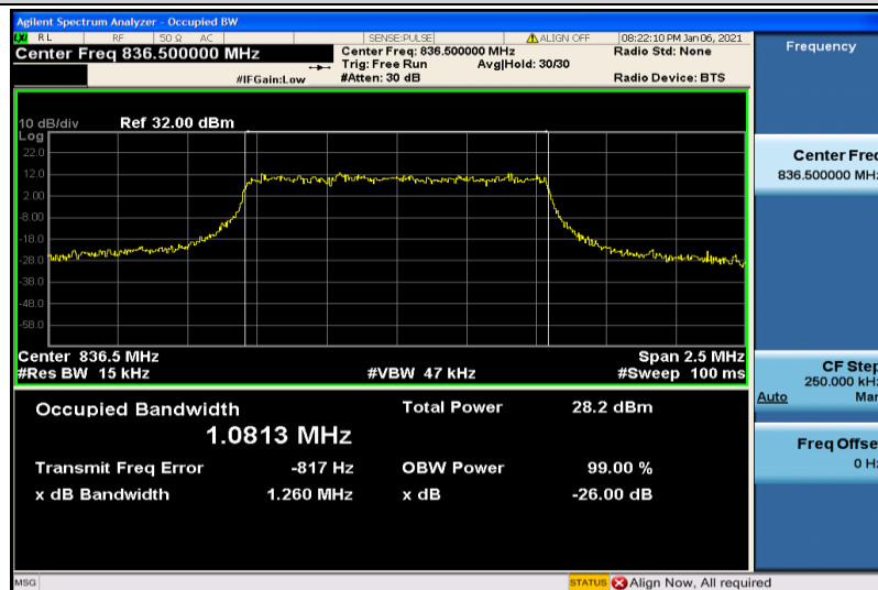
Band5-1.4MHz-16QAM-20525-6RB#0-1.0813
