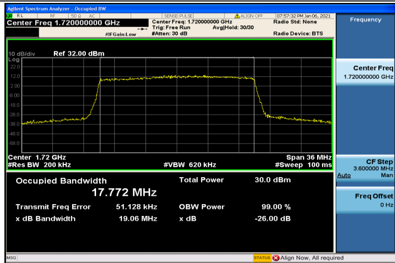
Band4-20MHz-16QAM-20050-100RB#0-17.772
