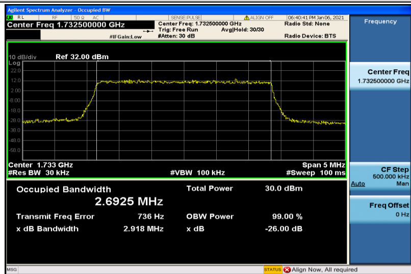
Band4-3MHz-QPSK-20175-15RB#0-2.6925
