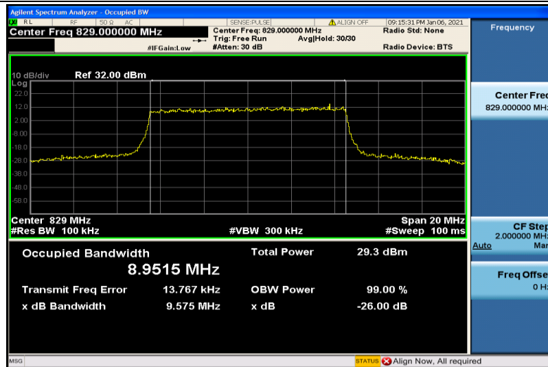
Band5-10MHz-16QAM-20450-50RB#0-8.9515
