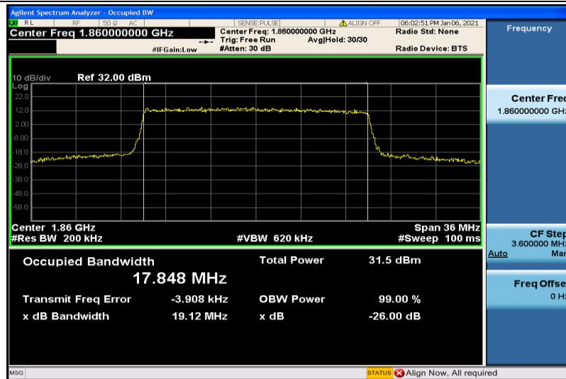
Band2-20MHz-16QAM-18700-100RB#0-17.848
