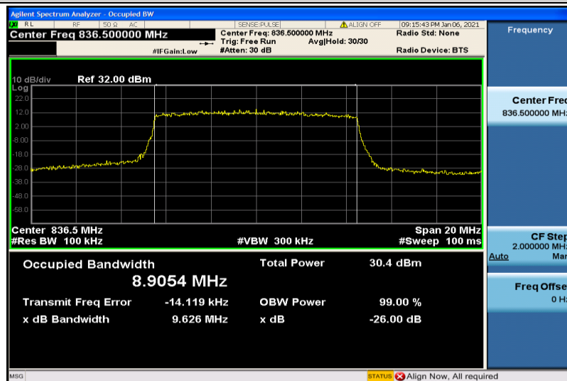
Band5-10MHz-QPSK-20525-50RB#0-8.9054
