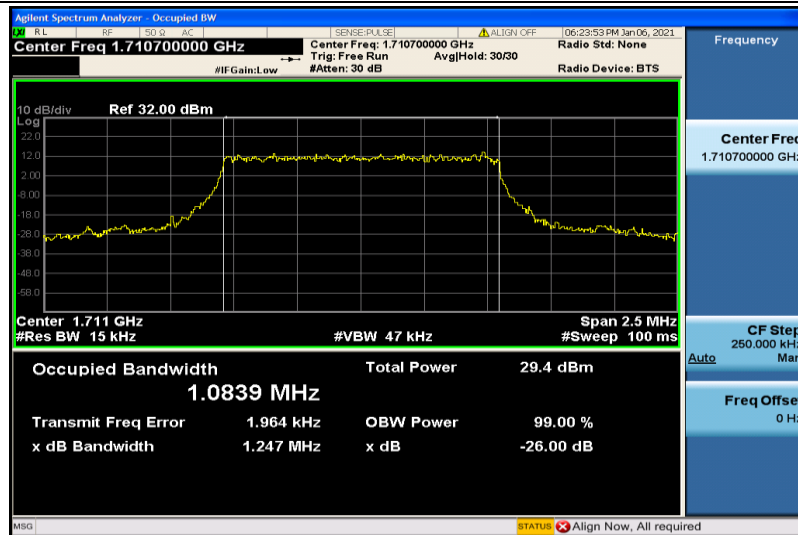
Band4-1.4MHz-QPSK-19957-6RB#0-1.0839
