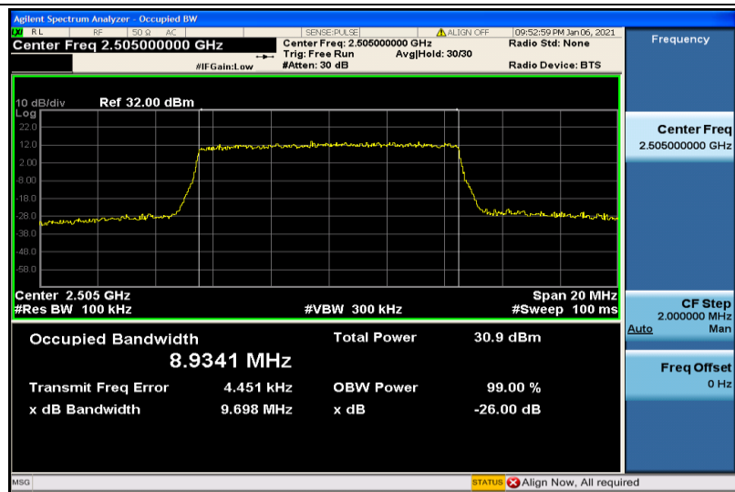
Band7-10MHz-16QAM-20800-50RB#0-8.9341
