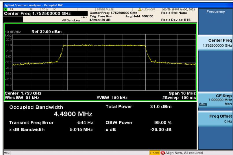
Band4-5MHz-QPSK-20375-25RB#0-4.4900
