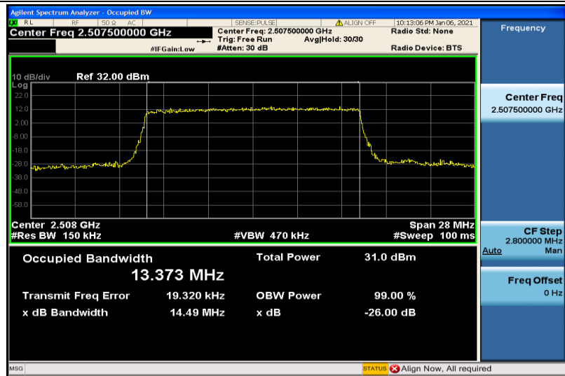
Band7-15MHz-16QAM-20825-75RB#0-13.373
