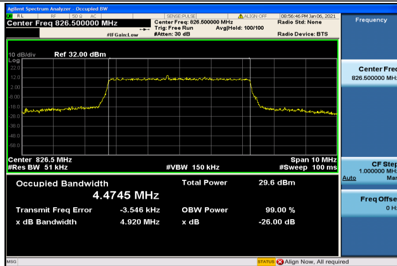
Band5-5MHz-16QAM-20425-25RB#0-4.4745
