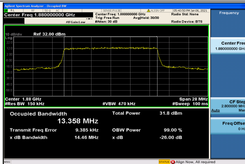
Band2-15MHz-QPSK-18900-75RB#0-13.358
