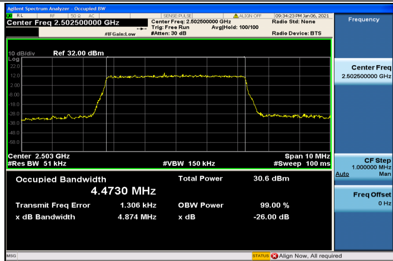
Band7-5MHz-16QAM-20775-25RB#0-4.4730
