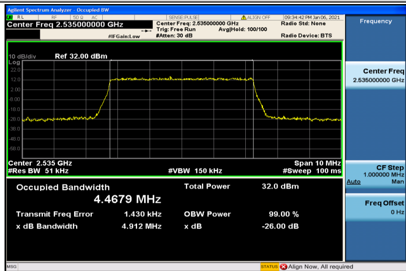
Band7-5MHz-QPSK-21100-25RB#0-4.4679
