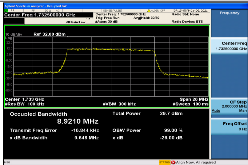
Band4-10MHz-16QAM-20175-50RB#0-8.9210
