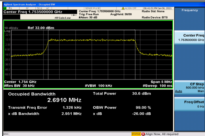
Band4-3MHz-QPSK-20385-15RB#0-2.6910
