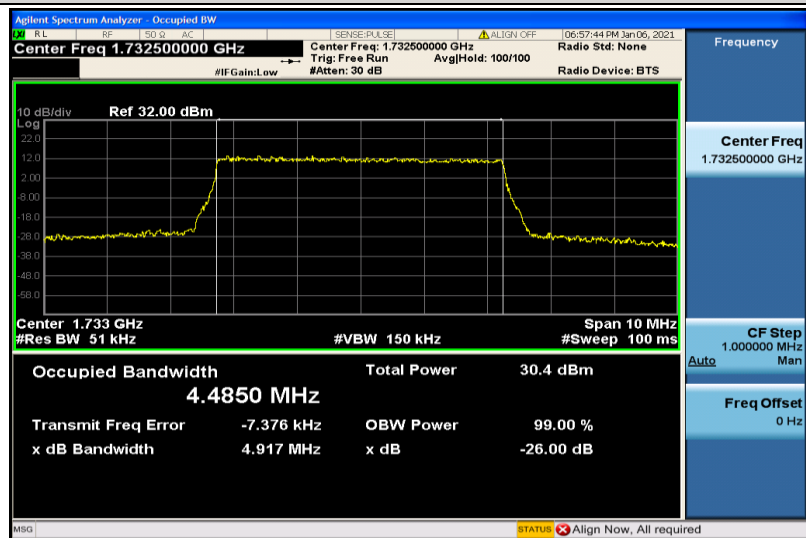
Band4-5MHz-QPSK-20175-25RB#0-4.4850
