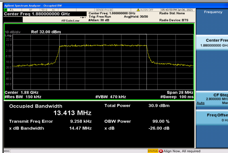
Band2-15MHz-16QAM-18900-75RB#0-13.413
