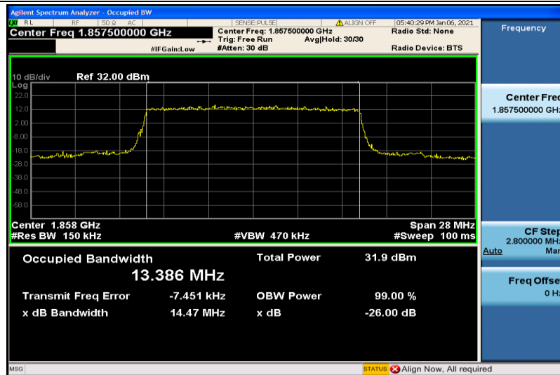
Band2-15MHz-QPSK-18675-75RB#0-13.386
