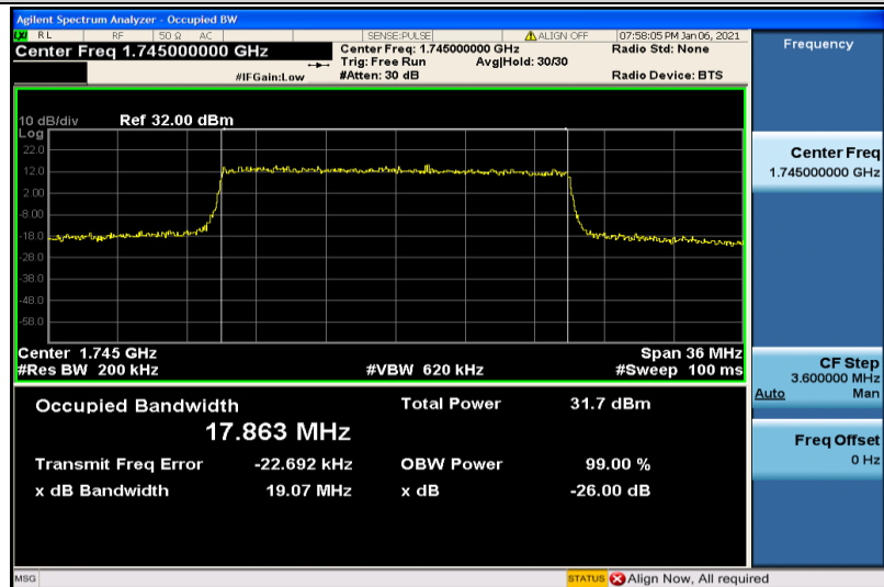
Band4-20MHz-QPSK-20300-100RB#0-17.863
