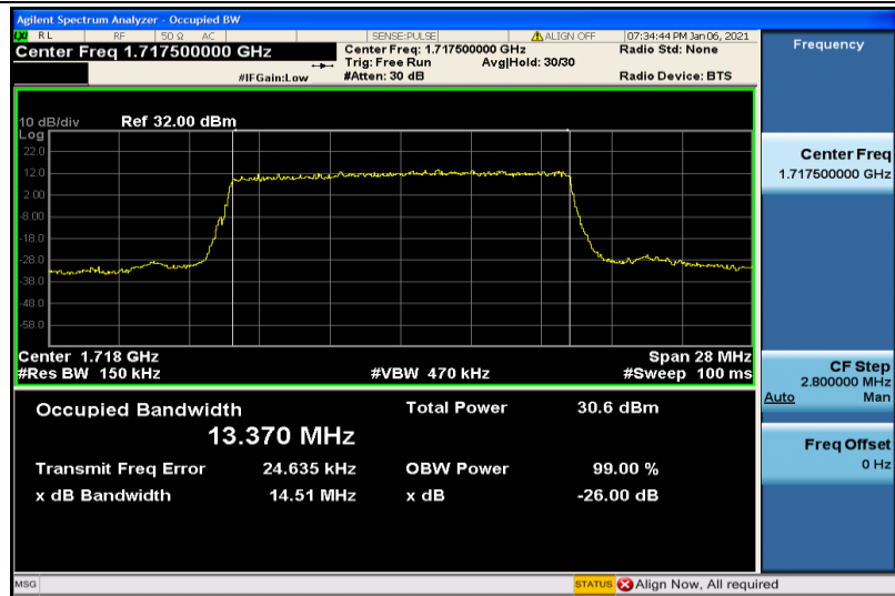
Band4-15MHz-QPSK-20025-75RB#0-13.370
