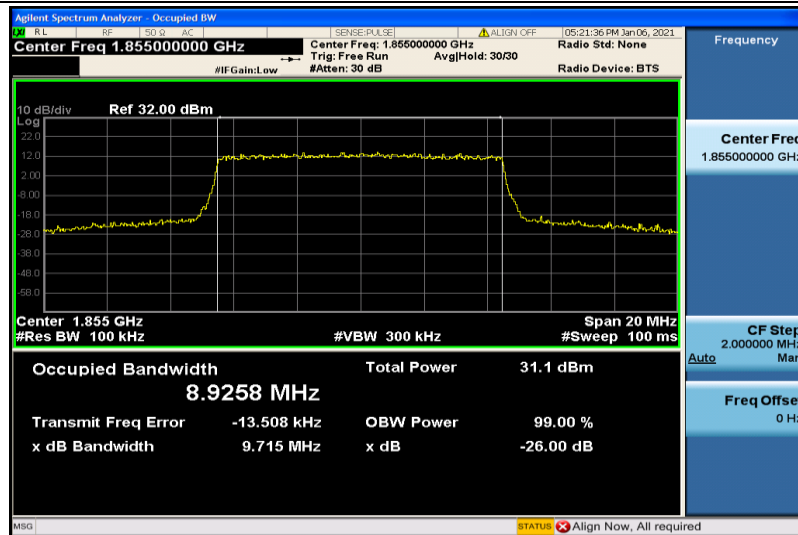
Band2-10MHz-16QAM-18650-50RB#0-8.9258
