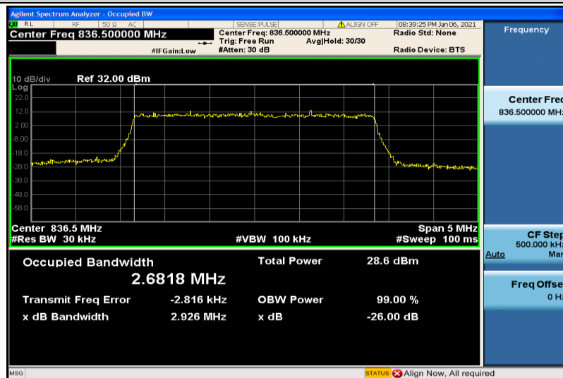
Band5-3MHz-16QAM-20525-15RB#0-2.6818
