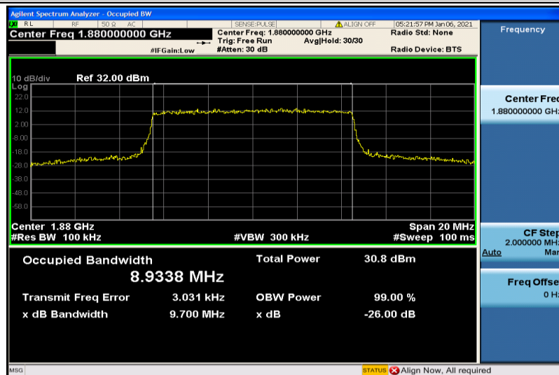
Band2-10MHz-16QAM-18900-50RB#0-8.9338
