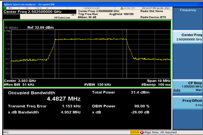
Band7-5MHz-QPSK-20775-25RB#0-4.4827
