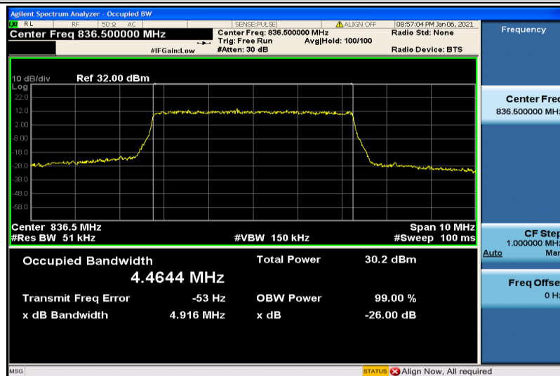
Band5-5MHz-QPSK-20525-25RB#0-4.4644
