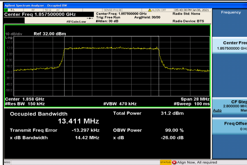
Band2-15MHz-16QAM-18675-75RB#0-13.411
