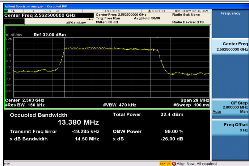
Band7-15MHz-QPSK-21375-75RB#0-13.380
