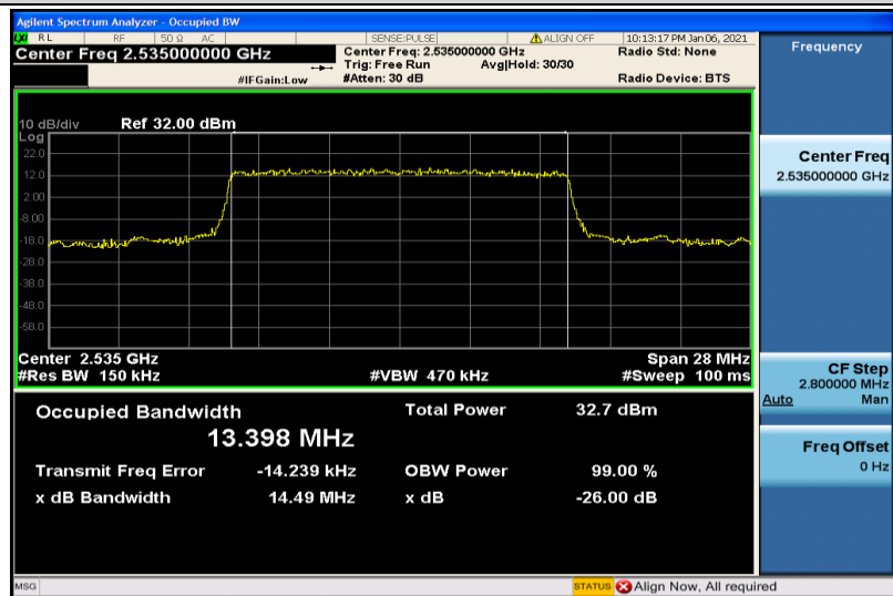
Band7-15MHz-QPSK-21100-75RB#0-13.398
