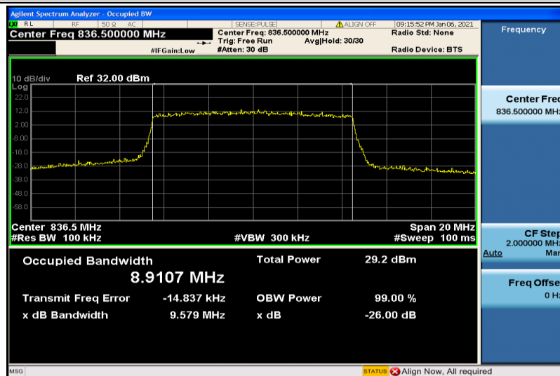
Band5-10MHz-16QAM-20525-50RB#0-8.9107
