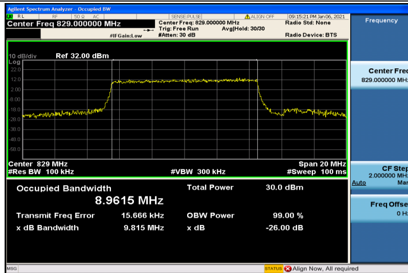
Band5-10MHz-QPSK-20450-50RB#0-8.9615
