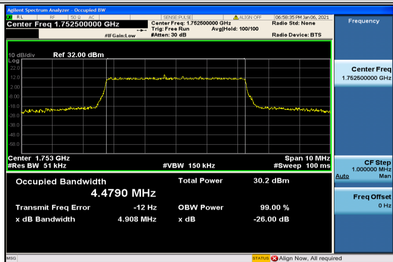
Band4-5MHz-16QAM-20375-25RB#0-4.4790
