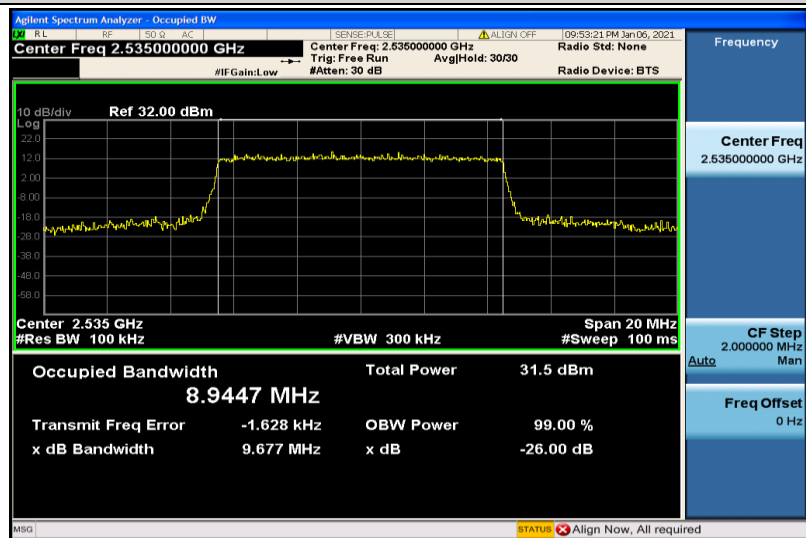
Band7-10MHz-16QAM-21100-50RB#0-8.9447
