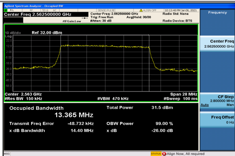
Band7-15MHz-16QAM-21375-75RB#0-13.365
