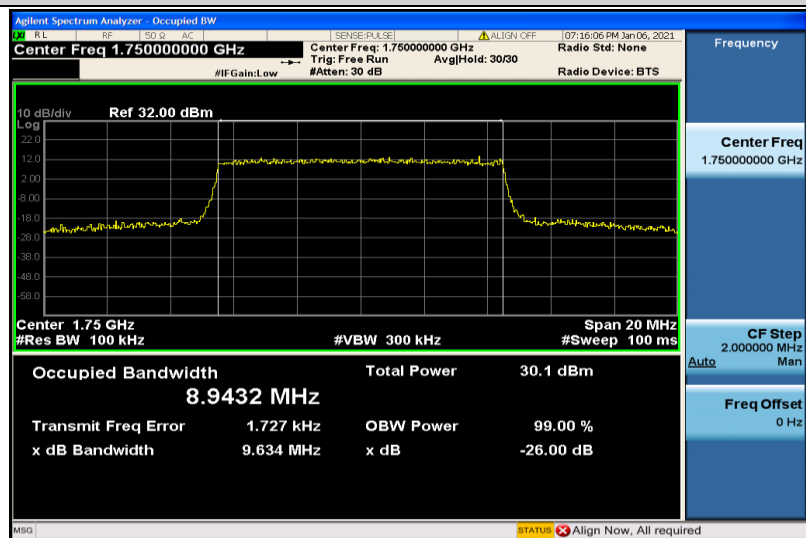
Band4-10MHz-16QAM-20350-50RB#0-8.9432
