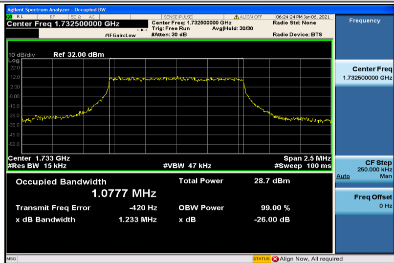
Band4-1.4MHz-16QAM-20175-6RB#0-1.0777
