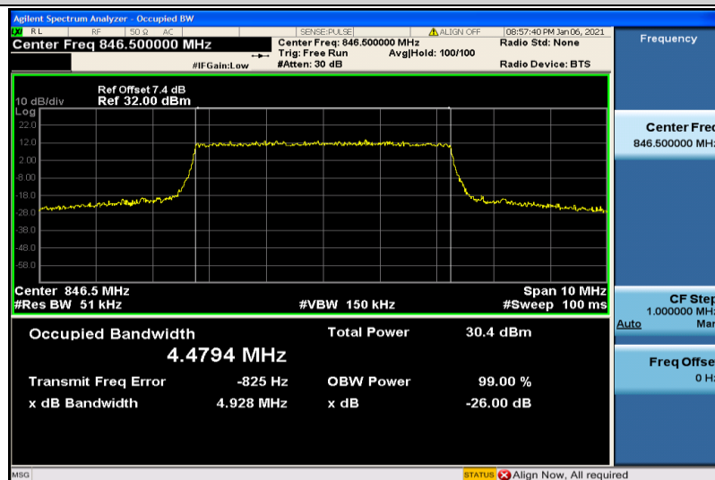
Band5-5MHz-QPSK-20625-25RB#0-4.4794
