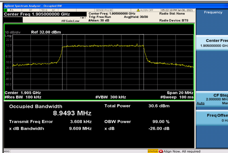
Band2-10MHz-16QAM-19150-50RB#0-8.9493
