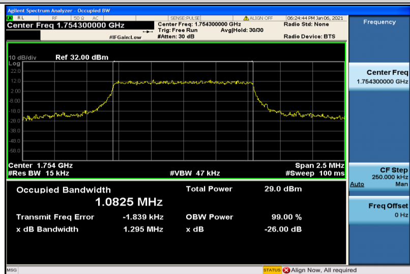
Band4-1.4MHz-16QAM-20393-6RB#0-1.0825
