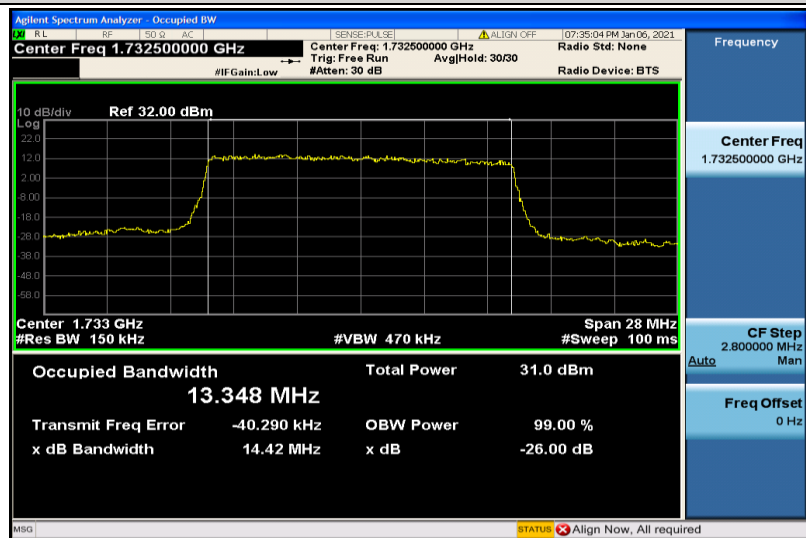
Band4-15MHz-QPSK-20175-75RB#0-13.348
