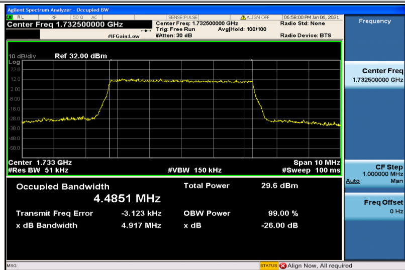
Band4-5MHz-16QAM-20175-25RB#0-4.4851
