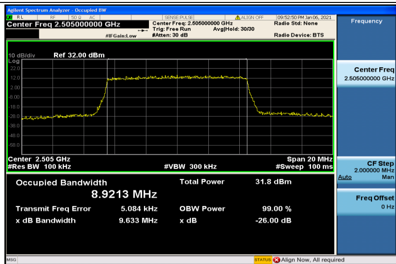
Band7-10MHz-QPSK-20800-50RB#0-8.9213
