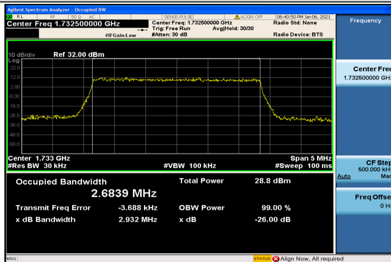
Band4-3MHz-16QAM-20175-15RB#0-2.6839
