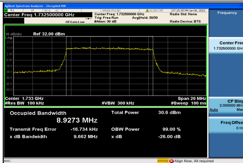
Band4-10MHz-QPSK-20175-50RB#0-8.9273
