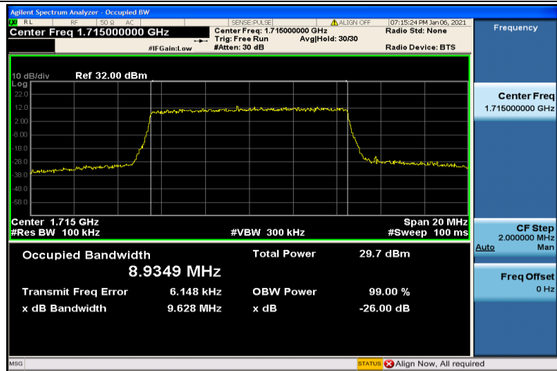
Band4-10MHz-16QAM-20000-50RB#0-8.9349
