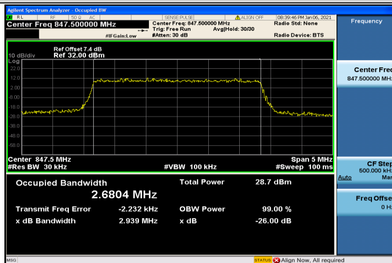
Band5-3MHz-16QAM-20635-15RB#0-2.6804
