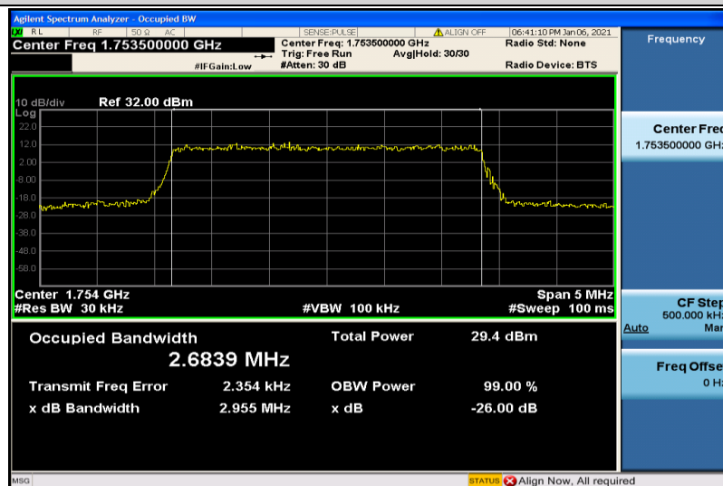
Band4-3MHz-16QAM-20385-15RB#0-2.6839
